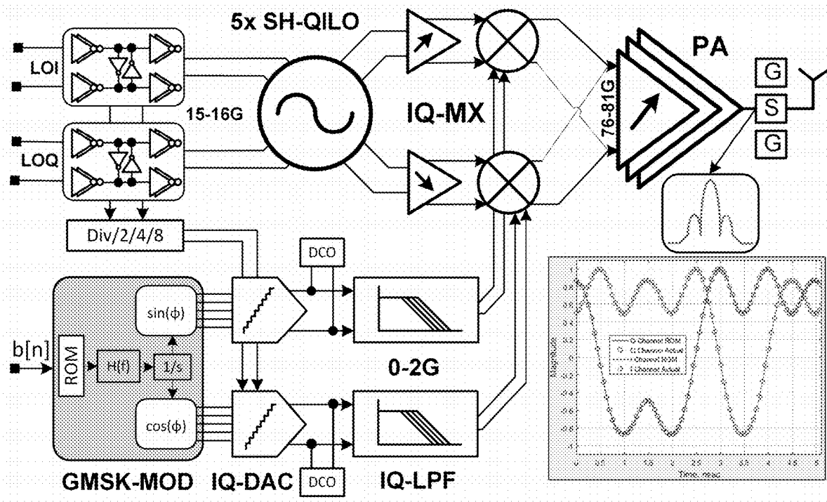
The quadrature GMSK transmitter architecture.
