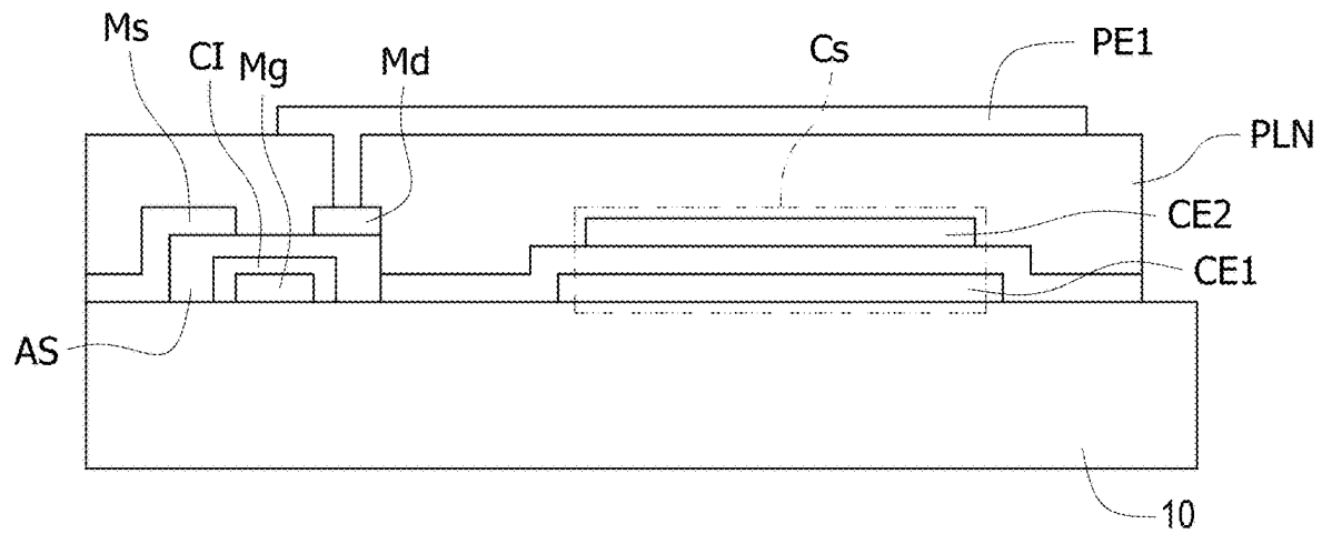
FIG.2C RELATED ART
