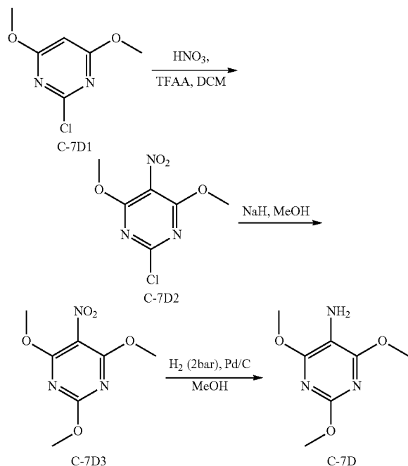
Reaction Scheme 5.
