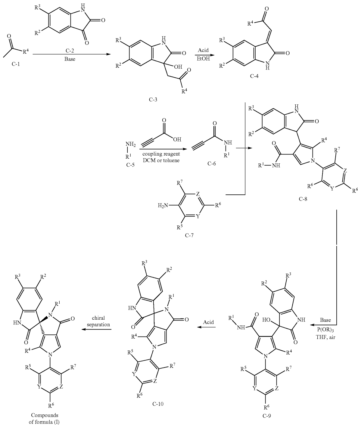
Reaction Scheme 1.
