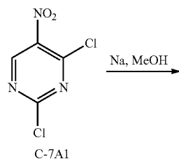
Reaction Scheme 2.
