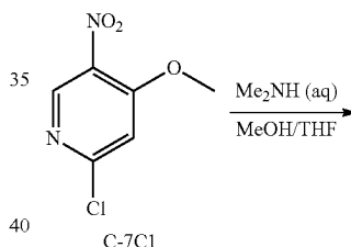
Reaction Scheme 4.
