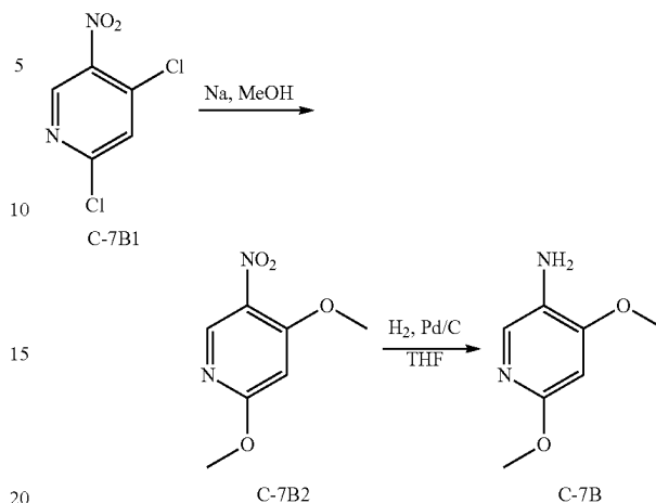
Reaction Scheme 3.
