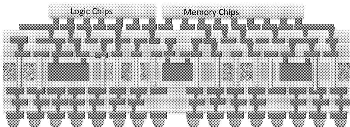
Chipset in multi-tile and multi-scale fan-out packages
