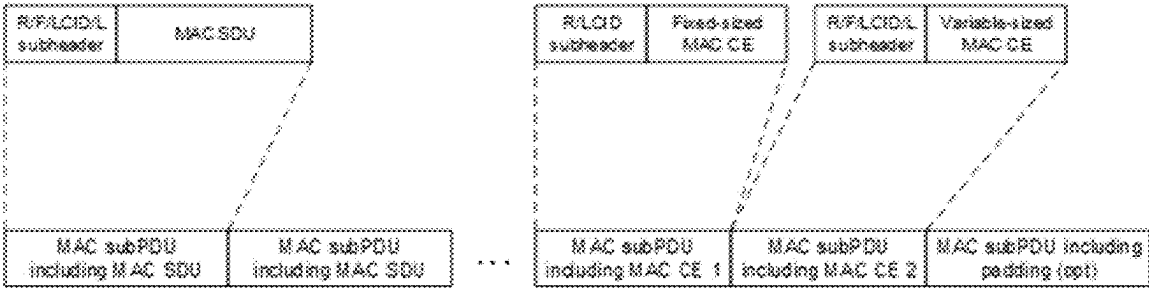
Example of a UL MAC PDU 3D20
