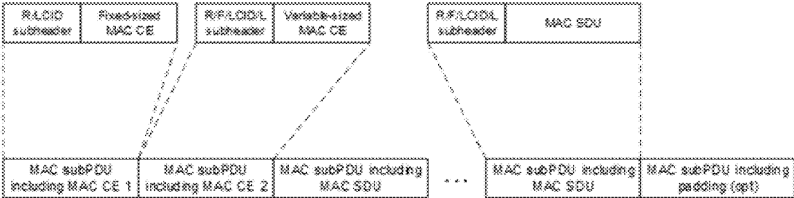
Example of a DL MAC PDU 3D10
