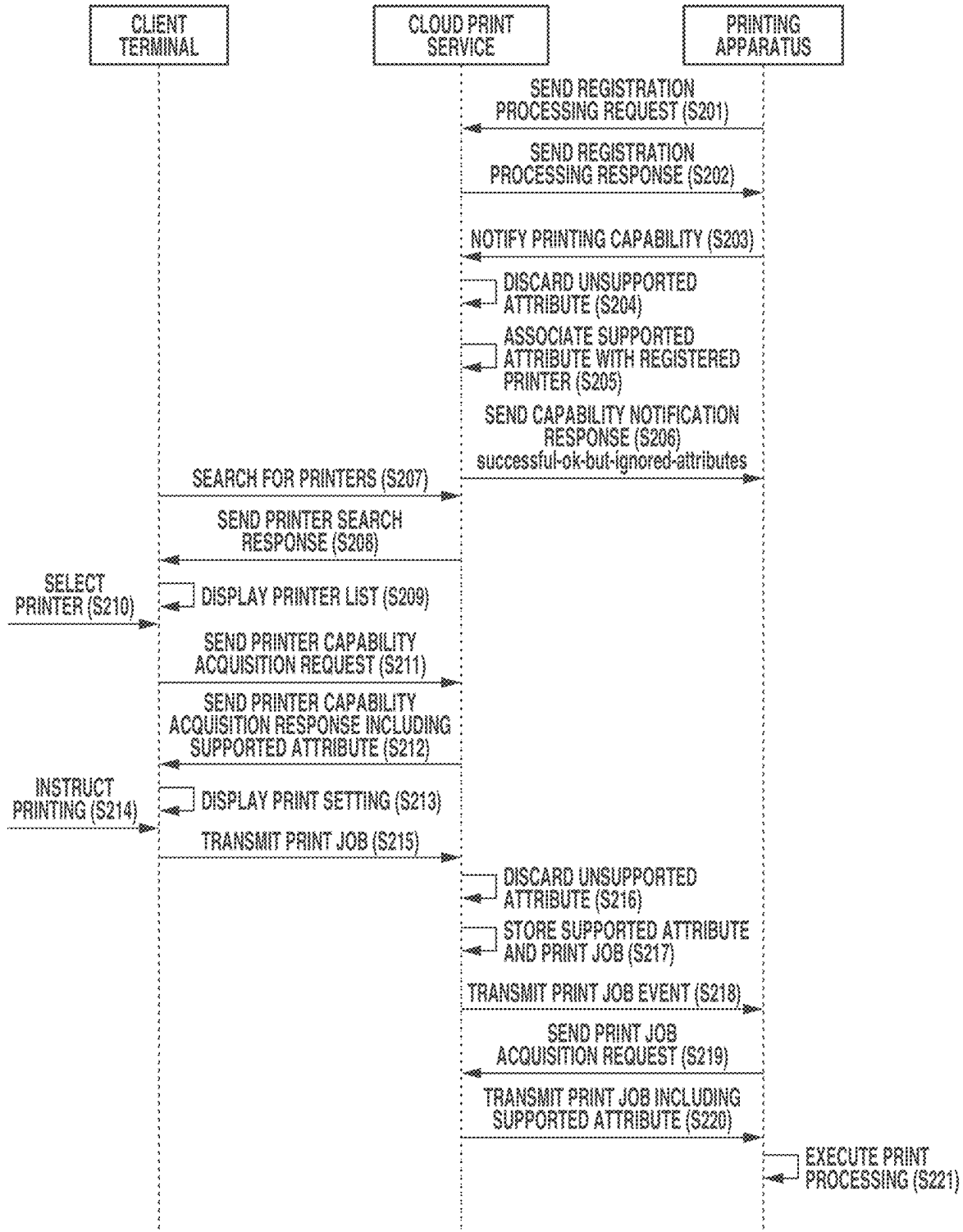
SEQUENCE DIAGRAM ILLUSTRATING CLOUD PRINT SERVICE OF RELATED ART
