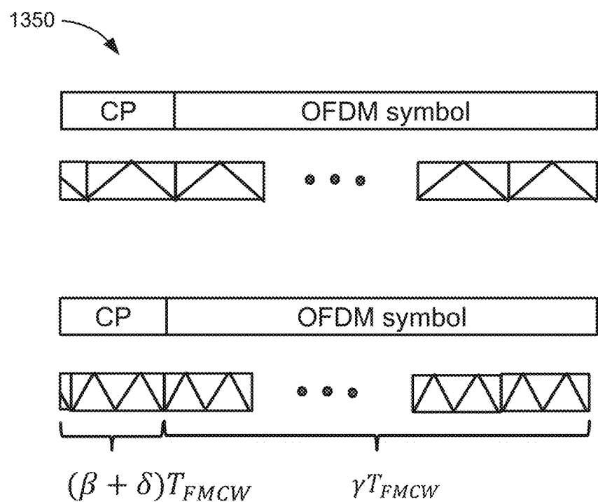
Piecewise linear chirp with CP structure
