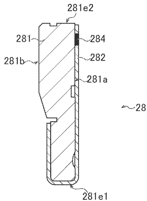
A-A CROSS SECTION
