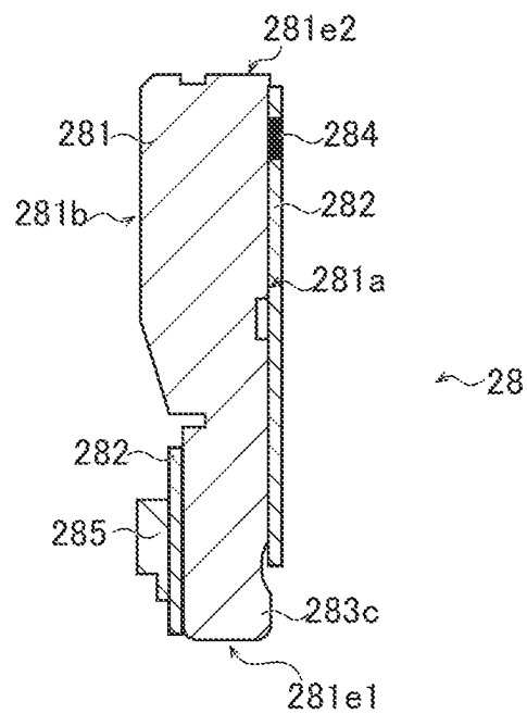
B-B CROSS SECTION
