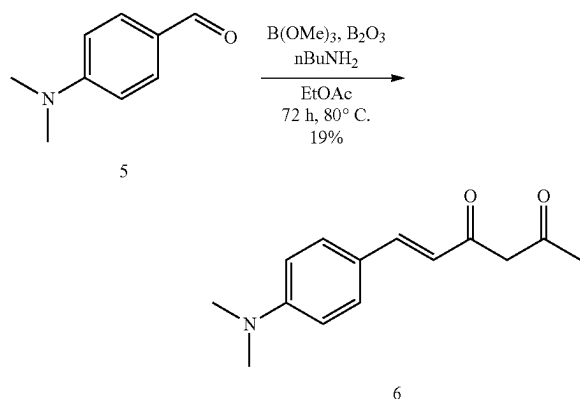
1-(4-(Dimethylamino)phenyl)-5-hydroxyhexa-1,4-dien-3-one (6)
