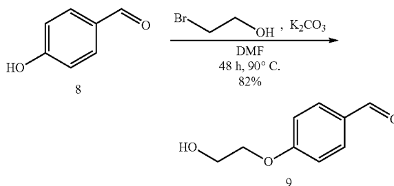
4-(2-Hydroxyethoxy) benzaldehyde (9)
