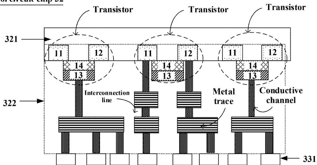
Control circuit chip 32
