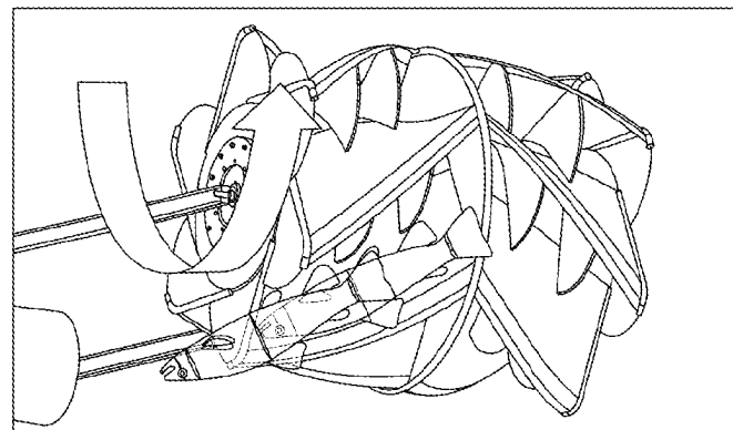
24" Salmonid Relative to Turbine
