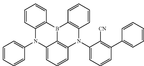
[Compound Group 1]
