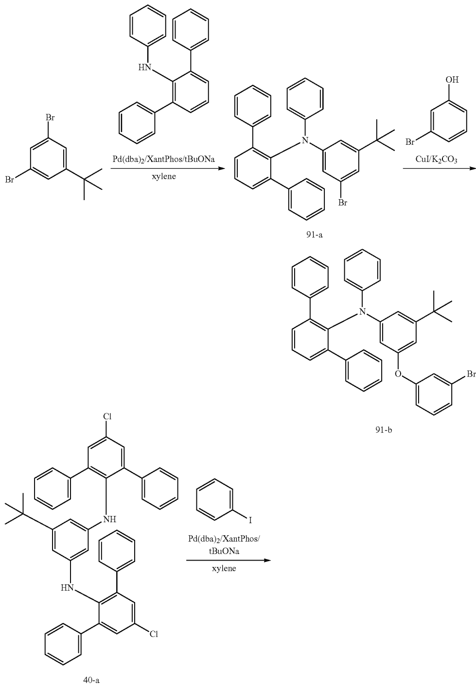
[Reaction Scheme 7]
