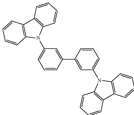
mCBP
