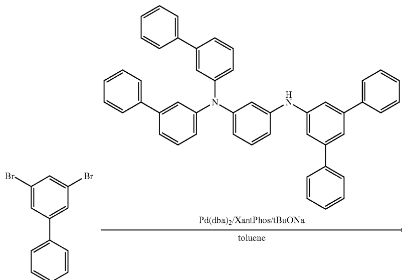
[Reaction Scheme 5]
