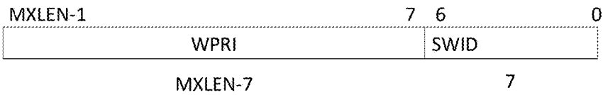
Custom Machine Address Translation and Protection CSR (matp)
