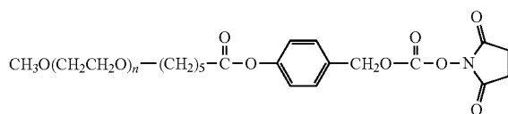
Formula XVI
