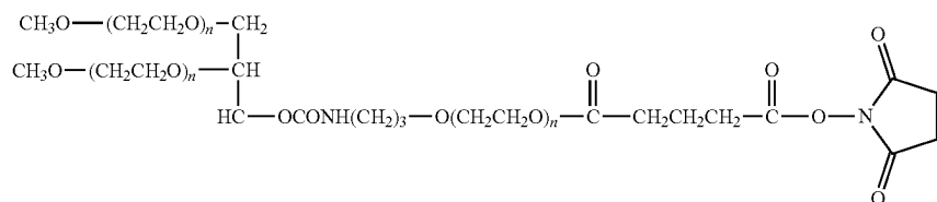
Formula XIII
