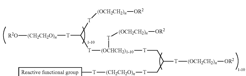
Formula H
