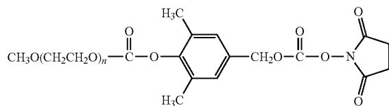
Formula XVI
