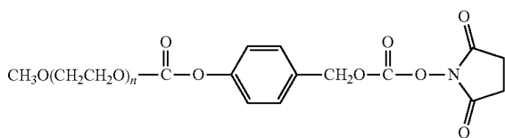
Formula XIV
