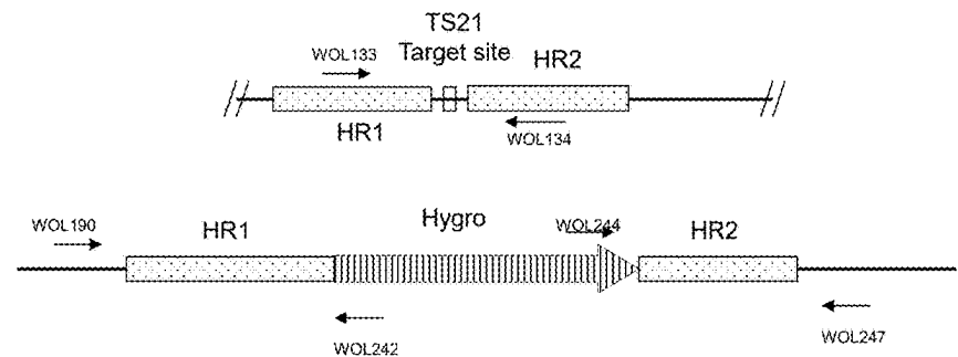
FIG. 3A: Genomic PCR assay to identify target site modification or transgene integration
