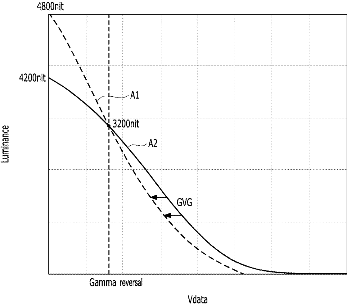
LUMINANCE CHARACTERISTICS OF A1 AND A2 ACCORDING TO Vdata
