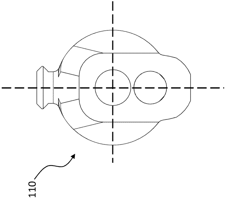
Firearm Adapter Proximal View
