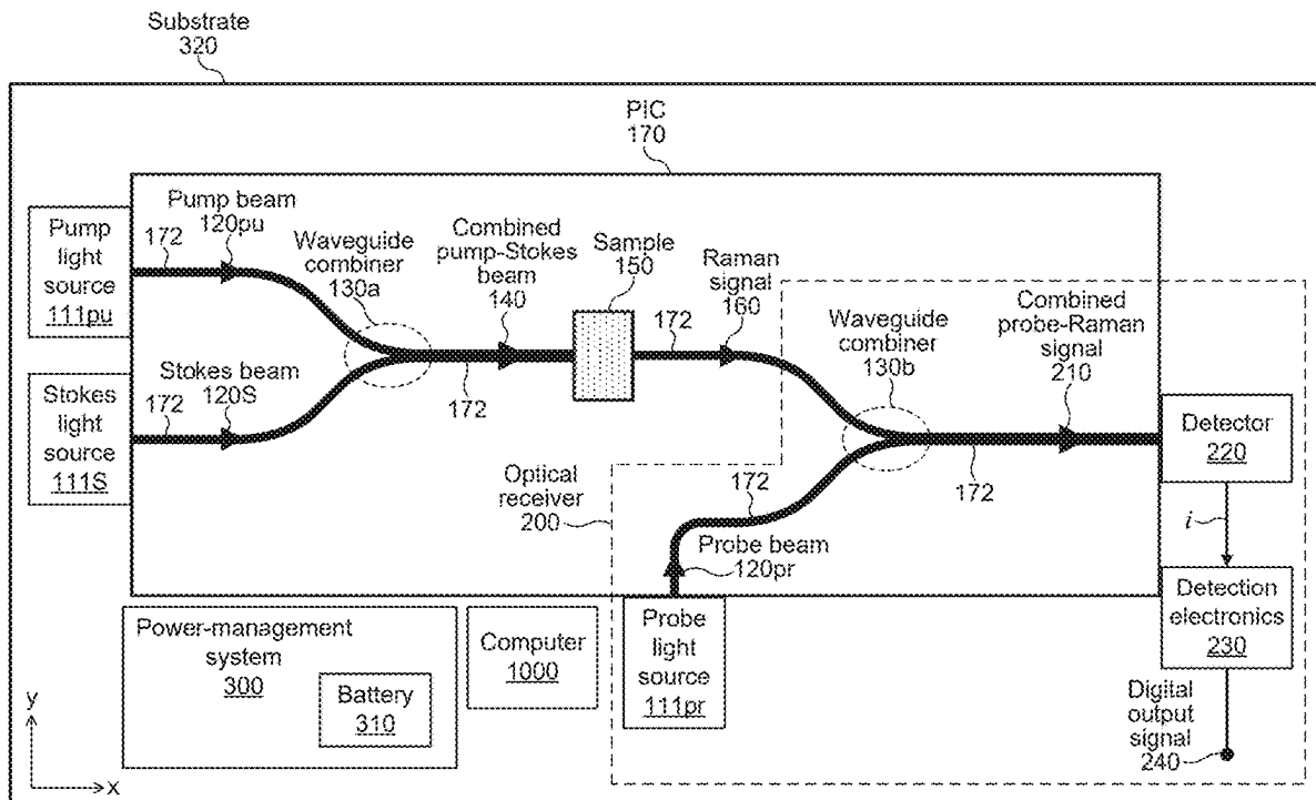
Raman spectroscopy system
