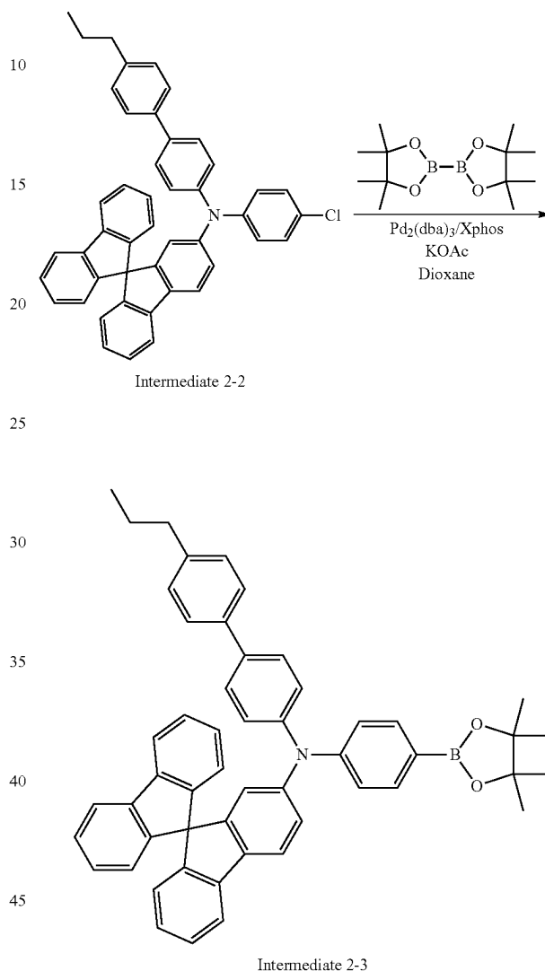
[Reaction Scheme 2-3]
