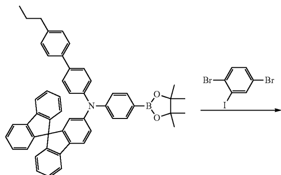
Intermediate 2-3
