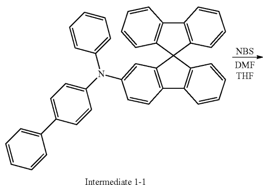
[Reaction Scheme 1-2]
