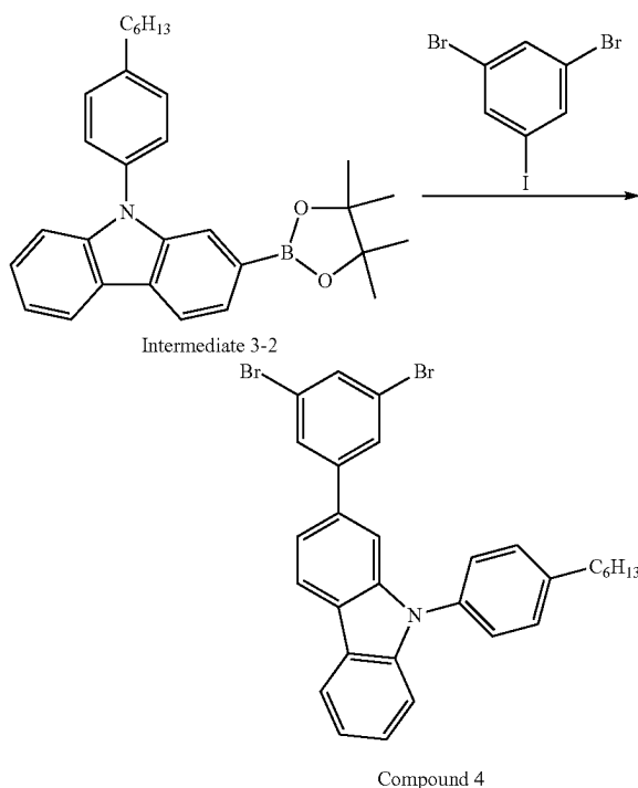
[Reaction Scheme 4-1]
