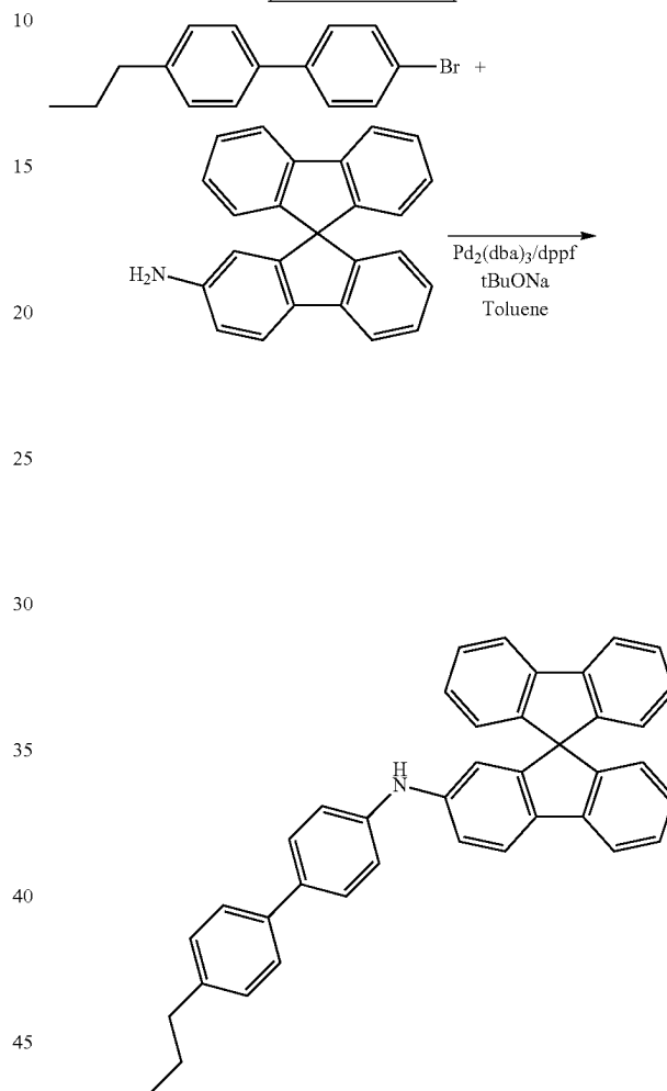
Intermediate 2-1
