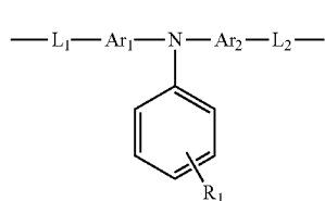
[Chemical Formula 1-1]
