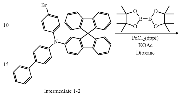
[Reaction Scheme 1-3]
