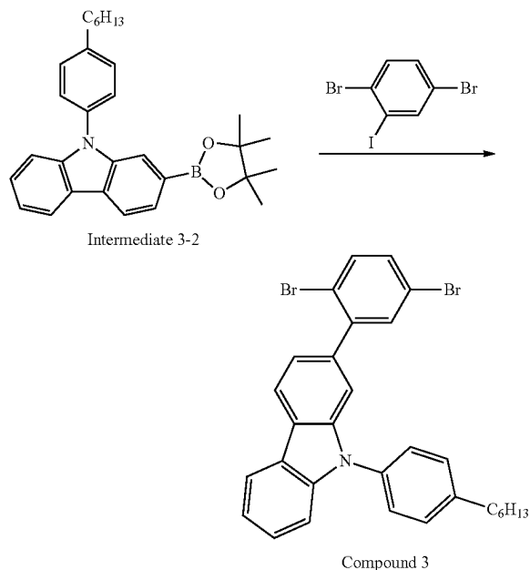
[Reaction Scheme 3-2]
