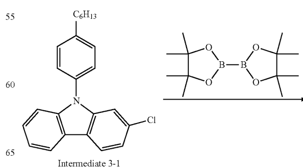
[Reaction Scheme 3-2]
