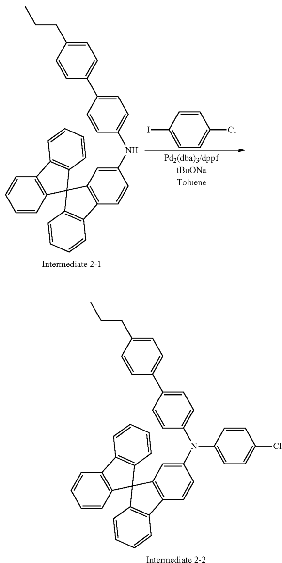
[Reaction Scheme 2-2]
