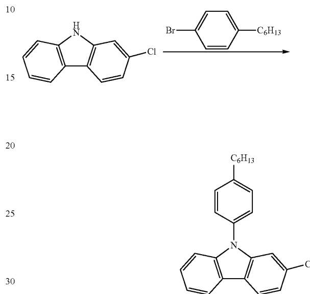
Intermediate 3-1
