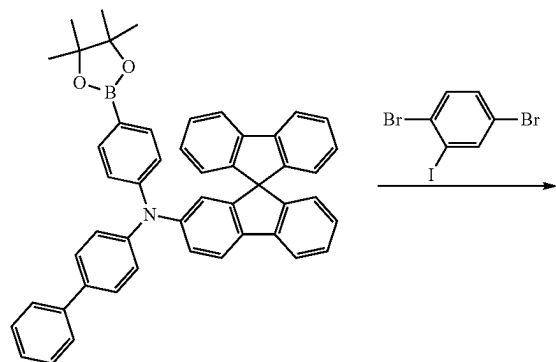
Intermediate 1-3
