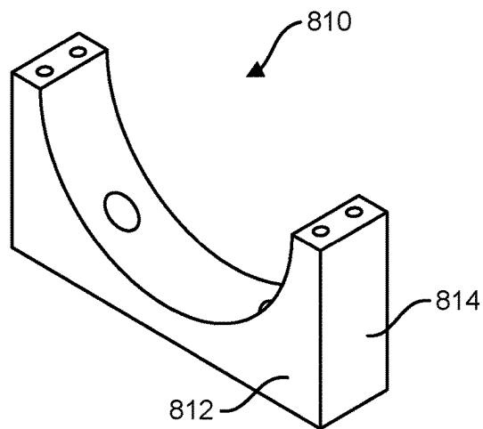
ISO VIEW
