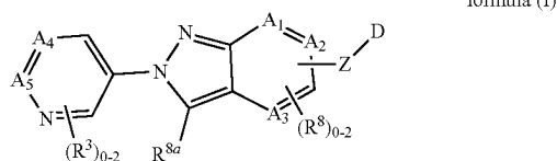
formula (I)
