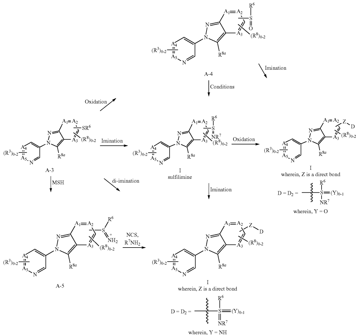
Scheme 6
