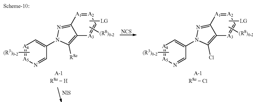
Scheme 10
