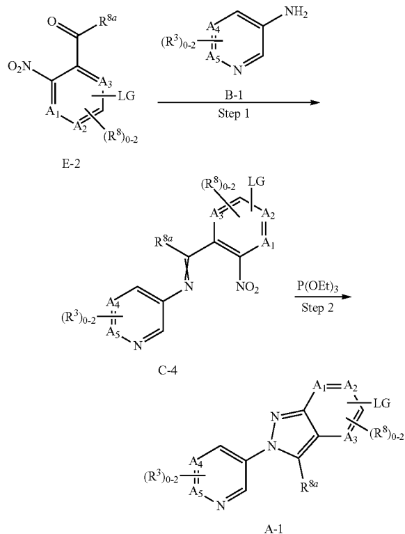
Scheme 14
