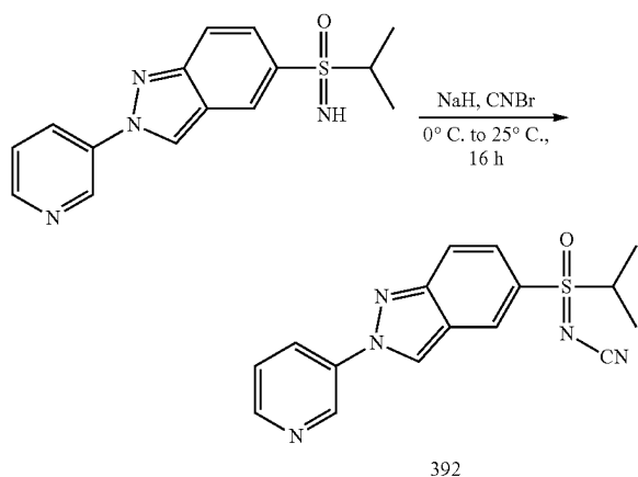
Example 14: Synthesis of N-(isopropyl(oxo)(2-(pyridin-3-yl)-2H-indazol-5-yl)- \lambda^6 -sulfaneylidene) cyanamide 392
