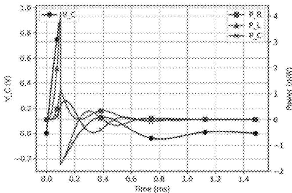
(c) RLC in series under-damping
