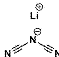
Lithium Dicyanamide
