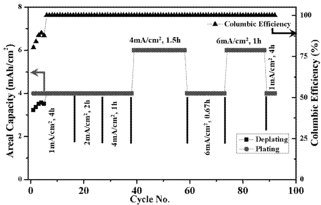
a) Coulombic Efficiency vs Current/Charge Density
