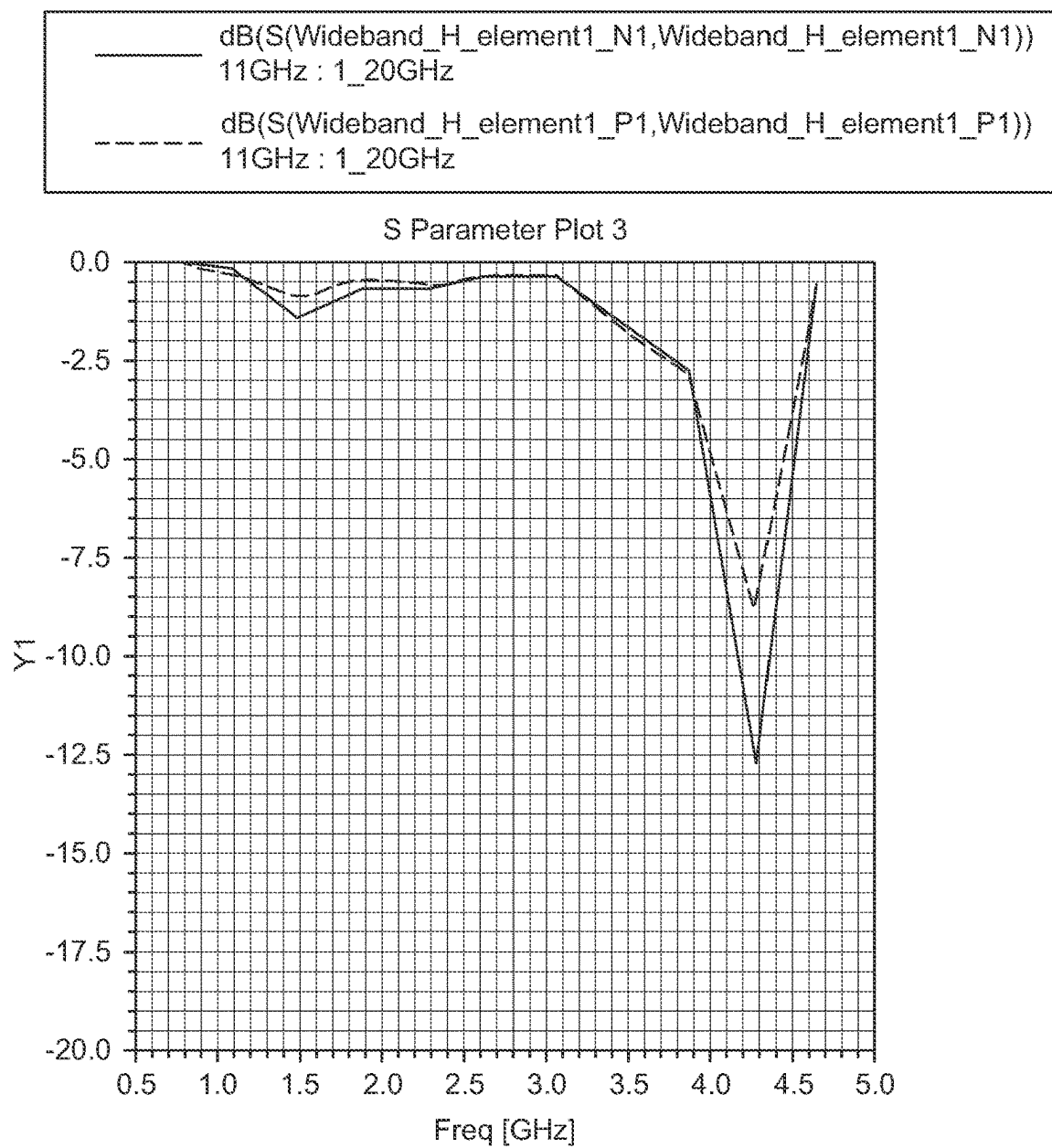
FIG. 16B (PRIOR ART)
