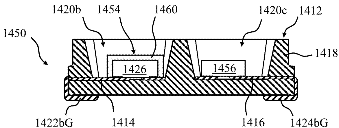
SECTION B-B
