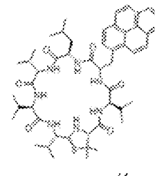
Chemical sum formula: C_{14}H_{18}N_2O_2S Exact molecular weight: 311.1303
