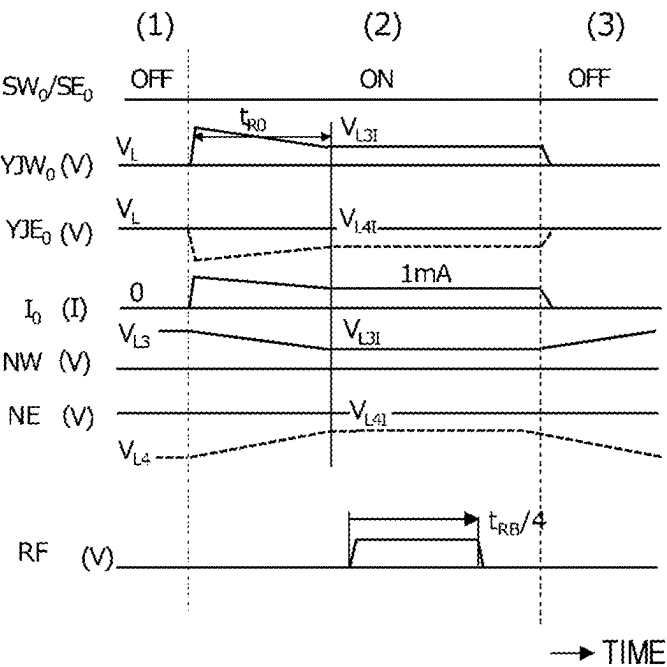
(b) OPERATION WAVEFORM OF Qubit ARRAY
