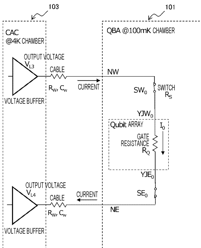
(a) CURRENT SUPPLY PATH TO QBA
