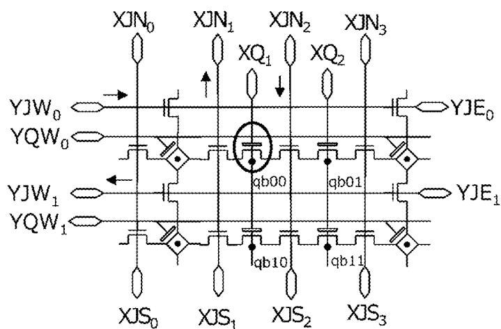
(a) ARRAY CIRCUIT DIAGRAM
