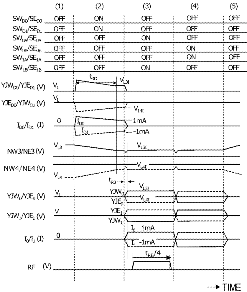
(b) OPERATION WAVEFORM OF Qubit ARRAY
