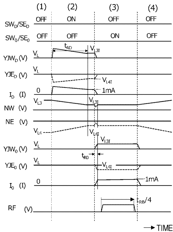
(b) OPERATION WAVEFORM OF Qubit ARRAY
