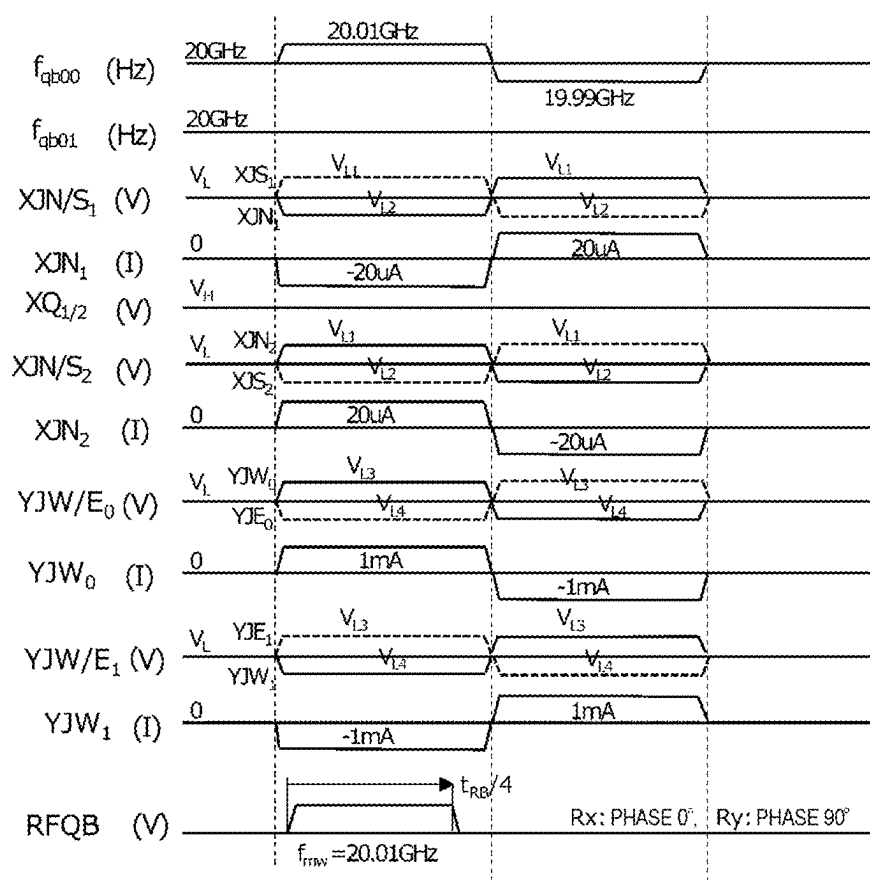
(b) OPERATION WAVEFORM
