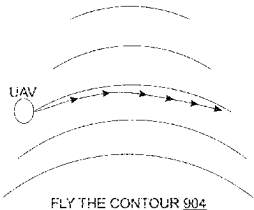
GRADIENT-BASED NAVIGATION
