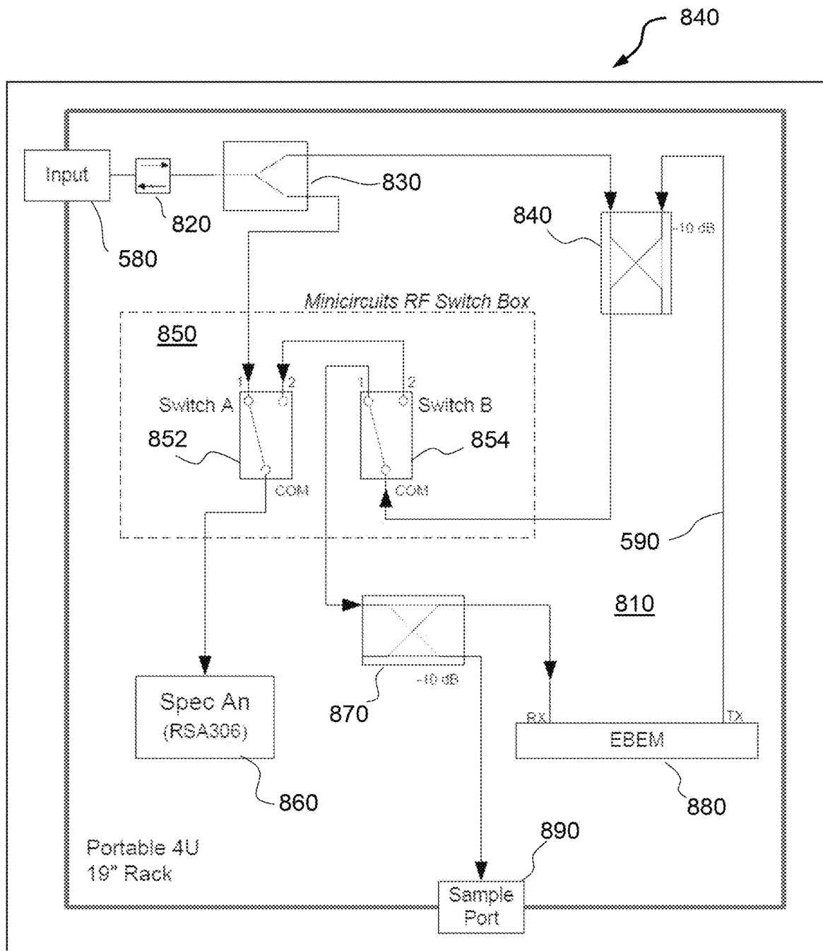
Unmanned BERT RF Hardware Diagram
