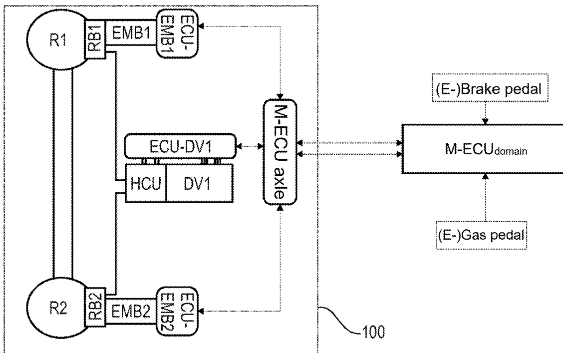
Axle module with EHB+EMB
