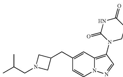
1-(5-((1-isobutylazetidin-3-yl)methyl)pyrazolo[1,5-a]pyridin-3-yl)dihydropyrimidine-2,4(1H,3H)-dione
