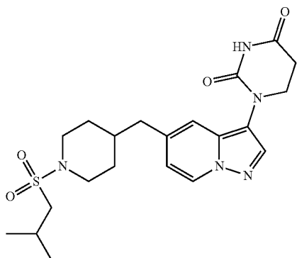
1-(5-((1-(isobutylsulfonyl)piperidin-4-yl)methyl)pyrazolo[1,5-a]pyridin-3-yl) dihydropyrimidine-2,4(1H,3H)-dione
