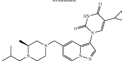
(S)-5-cyclopropyl-1-(5-((4-isobutyl-3-methylpiperazin-1-yl)methyl)pyrazolo[1,5-a]pyridin-3-yl)pyrimidine-2,4(1H,3H)-dione
