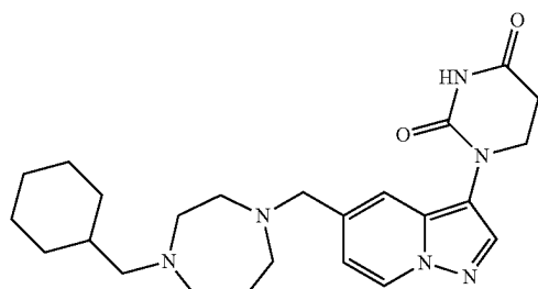
1-(5-((4-(cyclohexylmethyl)-1,4-diazepan-1-yl)methyl)pyrazolo[1,5-a]pyridin-3-yl)dihydropyrimidine-2,4(1H,3H)-dione
