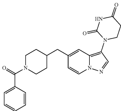
1-(5-((1-benzoylpiperidin-4-yl)methyl)pyrazolo[1,5-a]pyridin-3-yl)dihydropyrimidine-2,4(1H,3H)-dione
