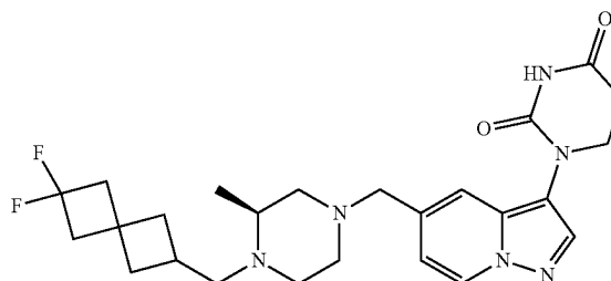
(S)-1-(5-(((4-((6,6-difluorospiro[3.3]heptan-2-yl)methyl)-3-methylpiperazin-1-yl)methyl)pyrazolo[1,5-a]pyridin-3-yl)dihydropyrimidine-2,4(1H,3H)-dione
