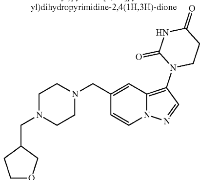
1-(5-((4-((tetrahydrofuran-3-yl)methyl)piperazin-1-yl)methyl)pyrazolo[1,5-a]pyridin-3-yl)dihydropyrimidine-2,4(1H,3H)-dione
