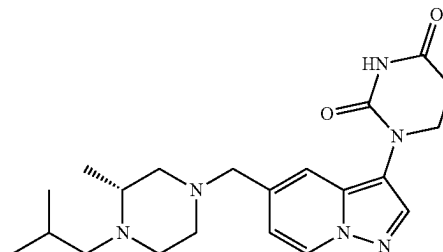
(R)-1-(5-((4-isobutyl-3-methylpiperazin-1-yl)methyl)pyrazolo[1,5-a]pyridin-3-yl)dihydropyrimidine-2,4(1H,3H)-dione
