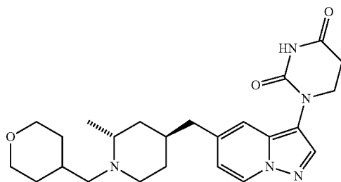
1-(5-(((2R,4S)-2-methyl-1-((tetrahydro-2H-pyran-4-yl)methyl)piperidin-4-yl)methyl)pyrazolo[1,5-a]pyridin-3-yl) dihydropyrimidine-2,4(1H,3H)-dione
