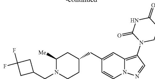
1-(5-(((2S,4R)-1-((3,3-difluorocyclobutyl)methyl)-2-methylpiperidin-4-yl)methyl)pyrazolo[1,5-a]pyridin-3-yl)dihydropyrimidine-2,4(1H,3H)-dione
