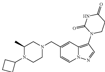
(S)-1-(5-((4-cyclobutyl-3-methylpiperazin-1-yl)methyl)pyrazolo[1,5-a]pyridin-3-yl)dihydropyrimidine-2,4(1H,3H)-dione
