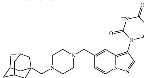
1-(5-((4-(((3r,5r,7r)-adamantan-1-yl)methyl)piperazin-1-yl)methyl)pyrazolo[1,5-a]pyridin-3-yl)dihydropyrimidine-2,4(1H,3H)-dione
