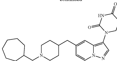
1-(5-((1-(cycloheptylmethyl)piperidin-4-yl)methyl)pyrazolo[1,5-a]pyridin-3-yl)dihydropyrimidine-2,4(1H,3H)-dione
