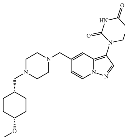
1-(5-((4-(((1s,4s)-4-methoxycyclohexyl)methyl)piperazin-1-yl)methyl)pyrazolo[1,5-a]pyridin-3-yl) dihydropyrimidine-2,4(1H,3H)-dione
