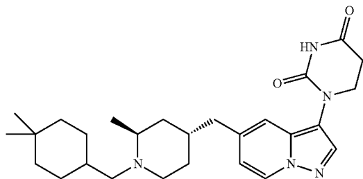
1-(5-(((2S,4R)-1-((4,4-dimethylcyclohexyl)methyl)-2-methylpiperidin-4-yl)methyl)pyrazolo[1,5-a]pyridin-3-yl)dihydropyrimidine-2,4(1H,3H)-dione
