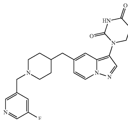
1-(5-((1-((5-fluoropyridin-3-yl)methyl)piperidin-4-yl)methyl)pyrazolo[1,5-a]pyridin-3-yl)dihydropyrimidine-2,4(1H,3H)-dione
