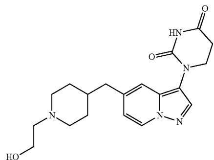
1-(5-((1-(2-hydroxyethyl)piperidin-4-yl)methyl)pyrazolo[1,5-a]pyridin-3-yl)dihydropyrimidine-2,4(1H,3H)-dione
