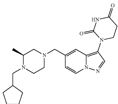
(S)-1-((5-((4-(cyclopentylmethyl)-3-methylpiperazin-1-yl)methyl)pyrazolo[1,5-a]pyridin-3-yl)dihydropyrimidine-2,4(1H,3H)-dione
