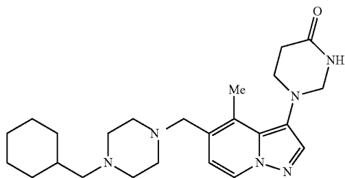
1-(5-((1-(cyclohexylmethyl)piperidin-4-yl)methyl)-4-methylpyrazolo[1,5-a]pyridin-3-yl)dihydropyrimidine-2,4(1H,3H)-dione
