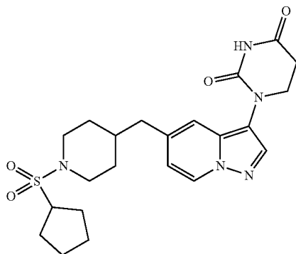
1-(5-((1-(cyclopentylsulfonyl)piperidin-4-yl)methyl)pyrazolo[1,5-a]pyridin-3-yl) dihydropyrimidine-2,4(1H,3H)-dione
