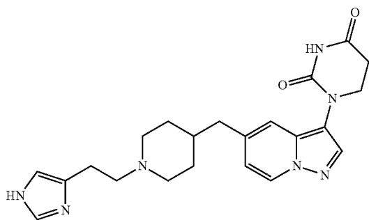
1-(5-((1-(2-(1H-imidazol-4-yl)ethyl)piperidin-4-yl)methyl)pyrazolo[1,5-a]pyridin-3-yl) dihydropyrimidine-2,4(1H,3H)-dione
