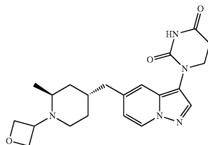
1-(5-(((2S,4R)-2-methyl-1-(oxetan-3-yl)piperidin-4-yl) methyl)pyrazolo[1,5-a]pyridin-3-yl) dihydropyrimidine- 2,4(1H,3H)-dione
