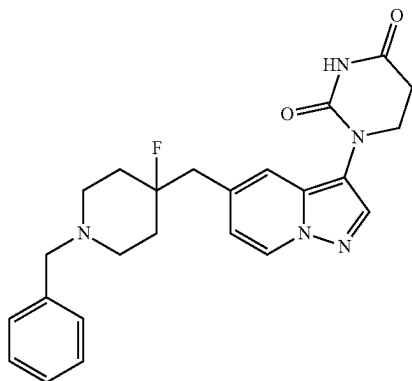
1-(5-((1-benzyl-4-fluoropiperidin-4-yl)methyl)pyrazolo[1,5-a]pyridin-3-yl)dihydropyrimidine-2,4(1H,3H)-dione
