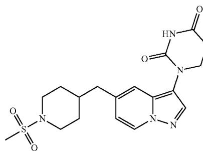
1-(5-((1-(methylsulfonyl)piperidin-4-yl)methyl)pyrazolo[1,5-a]pyridin-3-yl)dihydropyrimidine-2,4(1H,3H)-dione
