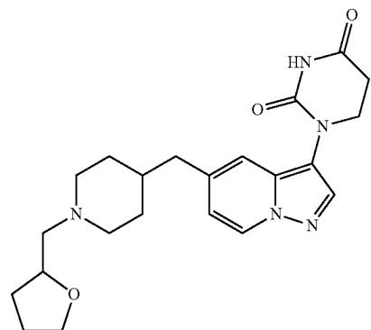
1-(5-((1-((tetrahydrofuran-2-yl)methyl)piperidin-4-yl)methyl)pyrazolo[1,5-a]pyridin-3-yl) dihydropyrimidine-2,4(1H,3H)-dione
