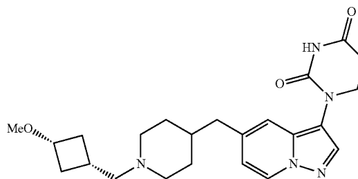
1-(5-((1-(((1S,3S)-3-methoxycyclobutyl)methyl)piperidin-4-yl)methyl)pyrazolo[1,5-a]pyridin-3-yl)dihydropyrimidine-2,4(1H,3H)-dione
