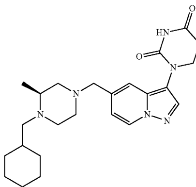
(S)-1-(5-((4-(cyclohexylmethyl)-3-methylpiperazin-1-yl)methyl)pyrazolo[1,5-a]pyridin-3-yl)dihydropyrimidine-2,4(1H,3H)-dione
