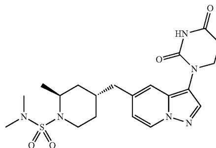
(2S,4R)-4-((3-(2,4-dioxotetrahydropyrimidin-1(2H)-yl)pyrazolo[1,5-a]pyridin-5-yl)methyl)-N,N,2-trimethylpiperidine-2-sulfonamide
