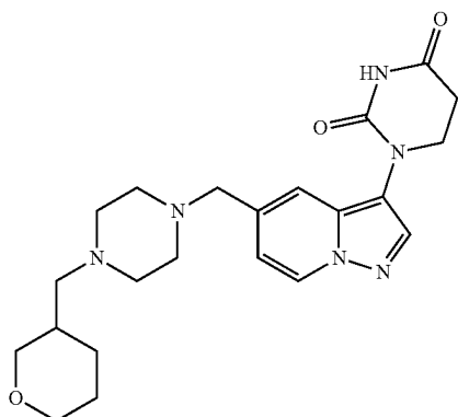
1-(5-((4-((tetrahydro-2H-pyran-3-yl)methyl)piperazin-1-yl)methyl)pyrazolo[1,5-a]pyridin-3-yl)dihydropyrimidine-2,4(1H,3H)-dione
