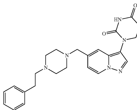
1-(5-((4-phenethylpiperazin-1-yl)methyl)pyrazolo[1,5-a]pyridin-3-yl)dihydropyrimidine-2,4(1H,3H)-dione
