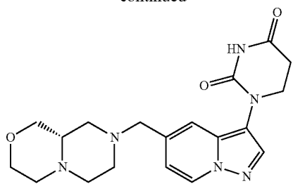
(S)-1-(5-((hexahydropyrazino[2,1-c][1,4]oxazin-8(1H)-yl)methyl)pyrazolo[1,5-a]pyridin-3-yl) dihydropyrimidine-2,4(1H,3H)-dione
