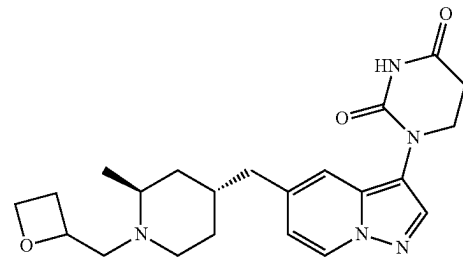
1-(5-(((2S,4R)-2-methyl-1-(oxetan-2-ylmethyl)piperidin- 4-yl)methyl)pyrazolo[1,5-a]pyridin-3-yl) dihydropyrimidine- 2,4(1H,3H)-dione
