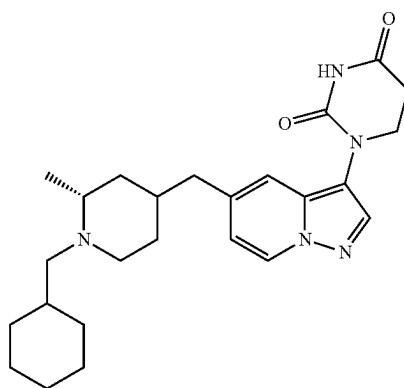
(R)-1-(5-((4-(cyclohexylmethyl)-3-methylpiperazin-1-yl)methyl)pyrazolo[1,5-a]pyridin-3-yl)dihydropyrimidine-2,4(1H,3H)-dione
