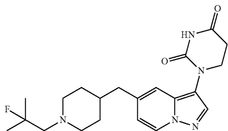
1-(5-((1-(2-fluoro-2-methylpropyl)piperidin-4-yl)methyl)pyrazolo[1,5-a]pyridin-3-yl) dihydropyrimidine-2,4(1H,3H)-dione
