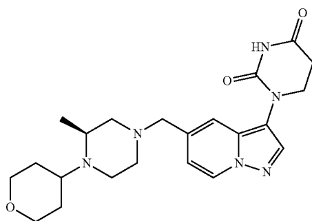
(S)-1-(5-((3-methyl-4-(tetrahydro-2H-pyran-4-yl)piperazin-1-yl)methyl)pyrazolo[1,5-a]pyridin-3-yl)dihydropyrimidine-2,4(1H,3H)-dione
