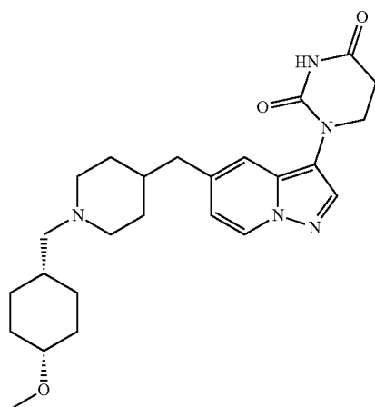
1-(5-(((1s,4s)-4-methoxycyclohexyl)methyl)piperidin-4-yl)methylpyrazolo[1,5-a]pyridin-3-yl)dihydropyrimidine-2,4(1H,3H)-dione
