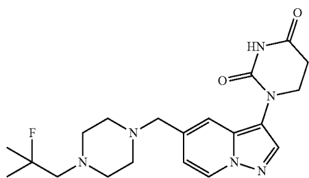
1-(5-((4-(2-fluoro-2-methylpropyl)piperazin-1-yl)methyl)pyrazolo[1,5-a]pyridin-3-yl)dihydropyrimidine-2,4(1H,3H)-dione
