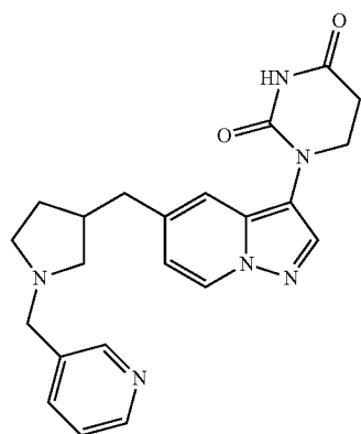
1-(5-((1-(pyridin-3-ylmethyl)pyrrolidin-3-yl)methyl)pyrazolo[1,5-a]pyridin-3-yl) dihydropyrimidine-2,4(1H,3H)-dione
