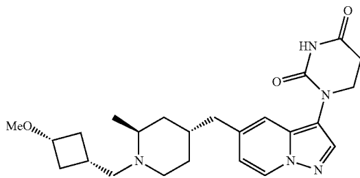
1-(5-(((2S,4R)-1-(((1S,3R)-3-methoxycyclobutyl)methyl)-2-methylpiperidin-4-yl)methyl)pyrazolo[1,5-a]pyridin-3-yl) dihydropyrimidine-2,4(1H,3H)-dione
