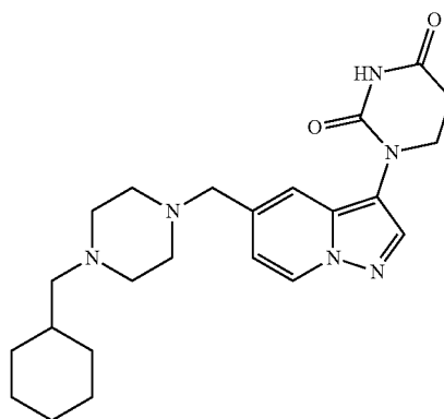
1-(5-((4-(cyclohexylmethyl)piperazin-1-yl)methyl)pyrazolo[1,5-a]pyridin-3-yl)dihydropyrimidine-2,4(1H,3H)-dione
