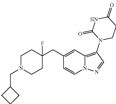
1-(5-((1-(1-cyclobutylmethyl)-4-fluoropiperidin-4-yl)methyl)pyrazolo[1,5-a]pyridin-3-yl)dihydropyrimidine-2,4(1H,3H)-dione
