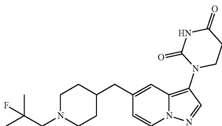
1-(5-((1-(2-fluoro-2-methylpropyl)piperidin-4-yl)methyl)pyrazolo[1,5-a]pyridin-3-yl)dihydropyrimidine-2,4(1H,3H)-dione
