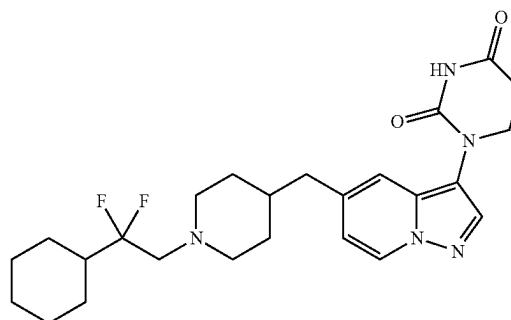
1-(5-((1-(2-cyclohexyl-2,2-difluoroethyl)piperidin-4-yl)methyl)pyrazolo[1,5-a]pyridin-3-yl) dihydropyrimidine-2,4(1H,3H)-dione
