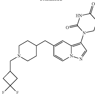
1-(5-((1-(3,3-difluorocyclobutyl)methyl)piperidin-4-yl)methyl)pyrazolo[1,5-a]pyridin-3-yl) dihydropyrimidine-2,4(1H,3H)-dione
