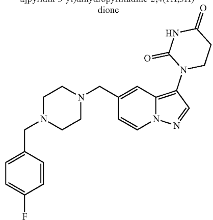
1-(5-((4-(4-fluorobenzyl)piperazin-1-yl)methyl)pyrazolo[1,5-a]pyridin-3-yl)dihydropyrimidine-2,4(1H,3H)-dione
