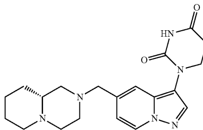
(R)-1-(5-((octahydro-2H-pyrido[1,2-a]pyrazin-2-yl)methyl)pyrazolo[1,5-a]pyridin-3-yl) dihydropyrimidine-2,4(1H,3H)-dione
