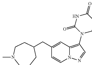
1-(5-((1-methylazepan-4-yl)methyl)pyrazolo[1,5-a]pyridin-3-yl)dihydropyrimidine-2,4-(1H,3H)-dione
