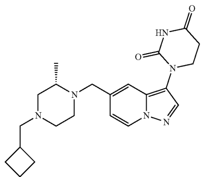
(S)-1-(5-((4-(cyclobutylmethyl)-2-methylpiperazin-1-yl)methyl)pyrazolo[1,5-a]pyridin-3-yl) dihydropyrimidine-2,4(1H,3H)-dione
