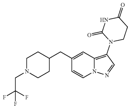
1-(5-((1-(2,2,2-trifluoroethyl)piperidin-4-yl)methyl)pyrazolo[1,5-a]pyridin-3-yl)dihydropyrimidine-2,4(1H,3H)-dione
