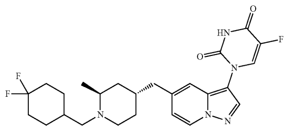
1-(5-(((2S,4R)-1-((4,4-difluorocyclohexyl)methyl)-2-methylpiperidin-4-yl)methyl)pyrazolo[1,5-a]pyridin-3-yl)-5-fluoropyrimidine-2,4(1H,3H)-dione
