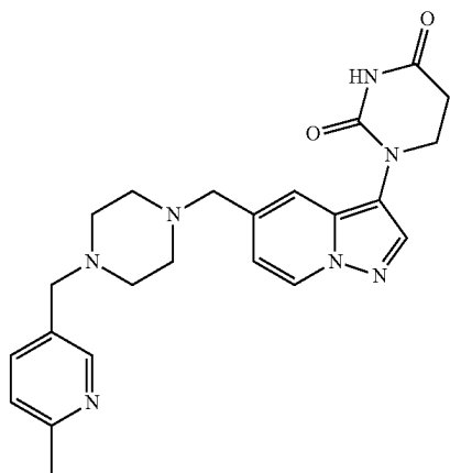
1-(5-((1-((6-methylpyridin-3-yl)methyl)piperidin-4-yl)methyl)pyrazolo[1,5-a]pyridin-3-yl) dihydropyrimidine-2,4(1H,3H)-dione
