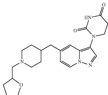
1-(5-((1-((tetrahydrofuran-2-yl)methyl)piperidin-4-yl)methyl)pyrazolo[1,5-
