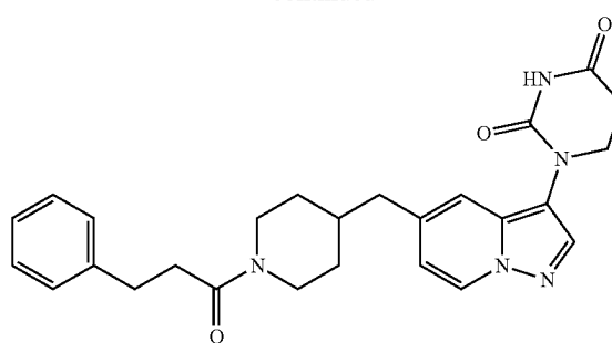
1-(5-((1-(3-phenylpropanoyl)piperidin-4-yl)methyl)pyrazolo[1,5-a]pyridin-3-yl) dihydropyrimidine-2,4(1H,3H)-dione
