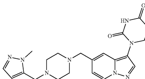
1-(5-((4-((1-methyl-1H-pyrazol-5-yl)methyl)piperazin-1-yl)methyl)pyrazolo[1,5-a]pyridin-3-yl)dihydropyrimidine-2,4(1H,3H)-dione
