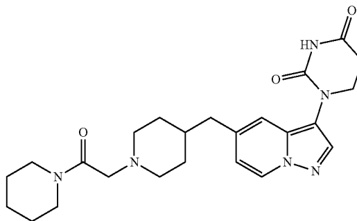
1-(5-((1-(2-oxo-2-(piperidin-1-yl)ethyl)piperidin-4-yl)methyl)pyrazolo[1,5-a]pyridin-3-yl)dihydropyrimidine-2,4(1H,3H)-dione
