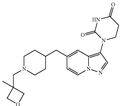
1-(5-((1-methyloxetan-3-yl)methyl)piperidin-4-yl)methylpyrazolo[1,5-a]pyridin-3-yl)dihydropyrimidine-2,4(1H,3H)-dione
