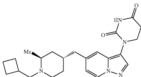
1-(5-(((2S,4R)-1-(cyclobutylmethyl)-2-methylpiperidin-4-yl)methyl)pyrazolo[1,5-a]pyridin-3-yl) dihydropyrimidine-2,4(1H,3H)-dione
