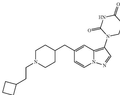
1-(5-((1-(2-cyclobutylethyl)piperidin-4-yl)methyl)pyrazolo[1,5-a]pyridin-3-yl)dihydropyrimidine-2,4(1H,3H)-dione
