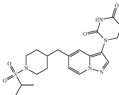
1-(5-((1-(isopropylsulfonyl)piperidin-4-yl)methyl)pyrazolo[1,5-a]pyridin-3-yl) dihydropyrimidine-2,4(1H,3H)-dione
