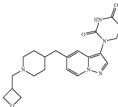
1-(5-((1-(oxetan-3-yl)methyl)piperidin-4-yl)methyl)pyrazolo[1,5-a]pyridin-3-yl) dihydropyrimidine-2,4(1H,3H)-dione
