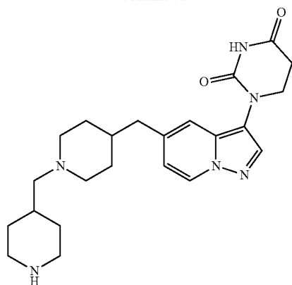
1-(5-((1-(piperidin-4-ylmethyl)piperidin-4-yl)methyl)pyrazolo[1,5-a]pyridin-3-yl)dihydropyrimidine-2,4(1H,3H)-dione
