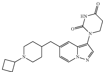
1-(5-((1-cyclobutylpiperidin-4-yl)methyl)pyrazolo[1,5-a]pyridin-3-yl) dihydropyrimidine-2,4(1H,3H)-dione
