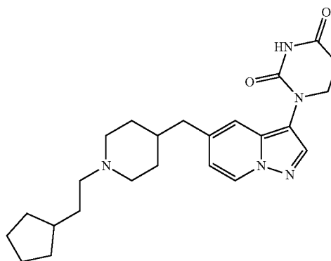
1-(5-((1-(2-cyclopentylethyl)piperidin-4-yl)methyl)pyrazolo[1,5-a]pyridin-3-yl)dihydropyrimidine-2,4(1H,3H)-dione
