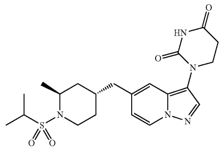
1-(5-(((2S,4R)-1-(isopropylsulfonyl)-2-methylpiperidin-4-yl)methyl)pyrazolo[1,5-a]pyridin-3-yl)dihydropyrimidine-2,4(1H,3H)-dione
