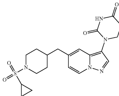
1-(5-((1-(cyclopropylsulfonyl)piperidin-4-yl)methyl)pyrazolo[1,5-a]pyridin-3-yl)dihydropyrimidine-2,4(1H,3H)-dione
