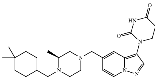
(S)-1-(5-(((4-((4,4-dimethylcyclohexyl)methyl)-3-methylpiperazin-1-yl)methyl)pyrazolo[1,5-a]pyridin-3-yl) dihydropyrimidine-2,4(1H,3H)-dione
