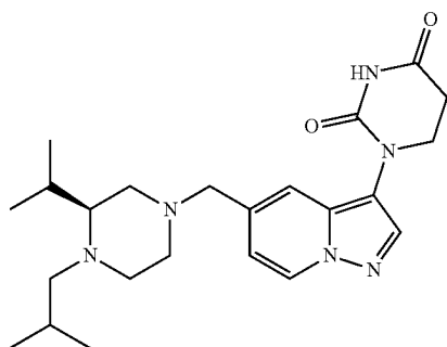
(S)-1-(5-((4-isobutyl-3-isopropylpiperazin-1-yl)methyl)pyrazolo[1,5-a]pyridin-3-yl)dihydropyrimidine-2,4(1H,3H)-dione
