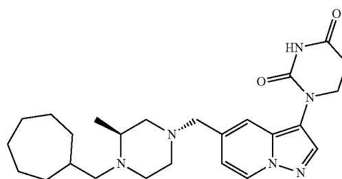
1-(5-(((2S,4R)-1-(cycloheptylmethyl)-2-methylpiperidin-4-yl)methyl)pyrazolo[1,5-a]pyridin-3-yl)dihydropyrimidine-2,4(1H,3H)-dione
