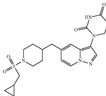
1-(5-((1-((cyclopropylmethyl)sulfonyl)piperidin-4-yl)methyl)pyrazolo[1,5-a]pyridin-3-yl)dihydropyrimidine-2,4(1H,3H)-dione
