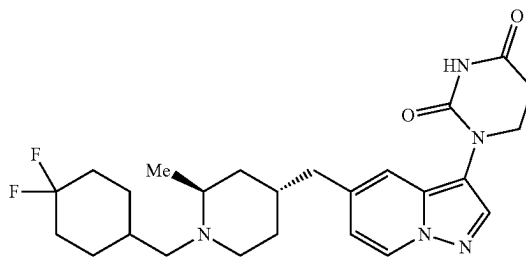
1-(5-(((2S,4R)-1-((4,4-difluorocyclohexyl)methyl)-2-methylpiperidin-4-yl)methyl)pyrazolo[1,5-a]pyridin-3-yl)dihydropyrimidine-2,4(1H,3H)-dione
