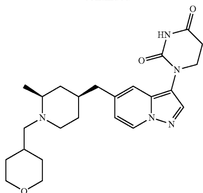
1-(5-(((2S,4S)-2-methyl-1-((tetrahydro-2H-pyran-4-yl)methyl)piperidin-4-yl)methyl)pyrazolo[1,5-a]pyridin-3-yl) dihydropyrimidine-2,4(1H,3H)-dione
