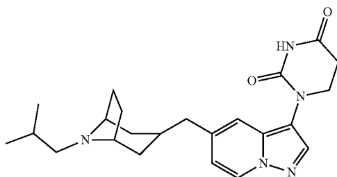
1-(5-(((1R,5S)-8-isobutyl-azabicyclo[3.2.1]octan-3-yl)methyl)pyrazolo[1,5-a]pyridin-3-yl) dihydropyrimidine-2,4(1H,3H)-dione
