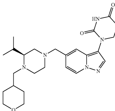
(S)-1-(5-((3-isopropyl-4-((tetrahydro-2H-pyran-4-yl)methyl)piperazin-1-yl)methyl)pyrazolo[1,5-a]pyridin-3-yl)dihydropyrimidine-2,4(1H,3H)-dione
