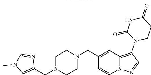
1-(5-((4-((1-methyl-1H-imidazol-4-yl)methyl)piperazin-1-yl)methyl)pyrazolo[1,5-a]pyridin-3-yl) dihydropyrimidine-2,4(1H,3H)-dione
