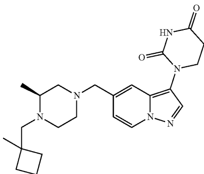
(S)-1-(5-(((3-methyl-4-((1-methylcyclobutyl)methyl)piperazin-1-yl)methyl)pyrazolo[1,5-a]pyridin-3-yl)dihydropyrimidine-2,4(1H,3H)-dione
