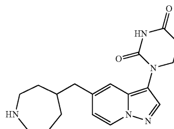
1-(5-(azepan-4-ylmethyl)pyrazolo[1,5-a]pyridin-3-yl)dihydropyrimidine-2,4-(1H,3H)-dione
