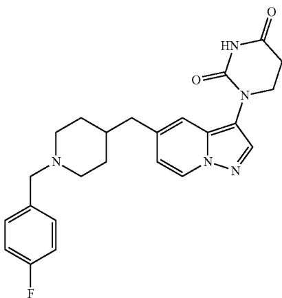
1-(5-((1-(4-fluorobenzyl)piperidin-4-yl)methyl)pyrazolo[1,5-a]pyridin-3-yl)dihydropyrimidine-2,4(1H,3H)-dione
