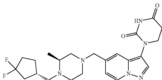
1-(5-(((S)-4-(((S)-3,3-difluorocyclopentyl)methyl)-3-methylpiperazin-1-yl)methyl)pyrazolo[1,5-a]pyridin-3-yl)dihydropyrimidine-2,4(1H,3H)-dione
