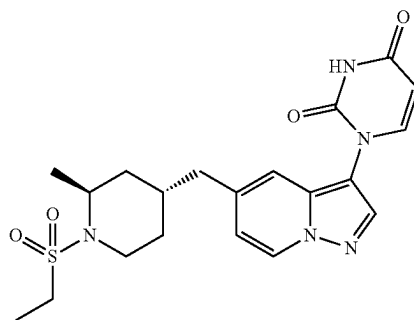
1-(5-(((2S,4R)-1-(ethylsulfonyl)-2-methylpiperidin-4-yl)methyl)pyrazolo[1,5-a]pyridin-3-yl)pyrimidine-2,4(1H,3H)-dione
