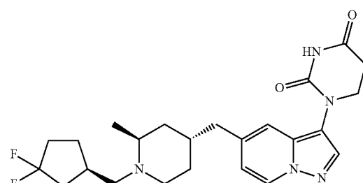
1-(5-(((2S,4R)-1-(((R)-3,3-difluorocyclopentyl)methyl)-2-methylpiperidin-4-yl)methyl)pyrazolo[1,5-a]pyridin-3-yl) dihydropyrimidine-2,4-(1H,3H)-dione
