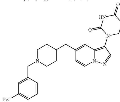
1-(5-((1-(3-(trifluoromethyl)benzyl)piperidin-4-yl)methyl)pyrazolo[1,5-a]pyridin-3-yl)dihydropyrimidine-2,4(1H,3H)-dione
