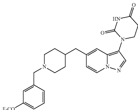
1-(5-((1-(3-(trifluoromethoxy)benzyl)piperidin-4-yl)methyl)pyrazolo[1,5-a]pyridin-3-yl)dihydropyrimidine-2,4(1H,3H)-dione
