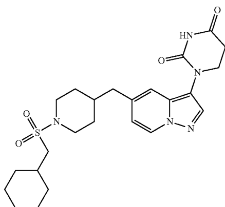
1-(5-((1-((cyclohexylmethyl)sulfonyl)piperidin-4-yl)methyl)pyrazolo[1,5-a]pyridin-3-yl)dihydropyrimidine-2,4(1H,3H)-dione
