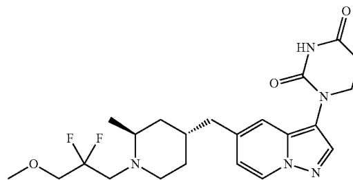
1-(5-(((2S,4R)-1-(2,2-difluoro-3-methoxypropyl)-2- methylpiperidin-4-yl)methyl)pyrazolo[1,5-a]pyridin-3- yl) dihydropyrimidine-2,4(1H,3H)-dione
