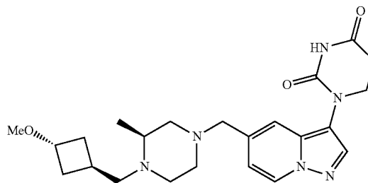
1-(5-(((S)-4-(((1R,3S)-3-methoxycyclobutyl)methyl)-3-methylpiperazin-1-yl)methyl)pyrazolo[1,5-a]pyridin-3-yl) dihydropyrimidine-2,4-(1H,3H)-dione
