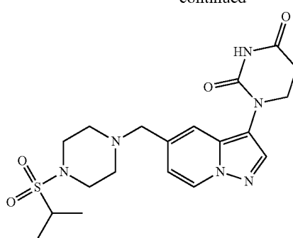
1-(5-((4-isopropylsulfonyl)piperazin-1-yl)methyl)pyrazolo[1,5-a]pyridin-3-yl)dihydropyrimidine-2,4(1H,3H)-dione
