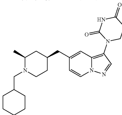
1-(5-(((2S,4S)-1-(cyclohexylmethyl)-2-methylpiperidin-4-yl)methyl)pyrazolo[1,5-a]pyridin-3-yl)dihydropyrimidine-2,4(1H,3H)-dione
