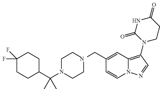
1-(5-((4-(2-(4,4-difluorocyclohexyl)propan-2-yl)piperazin-1-yl)methyl)pyrazolo[1,5-a]pyridin-3-yl)dihydropyrimidine-2,4(1H,3H)-dione
