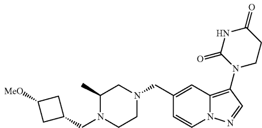
1-(5-(((S)-4-(((1S,3R)-3-methoxycyclobutyl)methyl)-3-methylpiperazin-1-yl)methyl)pyrazolo[1,5-a]pyridin-3-yl)dihydropyrimidine-2,4(1H,3H)-dione
