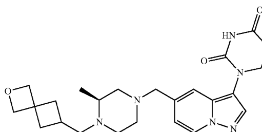
(S)-1-(5-(((4-((2-oxaspiro[3.3]heptan-6-yl)methyl)-3-methylpiperazin-1-yl)methyl)pyrazolo[1,5-a]pyridin-3-yl)dihydropyrimidine-2,4(1H,3H)-dione
