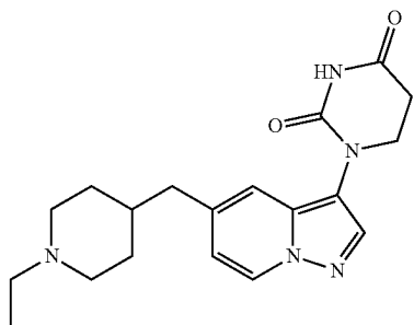
1-(5-((1-ethylpiperidin-4-yl)methyl)pyrazolo[1,5-a]pyridin-3-yl)dihydropyrimidine-2,4(1H,3H)-dione
