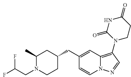
1-(5-(((2S,4R)-1-(2,2-difluoroethyl)-2-methylpiperidin-4-yl) methyl)pyrazolo[1,5-a]pyridin-3-yl) dihydropyrimidine- 2,4(1H,3H)-dione
