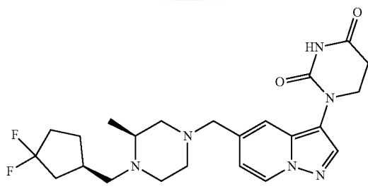
1-(5-(((S)-4-(((R)-3,3-difluorocyclopentyl)methyl)-3-methylpiperazin-1-yl)methyl)pyrazolo[1,5-a]pyridin-3-yl)dihydropyrimidine-2,4(1H,3H)-dione
