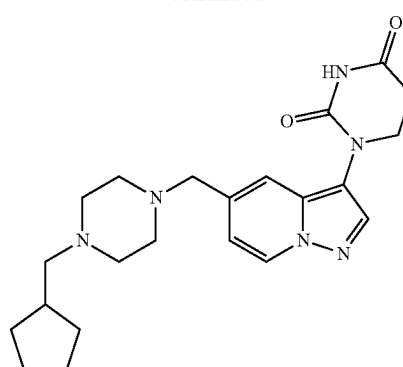
1-(5-((4-(cyclopentylmethyl)piperazin-1-yl)methyl)pyrazolo[1,5-a]pyridin-3-yl)dihydropyrimidine-2,4(1H,3H)-dione
