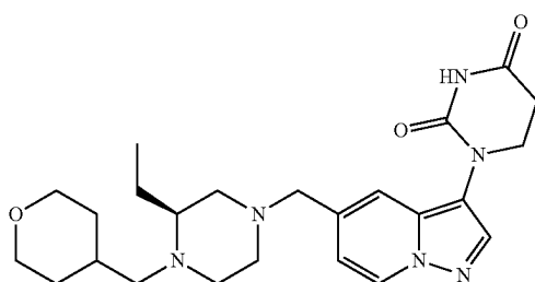
(S)-1-(5-((3-ethyl-4-((tetrahydro-2H-pyran-4-yl)methyl)piperazin-1-yl)methyl)pyrazolo[1,5-a]pyridin-3-yl)dihydropyrimidine-2,4(1H,3H)-dione
