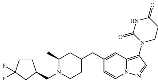
1-(5-(((S)-4-(((R)-3,3-difluorocyclopentyl)methyl)-3-methylpiperazin-1-yl)methyl)pyrazolo[1,5-a]pyridin-3-yl)dihydropyrimidine-2,4-(1H,3H)-dione
