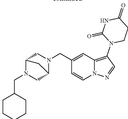
1-(5-(((1S,4S)-5-(cyclohexylmethyl)-2,5-diazabicyclo[2.2.1]heptan-2-yl)methyl)pyrazolo[1,5-a]pyridin-3-yl)dihydropyrimidine-2,4(1H,3H)-dione
