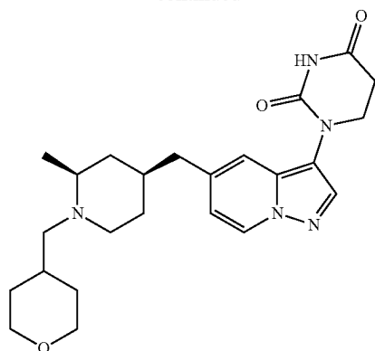
1-(5-(((2S,4S)-2-methyl-1-((tetrahydro-2H-pyran-4-yl)methyl)piperidin-4-yl)methyl)pyrazolo[1,5-a]pyridin-3-yl)dihydropyrimidine-2,4(1H,3H)-dione
