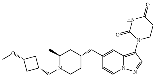
1-(5-(((2S,4R)-1-(((1S,3R)-3-methoxycyclobutyl)methyl)-2-methylpiperidin-4-yl)methyl)pyrazolo[1,5-a]pyridin-3-yl)dihydropyrimidine-2,4(1H,3H)-dione
