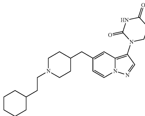
1-(5-((1-(2-cyclohexylethyl)piperidin-4-yl)methyl)pyrazolo[1,5-a]pyridin-3-yl)dihydropyrimidine-2,4(1H,3H)-dione
