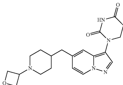
1-(5-((1-(oxetan-3-yl)piperidin-4-yl)methyl)pyrazolo[1,5-a]pyridin-3-yl) dihydropyrimidine-2,4(1H,3H)-dione
