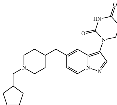
1-(5-((1-(cyclopentylmethyl)piperidin-4-yl)methyl)pyrazolo[1,5-a]pyridin-3-yl)dihydropyrimidine-2,4(1H,3H)-dione
