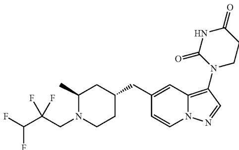
1-(5-(((2S,4R)-2-methyl-1-(2,2,3,3-tetrafluoropropyl) piperidin-4-yl)methyl)pyrazolo[1,5-a]pyridin-3-yl) dihydropyrimidine-2,4-(1H,3H)-dione
