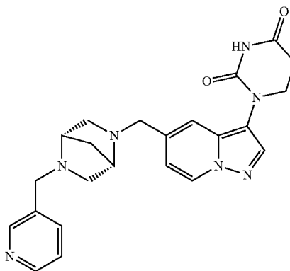
1-(5-(((1S,4S)-5-(pyridin-3-ylmethyl)-2,5-diazabicyclo[2.2.1]heptan-2-yl)methyl)pyrazolo[1,5-a]pyridin-3-yl)dihydropyrimidine-2,4(1H,3H)-dione
