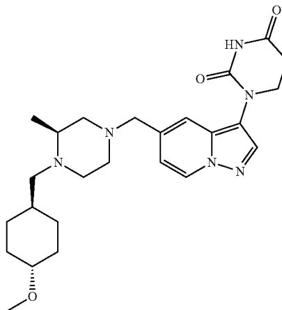
1-(5-(((S)-4-(((1R,4S)-4-methoxycyclohexyl)methyl)-3-methylpiperazin-1-yl)methyl)pyrazolo[1,5-a]pyridin-3-yl)dihydropyrimidine-2,4(1H,3H)-dione
