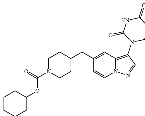
cyclohexyl 4-((3-(2,4-dioxotetrahydropyrimidin-1(2H)-yl)pyrazolo[1,5-a]pyridin-5-yl)methyl)piperidine-1-carboxylate
