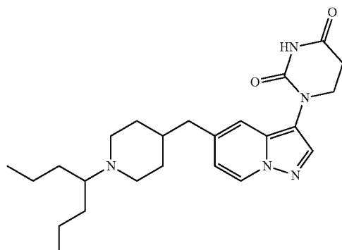
1-(5-((1-(heptan-4-yl)piperidin-4-yl)methyl)pyrazolo[1,5-a]pyridin-3-yl)dihydropyrimidine-2,4(1H,3H)-dione
