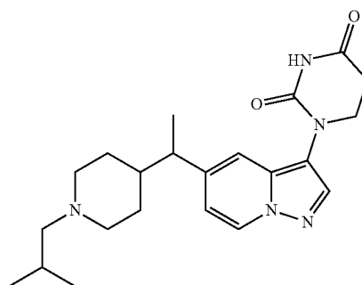
1-((5-((1-(1-isobutylpiperidin-4-yl)ethyl)pyrazolo[1,5-a]pyridin-3-yl)dihydropyrimidine-2,4(1H,3H)-dione
