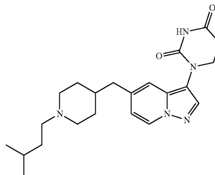
1-(5-((1-(isopentyl)piperidin-4-yl)methyl)pyrazolo[1,5-a]pyridin-3-yl) dihydropyrimidine-2,4(1H,3H)-dione
