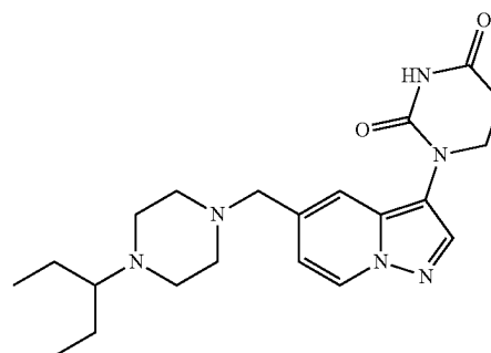
1-(5-((1-(pentan-3-yl)piperidin-4-yl)methyl)pyrazolo[1,5-a]pyridin-3-yl)dihydropyrimidine-2,4(1H,3H)-dione
