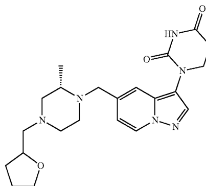
1-(5-(((2S)-2-methyl-4-((tetrahydrofuran-2-yl)methyl)piperazin-1-yl)methyl)pyrazolo[1,5-a]pyridin-3-yl)dihydropyrimidine-2,4(1H,3H)-dione
