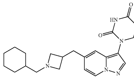
1-(5-((1-(cyclohexylmethyl)azetidin-3-yl)methyl)pyrazolo[1,5-a]pyridin-3-yl)dihydropyrimidine-2,4(1H,3H)-dione
