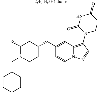
1-(5-(((2R,4R)-1-(cyclohexylmethyl)-2-methylpiperidin-4-yl)methyl)pyrazolo[1,5-a]pyridin-3-yl) dihydropyrimidine-2,4(1H,3H)-dione
