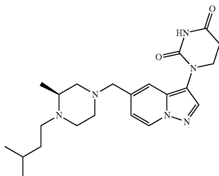
(S)-1-(5-((4-isopentyl-3-methylpiperazin-1-yl)methyl)pyrazolo[1,5-a]pyridin-3-yl)dihydropyrimidine-2,4(1H,3H)-dione
