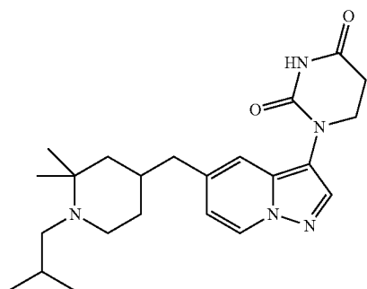
1-(5-((1-isobutyl-2,2-dimethylpiperidin-4-yl)methyl)pyrazolo[1,5-a]pyridin-3-yl)dihydropyrimidine-2,4(1H,3H)-dione
