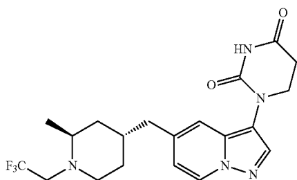
1-(5-(((2S,4R)-2-methyl-1-(2,2,2-trifluoroethyl) piperidin-4-yl)methyl)pyrazolo[1,5-a]pyridin-3- yl) dihydropyrimidine-2,4(1H,3H)-dione
