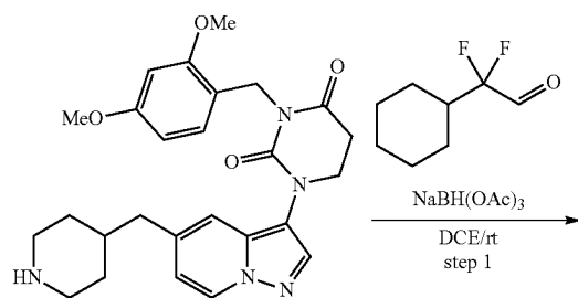
Example 112. Preparation of 1-(5-((1-(2-cyclohexyl-2,2-difluoroethyl)piperidin-4-yl)methyl)pyrazolo[1,5-a]pyridin-3-yl) dihydropyrimidine-2,4(1H, 3H)-dione
