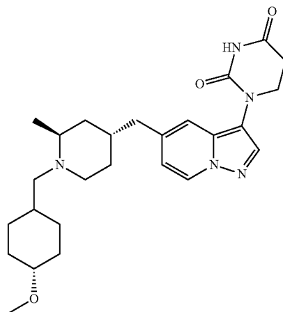
1-(5-(((2S,4R)-1-(((1r,4S)-4-methoxycyclohexyl)methyl)-2-methylpiperidin-4-yl)methyl)pyrazolo[1,5-a]pyridin-3-yl)dihydropyrimidine-2,4(1H,3H)-dione
