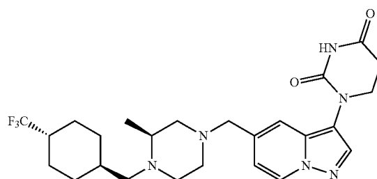
1-(5-(((S)-3-methyl-4-(((1R,4S)-4-(trifluoromethyl)cyclohexyl)methyl)piperazin-1-yl)methyl)pyrazolo[1,5-a]pyridin-3-yl)dihydropyrimidine-2,4(1H,3H)-dione
