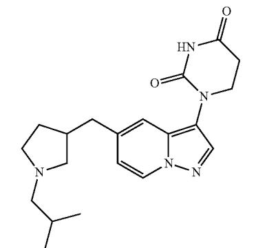
1-(5-((1-(isobutyl)pyrrolidin-3-yl)methyl)pyrazolo[1,5-a]pyridin-3-yl) dihydropyrimidine-2,4(1H,3H)-dione
