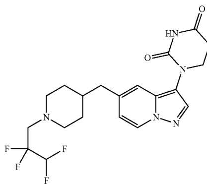
1-(5-((1-(2,2,3,3-tetrafluoropropyl)piperidin-4-yl)methyl)pyrazolo[1,5-a]pyridin-3-yl)dihydropyrimidine-2,4(1H,3H)-dione
