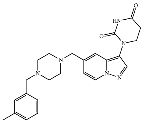
1-(5-((4-(3-methylbenzyl)piperazin-1-yl)methyl)pyrazolo[1,5-a]pyridin-3-yl)dihydropyrimidine-2,4(1H,3H)-dione
