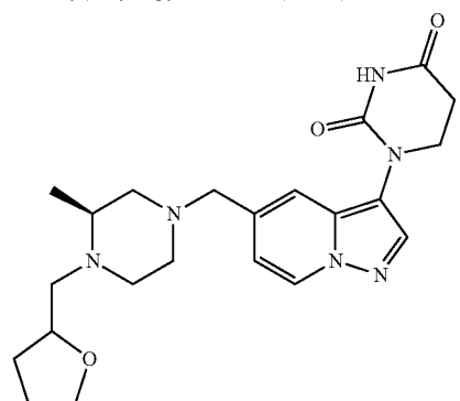
1-(5-(((3S)-3-methyl-4-((tetrahydrofuran-2-yl)methyl)piperazin-1-yl)methyl)pyrazolo[1,5-a]pyridin-3-yl)dihydropyrimidine-2,4(1H,3H)-dione
