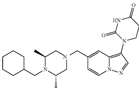
1-(5-(((3S,5S)-4-(cyclohexylmethyl)-3,5-dimethylpiperazin-1-yl)methyl)pyrazolo[1,5-a]pyridin-3-yl)dihydropyrimidine-2,4(1H,3H)-dione
