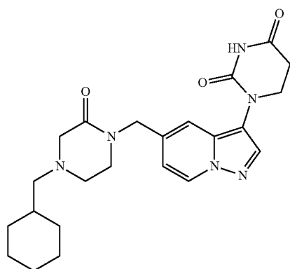
1-(5-((4-(cyclohexylmethyl)-2-oxopiperazin-1-yl)methyl)pyrazolo[1,5-a]pyridin-3-yl)dihydropyrimidine-2,4(1H,3H)-dione
