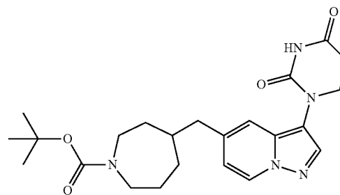
tert-butyl 4-((3-(2,4-dioxotetrahydropyrimidin-1(2H)-yl)pyrazolo[1,5-a]pyridin-5-yl)methyl)azepane-1-carboxylate
