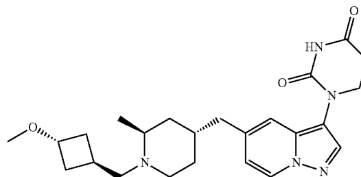
1-(5-(((2S,4R)-1-(((1r,3S)-3-methoxycyclobutyl)methyl)-2-methylpiperidin-4-yl)methyl)pyrazolo[1,5-a]pyridin-3-yl) dihydropyrimidine-2,4(1H,3H)-dione
