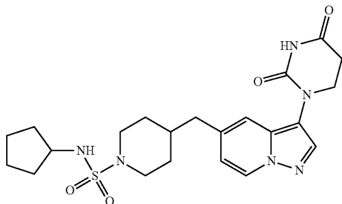
N-cyclopentyl-4-((3-(2,4-dioxotetrahydropyrimidin-1(2H)-yl)pyrazolo[1,5-a]pyridin-5-yl)piperidine-1-sulfonamide
