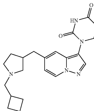
1-(5-((1-(cyclobutylmethyl)pyrrolidin-3-yl)methyl)pyrazolo[1,5-a]pyridin-3-yl) dihydropyrimidine-2,4(1H,3H)-dione
