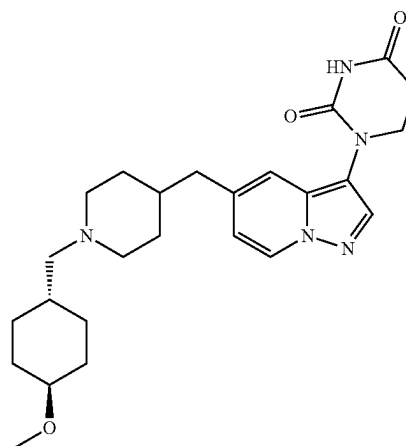
1-(5-(((1r,4r)-4-methoxycyclohexyl)methyl)piperidin-4-yl)methylpyrazolo[1,5-a]pyridin-3-yl)dihydropyrimidine-2,4(1H,3H)-dione
