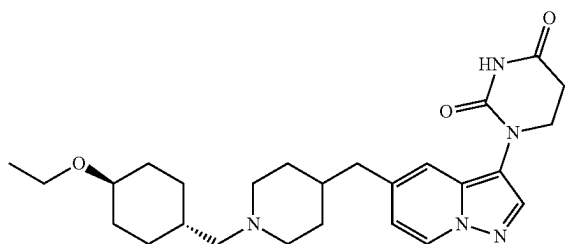
1-(5-((1-(((1R,4R)-4-ethoxycyclohexyl)methyl)piperidin-4-yl)methyl)pyrazolo[1,5-a]pyridin-3-yl)dihydropyrimidine-2,4(1H,3H)-dione
