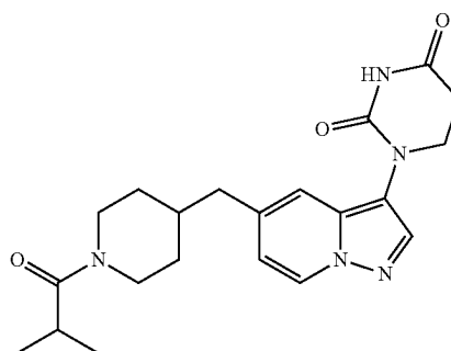
1-(5-((1-(isobutyryl)piperidin-4-yl)methyl)pyrazolo[1,5-a]pyridin-3-yl)dihydropyrimidine-2,4(1H,3H)-dione
