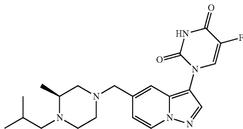
(S)-5-fluoro-1-(5-((4-isobutyl-3-methylpiperazin-1-yl)methyl)pyrazolo[1,5-a]pyridin-3-yl)pyrimidine-2,4(1H,3H)-dione
