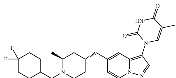
1-(5-(((2S,4R)-1-((4,4-difluorocyclohexyl)methyl)-2-methylpiperidin-4-yl)methyl)pyrazolo[1,5-a]pyridin-3-yl)-5-methylpyrimidine-2,4(1H,3H)-dione
