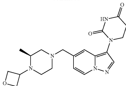
(S)-1-(5-((3-methyl-4-(oxetan-3-yl)piperazin-1-yl)methyl)pyrazolo[1,5-a]pyridin-3-yl)dihydropyrimidine-2,4(1H,3H)-dione
