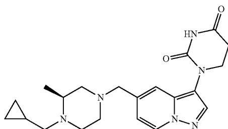
(S)-1-(5-(((4-(cyclopropylmethyl)-3-methylpiperazin-1-yl)methyl)pyrazolo[1,5-a]pyridin-3-yl)dihydropyrimidine-2,4(1H,3H)-dione
