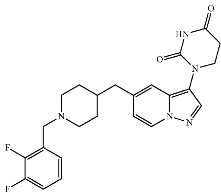
1-(5-((1-(2,3-difluorobenzyl)piperidin-4-yl)methyl)pyrazolo[1,5-a]pyridin-3-yl)dihydropyrimidine-2,4(1H,3H)-dione
