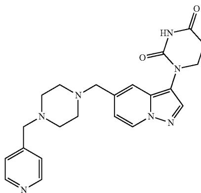
1-(5-((4-(pyridin-4-ylmethyl)piperazin-1-yl)methyl)pyrazolo[1,5-a]pyridin-3-yl) dihydropyrimidine-2,4(1H,3H)-dione
