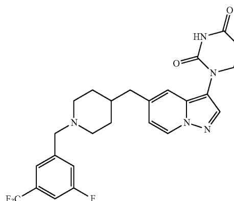
1-(5-((1-(3-fluoro-5-(trifluoromethyl)benzyl)piperidin-4-yl)methyl)pyrazolo[1,5-a]pyridin-3-yl) dihydropyrimidine-2,4(1H,3H)-dione
