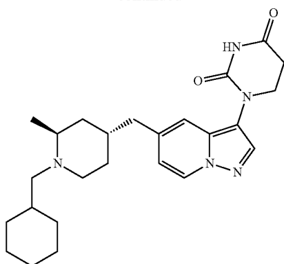
1-(5-(((2S,4R)-1-(cyclohexylmethyl)-2-methylpiperidin-4-yl)methyl)pyrazolo[1,5-a]pyridin-3-yl)dihydropyrimidine-2,4(1H,3H)-dione
