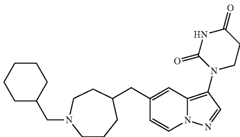
1-(5-((1-cyclohexylmethyl)azepan-4-yl)methyl)pyrazolo [1,5-a]pyridin-3-yl) dihydropyrimidine-2,4 (1H,3H)-dione
