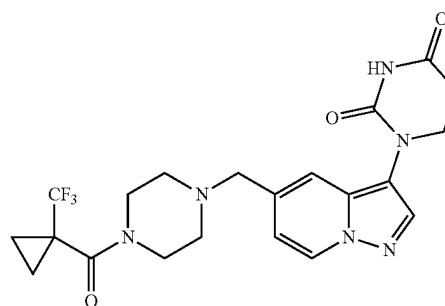
1-(5-((4-(1-(trifluoromethyl)cyclopropane-1-carbonyl)piperazin-1-yl)methyl)pyrazolo[1,5-a]pyridin-3-yl)dihydropyrimidine-2,4(1H,3H)-dione
