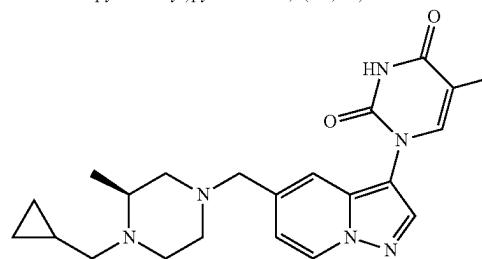
(S)-1-(5-((4-(cyclopropylmethyl)-3-methylpiperazin-1-yl)methyl)pyrazolo[1,5-a]pyridin-3-yl)-5-methylpyrimidine-2,4(1H,3H)-dione
