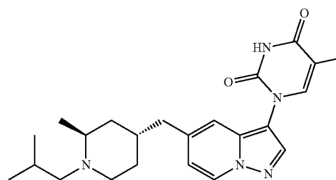
1-(5-(((2S,4R)-1-isobutyl-2-methylpiperidin-4-yl)methyl)pyrazolo[1,5-a]pyridin-3-yl)-5-methylpyrimidine-2,4(1H,3H)-dione
