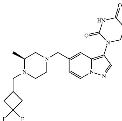
(S)-1-(5-((4-((3,3-difluorocyclobutyl)methyl)piperazin-1-yl)methyl)pyrazolo[1,5-a]pyridin-3-yl) dihydropyrimidine-2,4(1H,3H)-dione
