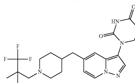
1-(5-((1-(3,3,3-trifluoro-2,2-dimethylpropyl)piperidin-4-yl)methyl)pyrazolo[1,5-a]pyridin-3-yl)dihydropyrimidine-2,4(1H,3H)-dione
