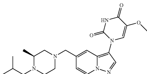
(S)-1-(5-((4-isobutyl-3-methylpiperazin-1-yl)methyl)pyrazolo[1,5-a]pyridin-3-yl)-5-methoxypyrimidine-2,4(1H,3H)-dione
