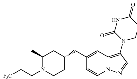
1-(5-(((2S,4R)-2-methyl-1-(3,3,3-trifluoropropyl) piperidin-4-yl)methyl)pyrazolo[1,5-a]pyridin-3-yl) dihydropyrimidine-2,4(1H,3H)-dione
