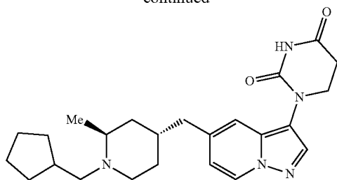
1-(5-(((2S,4R)-1-(cyclopentylmethyl)-2-methylpiperidin-4-yl)methyl)pyrazolo[1,5-a]pyridin-3-yl)dihydropyrimidine-2,4(1H,3H)-dione
