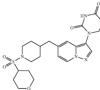
1-(5-((1-((tetrahydro-2H-pyran-4-yl)sulfonyl)piperidin-4-yl)methyl)pyrazolo[1,5-a]pyridin-3-yl) dihydropyrimidine-2,4(1H,3H)-dione
