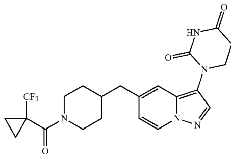
1-(5-((1-(1-trifluoromethyl)cyclopropane-1-carbonyl)piperidin-4-yl)methyl)pyrazolo[1,5-a]pyridin-3-yl) dihydropyrimidine-2,4(1H,3H)-dione
