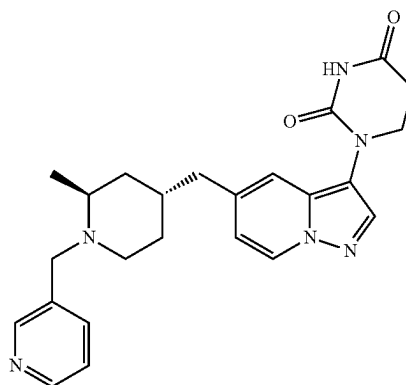
1-(5-(((2S,4R)-2-methyl-1-(pyridin-3-ylmethyl)piperidin-4-yl)piperidin-4-yl)methyl)pyrazolo[1,5-a]pyridin-3-yl)dihydropyrimidine-2,4(1H,3H)-dione
