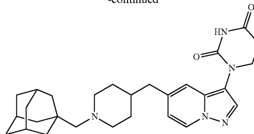
1-(5-(((1-((3r,5r,7r)-adamantan-1-yl)methyl)piperidin-4-yl)methyl)pyrazolo[1,5-a]pyridin-3-yl)dihydropyrimidine-2,4(1H,3H)-dione
