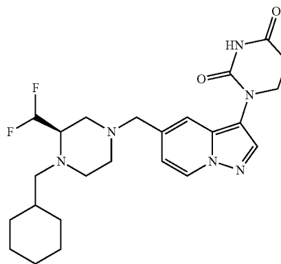
(R)-1-(5-((4-(cyclohexylmethyl)-3-(difluoromethyl)piperazin-1-yl)methyl)pyrazolo[1,5-a]pyridin-3-yl)dihydropyrimidine-2,4(1H,3H)-dione
