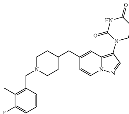
1-(5-((1-(3-fluoro-2-methylbenzyl)piperidin-4-yl)methyl)pyrazolo[1,5-a]pyridin-3-yl) dihydropyrimidine-2,4(1H,3H)-dione
