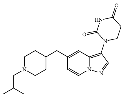
1-(5-((1-isobutyl)piperidin-4-yl)methyl)pyrazolo[1,5-a]pyridin-3-yl) dihydropyrimidine-2,4(1H,3H)-dione
