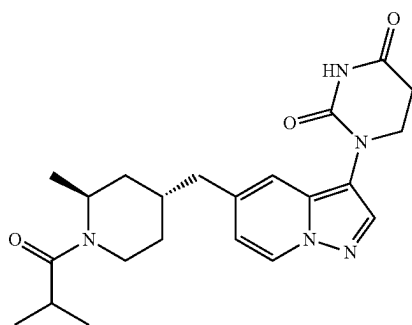
1-(5-(((2S,4R)-1-isobutyryl-2-methylpiperidin-4-yl)methyl)pyrazolo[1,5-a]pyridin-3-yl)dihydropyrimidine-2,4(1H,3H)-dione
