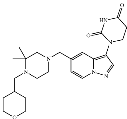
1-(5-((3,3-dimethyl-4-((tetrahydro-2H-pyran-4-yl)methyl)piperazin-1-yl)methyl)pyrazolo[1,5-a]pyridin-3-yl)dihydropyrimidine-2,4(1H,3H)-dione
