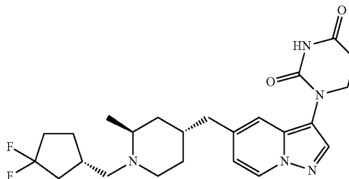
1-(5-(((2S,4R)-1-(((S)-3,3-difluorocyclopentyl)methyl)-2-methylpiperidin-4-yl)methyl)pyrazolo[1,5-a]pyridin-3-yl)dihydropyrimidine-2,4(1H,3H)-dione
