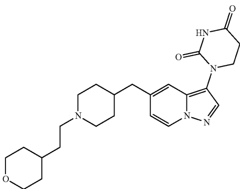
1-(5-((1-(2-(tetrahydro-2H-pyran-4-yl)ethyl)piperidin-4-yl)methyl)pyrazolo[1,5-a]pyridin-3-yl)dihydropyrimidine-2,4(1H,3H)-dione
