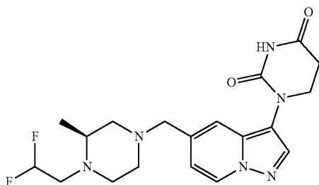
(S)-1-(5-((4-(2,2-difluoroethyl)-3-methylpiperazin-1-yl)methyl)pyrazolo[1,5-a]pyridin-3-yl)dihydropyrimidine-2,4(1H,3H)-dione
