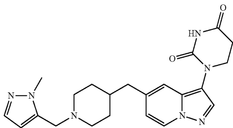
1-(5-((1-((1-methyl-1H-pyrazol-5-yl)methyl)piperidin-4-yl)methyl)pyrazolo[1,5-a]pyridin-3-yl)dihydropyrimidine-2,4(1H,3H)-dione
