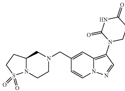
(S)-1-(5-(((1,1-dioxidohexahydro-5H-isothiazolo[2,3-a]pyrazin-5-yl)methyl)pyrazolo[1,5-a]pyridin-3-yl)dihydropyrimidine-2,4(1H,3H)-dione
