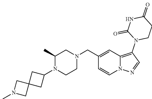
(S)-1-(5-((3-methyl-4-(2-methyl-2-azaspiro[3.3]heptan-6-yl)piperazin-1-yl)methyl)pyrazolo[1,5-a]pyridin-3-yl)dihydropyrimidine-2,4(1H,3H)-dione
