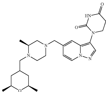
1-(5-(((3S)-4-(((2R,6S)-2,6-dimethyltetrahydro-2H-pyran-4-yl)methyl)-3-methylpiperazin-1-yl)methyl)pyrazolo[1,5-a]pyridin-3-yl)dihydropyrimidine-2,4(1H,3H)-dione
