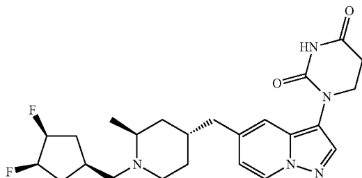
1-(5-(((2S,4R)-1-(((1R,3R,4S)-3,4-difluorocyclopentyl)methyl)-2-methylpiperidin-4-yl)methyl)pyrazolo[1,5-a]pyridin-3-yl)dihydropyrimidine-2,4(1H,3H)-dione
