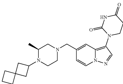
(S)-1-(5-((3-methyl-4-(spiro[3.3]heptan-2-yl)piperazin-1-yl)methyl)pyrazolo[1,5-a]pyridin-3-yl)dihydropyrimidine-2,4(1H,3H)-dione
