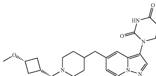
1-(5-(((1s,3s)-3-methoxycyclobutyl)methyl)piperidin-4-yl)methyl)pyrazolo[1,5-a]pyridin-3-yl) dihydropyrimidine-2,4(1H,3H)-dione
