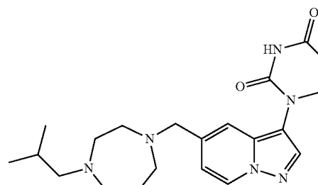
1-(5-((4-isobutyl-1,4-diazepan-1-yl)methyl)pyrazolo[1,5-a]pyridin-3-yl)dihydropyrimidine-2,4(1H,3H)-dione
