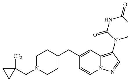
1-(5-((1-((1-(trifluoromethyl)cyclopropyl)methyl)piperidin-4-yl)methyl)pyrazolo[1,5-a]pyridin-3-yl)dihydropyrimidine-2,4(1H,3H)-dione
