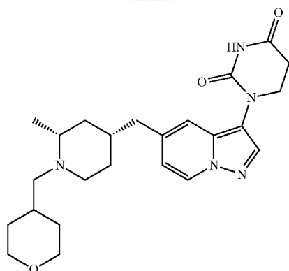
1-(5-(((2R,4R)-2-methyl-1-((tetrahydro-2H-pyran-4-yl)methyl)piperidin-4-yl)methyl)pyrazolo[1,5-a]pyridin-3-yl)dihydropyrimidine-2,4(1H,3H)-dione
