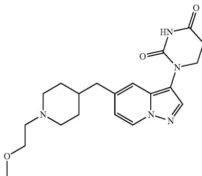
1-(5-((1-(2-methoxyethyl)piperidin-4-yl)methyl)pyrazolo[1,5-a]pyridin-3-yl)dihydropyrimidine-2,4(1H,3H)-dione
