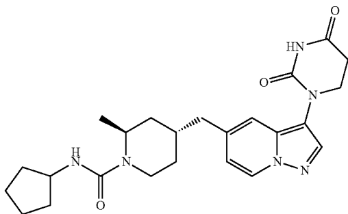
(2S,4R)-N-cyclopentyl-4-((3-(2,4-dioxotetrahydropyrimidin-1(2H)-yl)pyrazolo[1,5-a]pyridin-5-yl)methyl)-2-methylpiperidine-1-carboxamide
