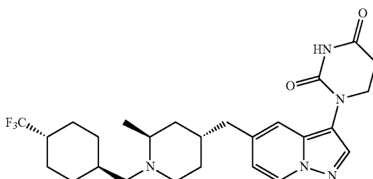
1-(5-(((2S,4R)-2-methyl-1-(((1R,4S)-4-(trifluoromethyl)cyclohexyl)methyl)piperidin-4-yl)methyl)pyrazolo[1,5-a]pyridin-3-yl)dihydropyrimidine-2,4(1H,3H)-dione
