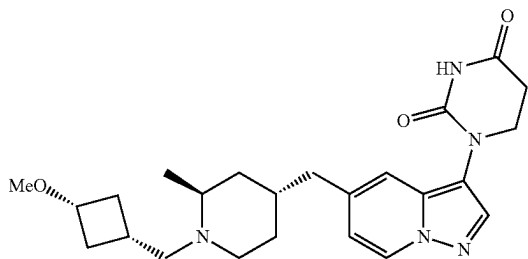
1-(5-(((2S,4R)-1-(((1S,3R)-3-methoxycyclobutyl)methyl)-2-methylpiperidin-4-yl)methyl)pyrazolo[1,5-a]pyridin-3-yl)dihydropyrimidine-2,4-(1H,3H)-dione
