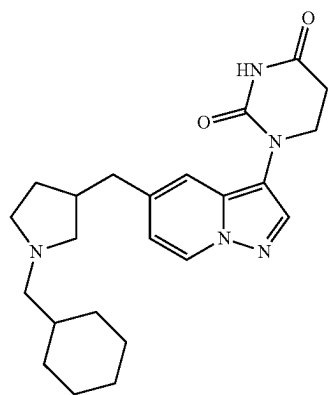
1-(5-((1-(cyclohexylmethyl)pyrrolidin-3-yl)methyl)pyrazolo[1,5-a]pyridin-3-yl) dihydropyrimidine-2,4(1H,3H)-dione
