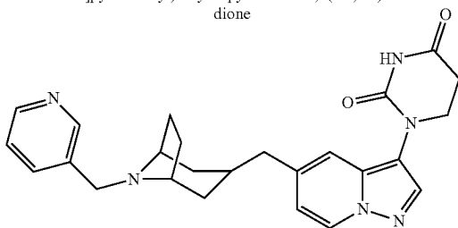
1-(5-(((1R,5S)-8-(pyridin-3-ylmethyl)-8-azabicyclo[3.2.1]octan-3-yl)methyl)pyrazolo[1,5-a]pyridin-3-yl)dihydropyrimidine-2,4(1H,3H)-dione
