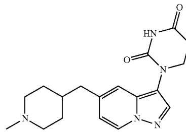
1-(5-((1-methylpiperidin-4-yl)methyl)pyrazolo[1,5-a]pyridin-3-yl)dihydropyrimidine-2,4(1H,3H)-dione
