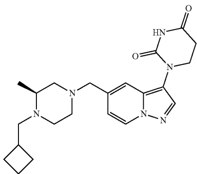
(S)-1-(5-((4-(cyclobutylmethyl)-3-methylpiperazin-1-yl)methyl)pyrazolo[1,5-a]pyridin-3-yl) dihydropyrimidine-2,4(1H,3H)-dione
