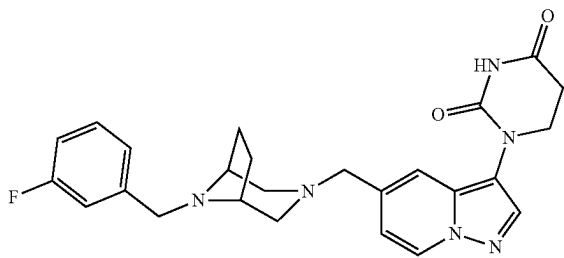
1-(5-(((1R,5S)-8-(3-fluorobenzyl)-3,8-diazabicyclo[3.2.1]octan-3-yl)methyl)pyrazolo[1,5-a]pyridin-3-yl) dihydropyrimidine-2,4(1H,3H)-dione
