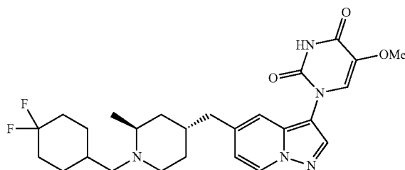
1-(5-(((2S,4R)-1-((4,4-difluorocyclohexyl)methyl)-2-methylpiperidin-4-yl)methyl)pyrazolo[1,5-a]pyridin-3-yl)-5-methoxypyrimidine-2,4(1H,3H)-dione
