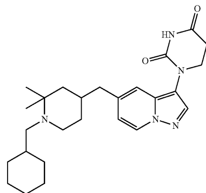
1-(5-((4-(cyclohexylmethyl)-3,3-dimethylpiperazin-1-yl)methyl)pyrazolo[1,5-a]pyridin-3-yl)dihydropyrimidine-2,4(1H,3H)-dione
