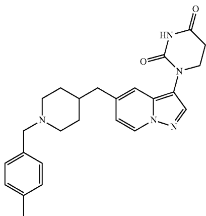
1-(5-((1-(4-methylbenzyl)piperidin-4-yl)methyl)pyrazolo[1,5-a]pyridin-3-yl) dihydropyrimidine-2,4(1H,3H)-dione
