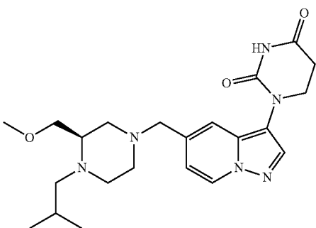
(R)-1-(5-((4-isobutyl-3-(methoxymethyl)piperazin-1-yl)methyl)pyrazolo[1,5-a]pyridin-3-yl)dihydropyrimidine-2,4(1H,3H)-dione
