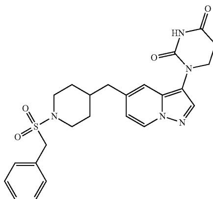
1-(5-((1-(benzylsulfonyl)piperidin-4-yl)methyl)pyrazolo[1,5-a]pyridin-3-yl)dihydropyrimidine-2,4(1H,3H)-dione
