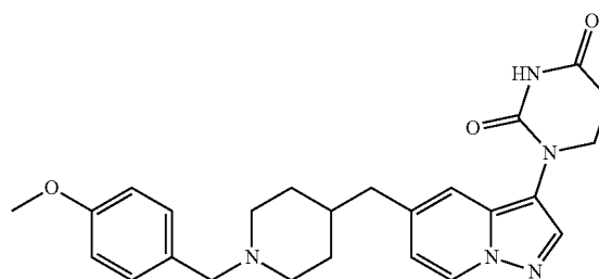
1-(5-((1-(4-methoxybenzyl)piperidin-4-yl)methyl)pyrazolo[1,5-a]pyridin-3-yl)dihydropyrimidine-2,4(1H,3H)-dione
