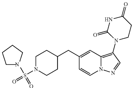
1-(5-(((1-(pyrrolidin-1-yl)sulfonyl)piperidin-4-yl)methyl)pyrazolo[1,5-a]pyridin-3-yl) dihydropyrimidine-2,4(1H,3H)-dione
