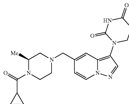
(S)-1-(5-((4-(cyclopropanecarbonyl)-3-methylpiperazin-1-yl)methyl)pyrazolo[1,5-a]pyridin-3-yl)dihydropyrimidine-2,4(1H,3H)-dione
