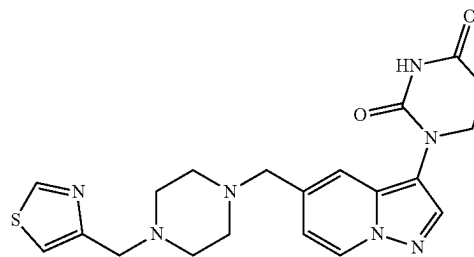
1-(5-((4-(thiazol-4-ylmethyl)piperazin-1-yl)methyl)pyrazolo[1,5-a]pyridin-3-yl) dihydropyrimidine-2,4(1H,3H)-dione
