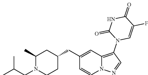
5-fluoro-1-(5-(((2S,4R)-1-isobutyl-2-methylpiperidin-4-yl)methyl)pyrazolo[1,5-a]pyridin-3-yl)pyrimidine-2,4(1H,3H)-dione
