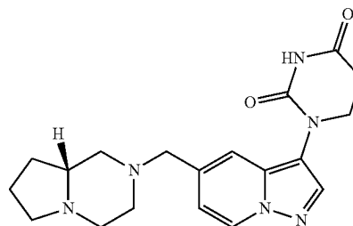
(R)-1-(5-((hexahydropyrrolo[1,2-a]pyrazin-2(1H)-yl)methyl)pyrazolo[1,5-a]pyridin-3-yl)dihydropyrimidine-2,4(1H,3H)-dione
