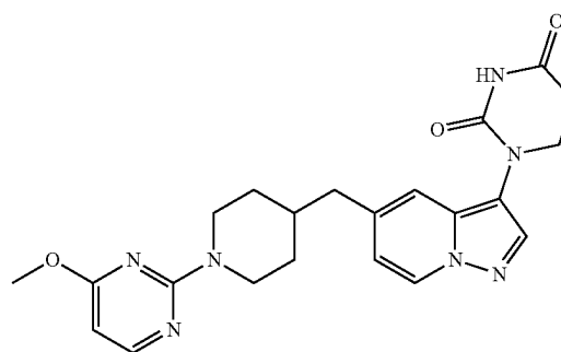
1-(5-((1-(4-methoxypyrimidin-2-yl)piperidin-4-yl)methyl)pyrazolo[1,5-a]pyridin-3-yl)dihydropyrimidine-2,4(1H,3H)-dione
