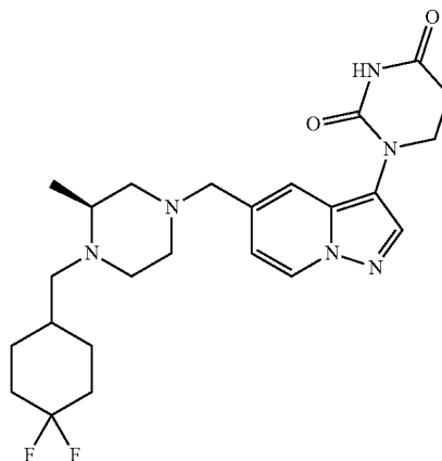
(S)-1-(5-((4-((4,4-difluorocyclohexyl)methyl)-3-methylpiperazin-1-yl)methyl)pyrazolo[1,5-a]pyridin-3-yl)dihydropyrimidine-2,4(1H,3H)-dione
