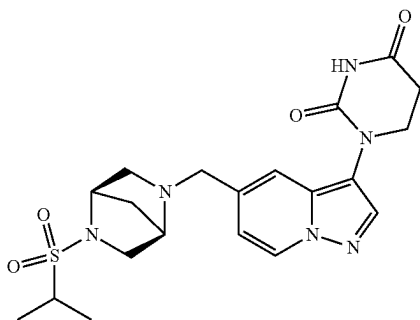
1-(5-(((1R,4R)-5-(isopropylsulfonyl)-2,5-diazabicyclo[2.2.1]heptan-2-yl)methyl)pyrazolo[1,5-a]pyridin-3-yl)dihydropyrimidine-2,4(1H,3H)-dione
