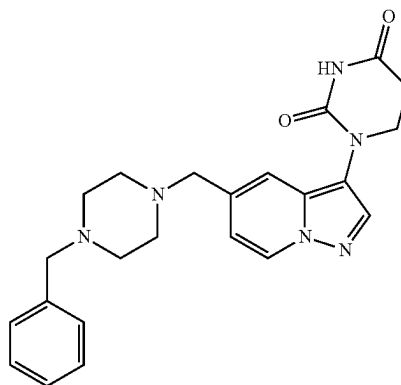
1-(5-((4-benzylpiperazin-1-yl)methyl)pyrazolo[1,5-a]pyridin-3-yl)dihydropyrimidine-2,4(1H,3H)-dione
