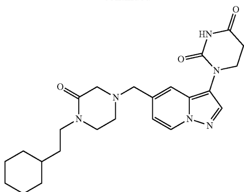
1-(5-((4-(2-cyclohexylethyl)-3-oxopiperazin-1-yl)methyl)pyrazolo[1,5-a]pyridin-3-yl)dihydropyrimidine-2,4(1H,3H)-dione
