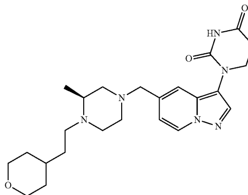
(S)-1-(5-((3-methyl-4-(2-(tetrahydro-2H-pyran-4-yl)ethyl)piperazin-1-yl)methyl)pyrazolo[1,5-a]pyridin-3-yl) dihydropyrimidine-2,4(1H,3H)-dione
