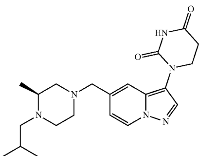
(S)-1-(5-((4-isobutyl-3-methylpiperazin-1-yl)methyl)pyrazolo[1,5-a]pyridin-3-yl)dihydropyrimidine-2,4(1H,3H)-dione
