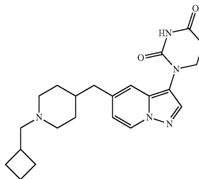
1-(5-((1-(cyclobutylmethyl)piperidin-4-yl)methyl)pyrazolo[1,5-a]pyridin-3-yl) dihydropyrimidine-2,4(1H,3H)-dione
