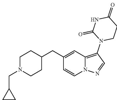
1-(5-((1-(cyclopropylmethyl)piperidin-4-yl)methyl)pyrazolo[1,5-a]pyridin-3-yl)dihydropyrimidine-2,4(1H,3H)-dione
