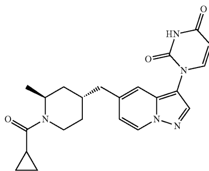
1-(5-(((2S,4R)-1-(cyclopropanecarbonyl)-2-methylpiperidin-4-yl)methyl)pyrazolo[1,5-a]pyridin-3-yl)pyrimidine-2,4(1H,3H)-dione
