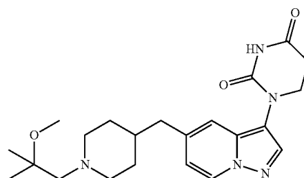
1-(5-((1-(2-methoxy-2-methylpropyl)piperidin-4-yl)methyl)pyrazolo[1,5-a]pyridin-3-yl)dihydropyrimidine-2,4(1H,3H)-dione
