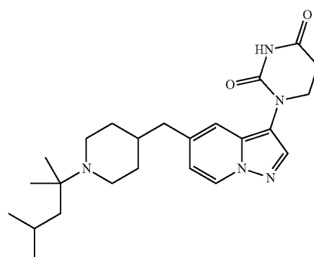
1-(5-((1-(2,4-dimethylpentan-2-yl)piperidin-4-yl)methyl)pyrazolo[1,5-a]pyridin-3-yl)dihydropyrimidine-2,4(1H,3H)-dione
