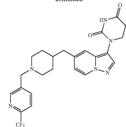
1-(5-((1-((6-(trifluoromethyl)pyridin-3-yl)methyl)piperidin-4-yl)methyl)pyrazolo[1,5-a]pyridin-3-yl)dihydropyrimidine-2,4(1H,3H)-dione
