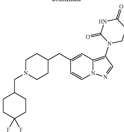
1-(5-((1-((4,4-difluorocyclohexyl)methyl)piperidin-4-yl)methyl)pyrazolo[1,5-a]pyridin-3-yl) dihydropyrimidine-2,4(1H,3H)-dione
