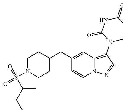
1-(5-((1-(sec-butylsulfonyl)piperidin-4-yl)methyl)pyrazolo[1,5-a]pyridin-3-yl)dihydropyrimidine-2,4(1H,3H)-dione
