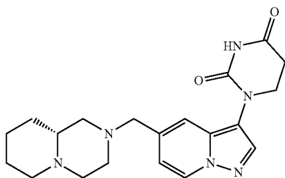
(R)-1-(5-((octahydro-2H-pyrido[1,2-a]pyrazin-2-yl)methyl)pyrazolo[1,5-a]pyridin-3-yl)dihydropyrimidine-2,4(1H,3H)-dione
