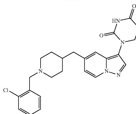
1-(5-((1-(2-chlorobenzyl)piperidin-4-yl)methyl)pyrazolo[1,5-a]pyridin-3-yl)dihydropyrimidine-2,4(1H,3H)-dione
