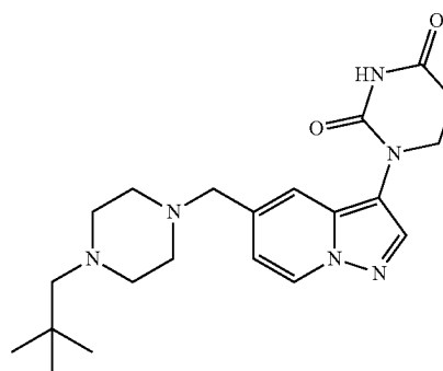
1-(5-((1-neopentylpiperidin-4-yl)methyl)pyrazolo[1,5-a]pyridin-3-yl)dihydropyrimidine-2,4(1H,3H)-dione
