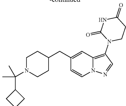
1-(5-((1-(2-cyclobutylpropan-2-yl)piperidin-4-yl)methyl)pyrazolo[1,5-a]pyridin-3-yl)dihydropyrimidine-2,4(1H,3H)-dione
