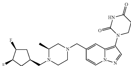
1-(5-(((S)-4-(((1R,3R,4S)-3,4-difluorocyclopentyl)methyl)-3-methylpiperazin-1-yl)methyl)pyrazolo[1,5-a]pyridin-3-yl)dihydropyrimidine-2,4-(1H,3H)-dione
