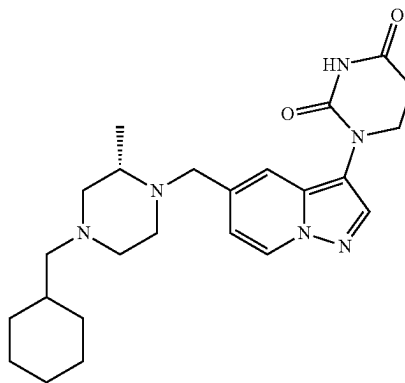
(S)-1-(5-((4-(cyclohexylmethyl)-2-methylpiperazin-1-yl)methyl)pyrazolo[1,5-a]pyridin-3-yl)dihydropyrimidine-2,4(1H,3H)-dione
