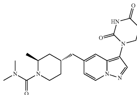
(2S,4R)-4-((3-(2,4-dioxotetrahydropyrimidin-1(2H)-yl)pyrazolo[1,5-a]pyridin-5-yl)methyl)-N,N,2-trimethylpiperidine-1-carboxamide
