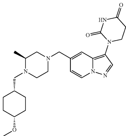
1-(5-(((S)-4-((1S,4R)-4-methoxycyclohexyl)methyl)-3-methylpiperazin-1-yl)methyl)pyrazolo[1,5-a]pyridin-3-yl)dihydropyrimidine-2,4(1H,3H)-dione
