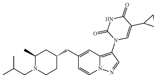
5-cyclopropyl-1-(5-(((2S,4R)-1-isobutyl-2-methylpiperidin-4-yl)methyl)pyrazolo[1,5-a]pyridin-3-yl)pyrimidine-2,4(1H,3H)-dione
