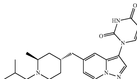
1-(5-(((2S,4R)-1-isobutyl-2-methylpiperidin-4-yl)methyl)pyrazolo[1,5-a]pyridin-3-yl)pyrimidine-2,4(1H,3H)-dione
