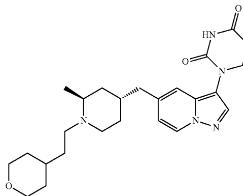
1-(5-(((2S,4R)-2-methyl-1-(2-(tetrahydro-2H-pyran-4-yl)ethyl)piperidin-4-yl)methyl)pyrazolo[1,5-a]pyridin-3-yl) dihydropyrimidine-2,4(1H,3H)-dione
