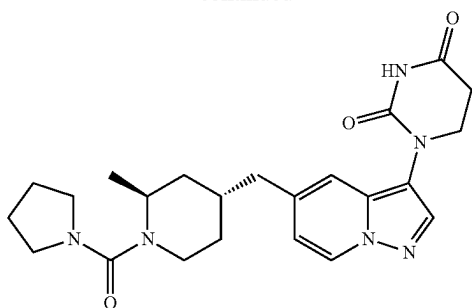
1-(5-(((2S,4R)-2-methyl-1-(pyrrolidin-1-yl)carbamoyl)piperidin-4-yl)methyl)pyrazolo[1,5-a]pyridin-3-yl) dihydropyrimidine-2,4(1H,3H)-dione
