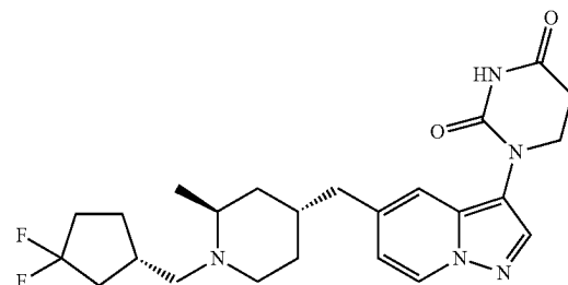
1-(5-(((2S,4R)-1-(((S)-3,3-difluorocyclopentyl)methyl)-2-methylpiperidin-4-yl)methyl)pyrazolo[1,5-a]pyridin-3-yl) dihydropyrimidine-2,4-(1H,3H)-dione
