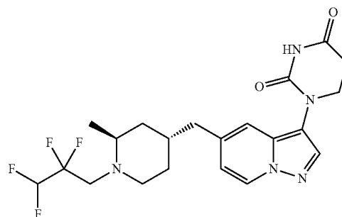
1-(5-(((2S,4R)-2-methyl-1-(2,2,3,3-tetrafluoropropyl)piperidin-4-yl)methyl)pyrazolo[1,5-a]pyridin-3-yl)dihydropyrimidine-2,4(1H,3H)-dione
