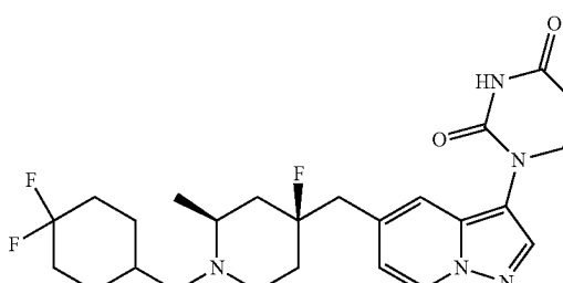
1-(5-(((2S,4S)-1-(((4,4-difluorocyclohexyl)methyl)-4-fluoro-2-methylpiperidin-4-yl)methyl)pyrazolo[1,5-a]pyridin-3-yl)dihydropyrimidine-2,4(1H,3H)-dione
