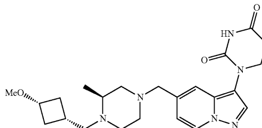
1-(5-(((S)-4-(((1R,3R)-3-methoxycyclobutyl)methyl)-3-methylpiperazin-1-yl)methyl)pyrazolo[1,5-a]pyridin-3-yl) dihydropyrimidine-2,4-(1H,3H)-dione
