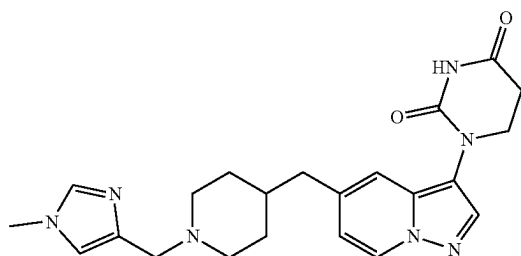
1-(5-((1-((1-methyl-1H-imidazol-4-yl)methyl)piperidin-4-yl)methyl)pyrazolo[1,5-a]pyridin-3-yl) dihydropyrimidine-2,4(1H,3H)-dione
