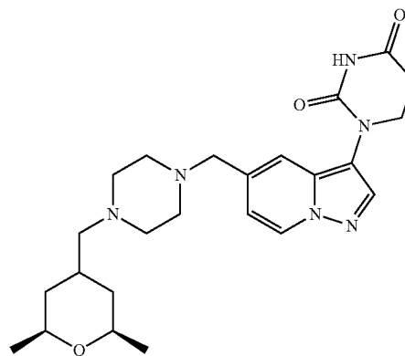
1-((5-(((4-(((2R,6S)-2,6-dimethyltetrahydro-2H-pyran-4-yl)methyl)piperazin-1-yl)methyl)pyrazolo[1,5-a]pyridin-3-yl)dihydropyrimidine-2,4(1H,3H)-dione
