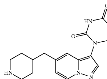
1-(5-(piperidin-4-ylmethyl)pyrazolo[1,5-a]pyridin-3-yl)dihydropyrimidine-2,4(1H,3H)-dione
