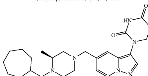
(S)-1-(5-((4-(cycloheptylmethyl)-3-methylpiperazin-1-yl)methyl)pyrazolo[1,5-a]pyridin-3-yl)dihydropyrimidine-2,4(1H,3H)-dione
