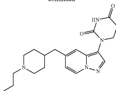
1-(5-((4-propylpiperazin-1-yl)methyl)pyrazolo[1,5-a]pyridin-3-yl)dihydropyrimidine-2,4(1H,3H)-dione
