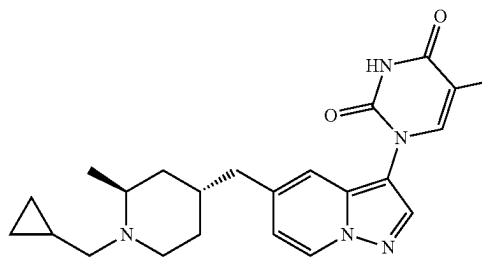
1-(5-(((2S,4R)-1-(cyclopropylmethyl)-2-methylpiperidin-4-yl)methyl)pyrazolo[1,5-a]pyridin-3-yl)-5-methylpyrimidine-2,4(1H,3H)-dione
