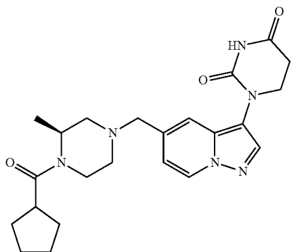
(S)-1-(5-((4-(cyclopentanecarbonyl)-3-methylpiperazin-1-yl)methyl)pyrazolo[1,5-a]pyridin-3-yl)dihydropyrimidine-2,4(1H,3H)-dione
