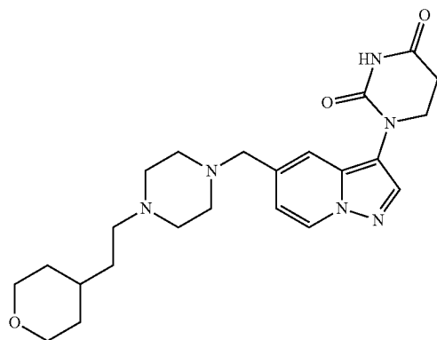
1-(5-((4-(2-(tetrahydro-2H-pyran-4-yl)ethyl)piperazin-1-yl)methyl)pyrazolo[1,5-a]pyridin-3-yl)dihydropyrimidine-2,4(1H,3H)-dione
