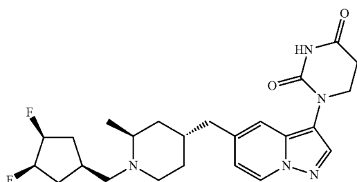
1-(5-(((2S,4R)-1-(((1R,3R,4S)-3,4-difluorocyclopentyl)methyl)-2-methylpiperidin-4-yl)methyl)pyrazolo[1,5-a]pyridin-3-yl)dihydropyrimidine-2,4-(1H,3H)-dione
