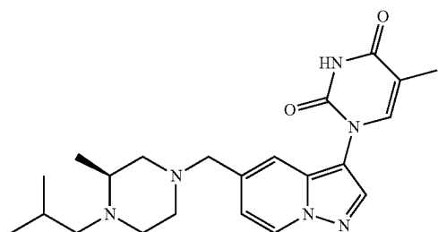
(S)-1-(5-((4-isobutyl-3-methylpiperazin-1-yl)methyl)pyrazolo[1,5-a]pyridin-3-yl)-5-methylpyrimidine-2,4(1H,3H)-dione
