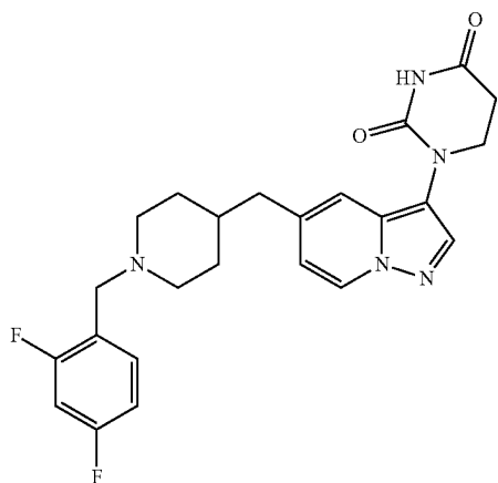
1-(5-((1-(2,4-difluorobenzyl)piperidin-4-yl)methyl)pyrazolo[1,5-a]pyridin-3-yl) dihydropyrimidine-2,4(1H,3H)-dione
