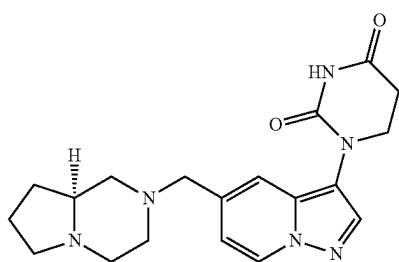
(S)-1-(5-((hexahydropyrrolo[1,2-a]pyrazin-2(1H)-yl)methyl)pyrazolo[1,5-a]pyridin-3-yl)dihydropyrimidine-2,4(1H,3H)-dione
