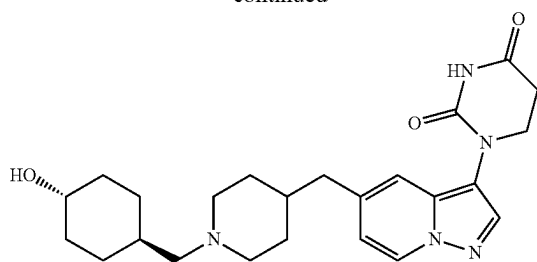
1-(5-(((1-(1r,4r)-4-hydroxycyclohexyl)methyl)piperidin-4-yl)methyl)pyrazolo[1,5-a]pyridin-3-yl)dihydropyrimidine-2,4(1H,3H)-dione
