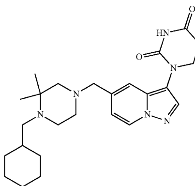
1-(5-((4-(cyclohexylmethyl)-3,3-dimethylpiperazin-1-yl)methyl)pyrazolo[1,5-a]pyridin-3-yl)dihydropyrimidine-2,4(1H,3H)-dione
