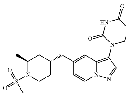
1-(5-(((2S,4R)-2-methyl-1-(methylsulfonyl)piperidin-4-yl)methyl)pyrazolo[1,5-a]pyridin-3-yl) dihydropyrimidine-2,4(1H,3H)-dione
