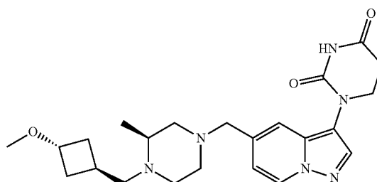
1-(5-(((S)-4-(((1R,3S)-3-methoxycyclobutyl)methyl)-3-methylpiperazin-1-yl)methyl)pyrazolo[1,5-a]pyridin-3-yl)dihydropyrimidine-2,4(1H,3H)-dione
