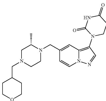
(S)-1-(5-((2-methyl-4-((tetrahydro-2H-pyran-4-yl)methyl)piperazin-1-yl)methyl)pyrazolo[1,5-a]pyridin-3-yl)dihydropyrimidine-2,4(1H,3H)-dione
