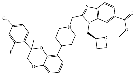
Methyl 2-((4-(3-(4-chloro-2-fluorophenyl)-3-methyl-2,3-dihydrobenzo[b][1,4]dioxan-5-yl)piperidin-1-yl)methyl)-1-(((S)-oxetan-2-yl)methyl)-1H-benzo[d]imidazole-6-carboxylate (a mixture of diastereomers)
