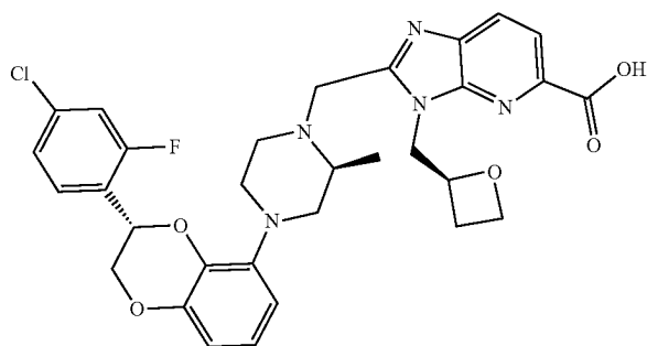
2-(((S)-4-((S)-3-(4-Chloro-2-fluorophenyl)-2,3-dihydrobenzo[b][1,4]dioxan-5-yl)-2-methylpiperazin-1-yl)methyl)-3-((S)-oxetan-2-ylmethyl)-3H-imidazo[4,5-b]pyridine-5-carboxylic acid 8
