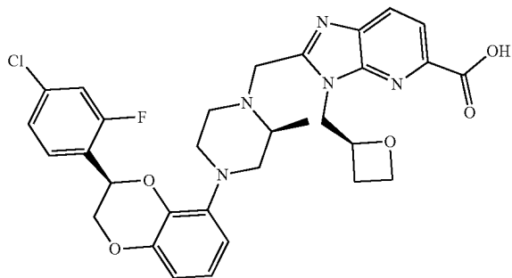
2-(((S)-4-((R)-3-(4-Chloro-2-fluorophenyl)-2,3-dihydrobenzo[b][1,4]dioxan-5-yl)-2-methylpiperazin-1-yl)methyl)-3-((S)-oxetan-2-ylmethyl)-3H-imidazo[4,5-b]pyridine-5-carboxylic acid
