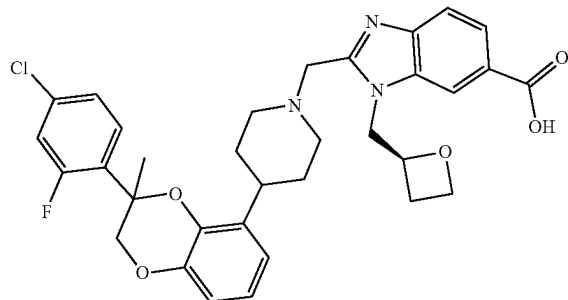
2-((4-(3-(4-Chloro-2-fluorophenyl)-3-methyl-2,3-dihydrobenzo[b][1,4]dioxan-5-yl)piperidin-1-yl)methyl)-1-(((S)-oxetan-2-yl)methyl)-1H-benzo[d]imidazole-6-carboxylic acid (a mixture of diastereomers) 20
