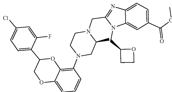
Methyl 2-(((2S)-4-(3-(4-chloro-2-fluorophenyl)-2-methylpiperazin-1-yl)methyl)-1-(((S)-oxetan-2-yl)methyl)-1H-benzo[d]imidazole-6-carboxylate (a mixture of diastereomers) 19c
