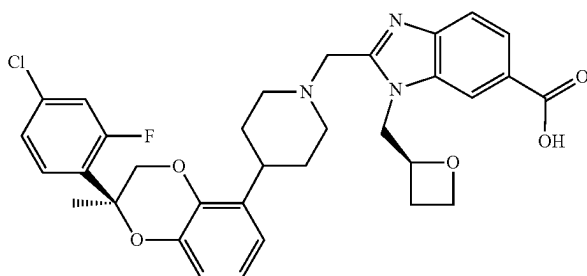
2-((4-((R)-2-(4-Chloro-2-fluorophenyl)-2-methyl-2,3-dihydrobenzo[b][1,4]dioxan-5-yl)piperidin-1-yl)methyl)-1-(((S)-oxetan-2-yl)methyl)-1H-benzo[d]imidazole-6-carboxylic acid
