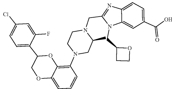
2-(((2S)-4-(3-(4-Chloro-2-fluorophenyl)-2-methylpiperazin-1-yl)methyl)-1-(((S)-oxetan-2-yl)methyl)-1H-benzo[d]imidazole-6-carboxylic acid (a mixture of diastereomers) 19
