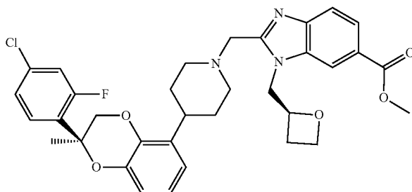
Methyl 2-((4-((R)-2-(4-chloro-2-fluorophenyl)-2-methyl-2,3-dihydrobenzo[b][1,4]dioxan-5-yl)piperidin-1-yl)methyl)-1-(((S)-oxetan-2-yl)methyl)-1H-benzo[d]imidazole-6-carboxylate
