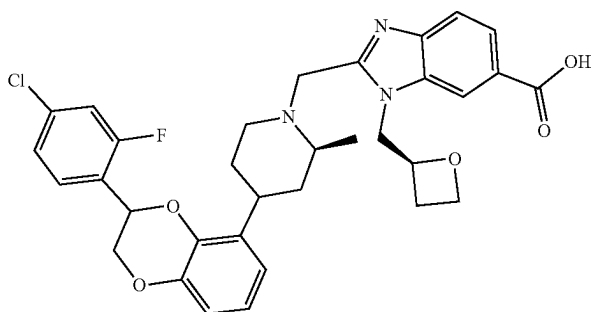
2-(((S)-4-(3-(4-Chloro-2-fluorophenyl)-2,3-dihydrobenzo[b][1,4]dioxan-5-yl)-2-methylpiperidin-1-yl)methyl)-1-(((S)-oxetan-2-yl)methyl)-1H-benzo[d]imidazole-6-carboxylic acid (a mixture of diastereomers)
