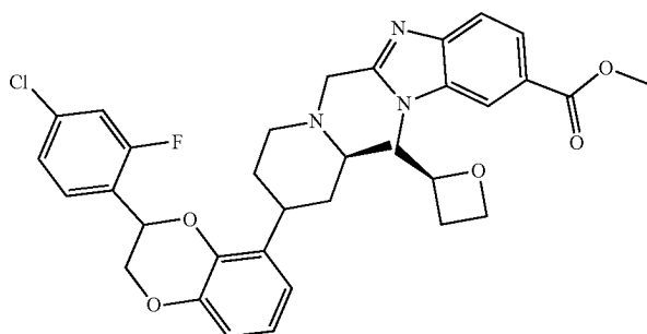
Methyl 2-(((2S)-4-(3-(4-chloro-2-fluorophenyl)-2,3-dihydrobenzo[b][1,4]dioxan-5-yl)-2-methylpiperidin-1-yl)methyl)-1-(((S)-oxetan-2-yl)methyl)-1H-benzo[d]imidazole-6-carboxylate (a mixture of diastereomers)
