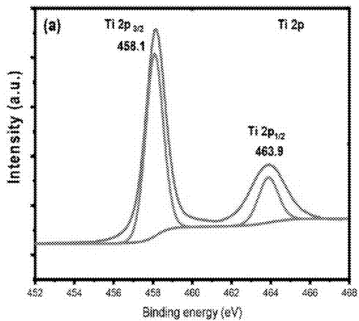
Fig. 8A - XPS spectra of Ti 2p
