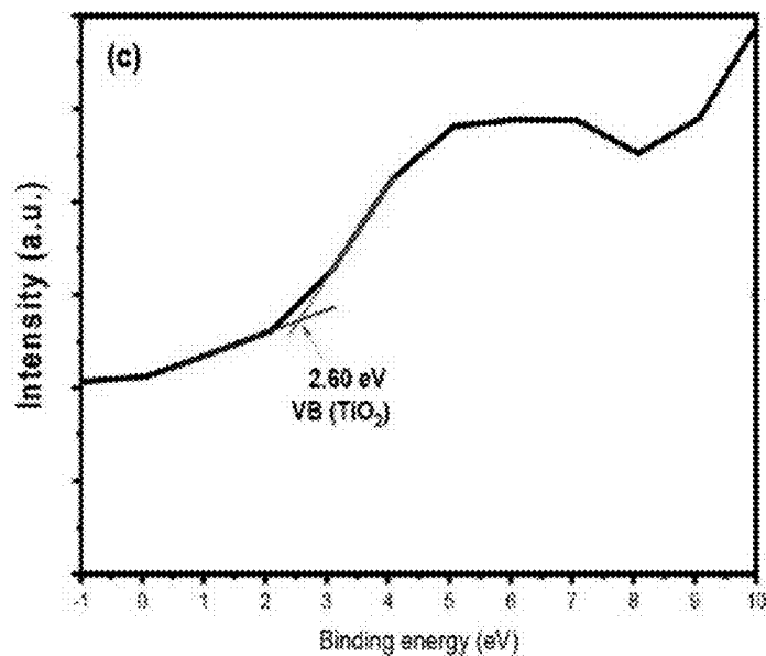
Fig. 8C - Wide spectra for TiO 2 VB calculation
