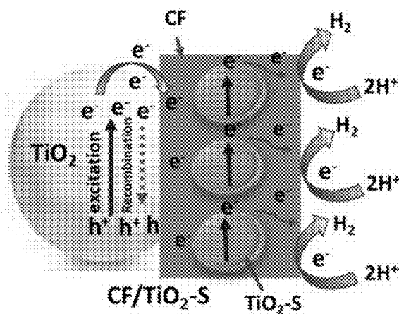
Fig. 12D - Schematic illustration of charge transfer over \text{CFs/TiO}_2\text{-S} produced using sol-gel approach
