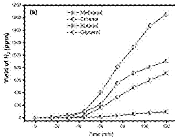
Fig. 13 - Effect of sacrificial reagents on the performance of the 3CFs/TiO 2 -S composite catalyst
