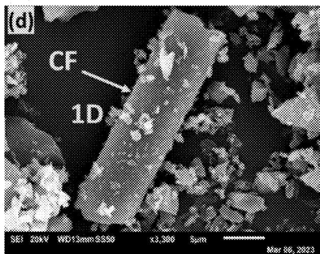
Fig. 7D - SEM images of CFs
