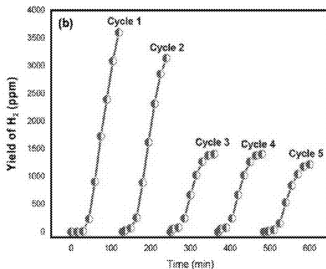
Fig. 15B - Photostability of 3CFs/TiO 2 -S with 5% methanol for continuous H 2 evolution for consecutive 5 cycles with 150 mg catalyst loading
