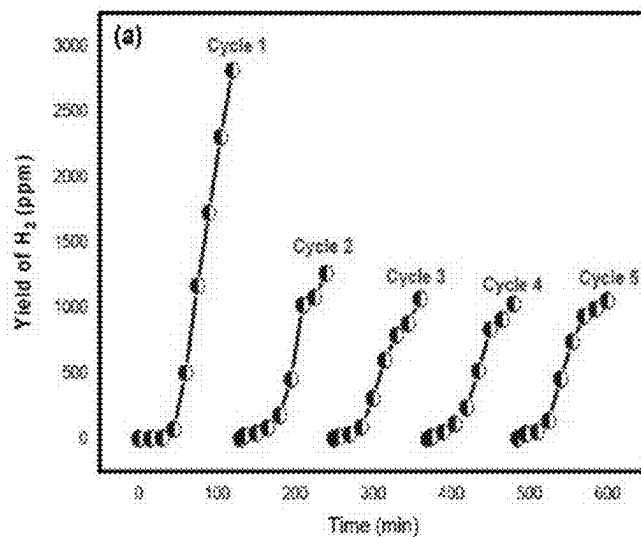
Fig. 15A - Photostability of 3CFs/TiO 2 -S with 5% glycerol for continuous H 2 evolution for 5 consecutive cycles with 150 mg catalyst loading
