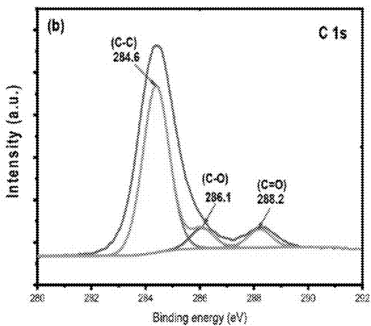
Fig. 8B - XPS spectra of C 1s
