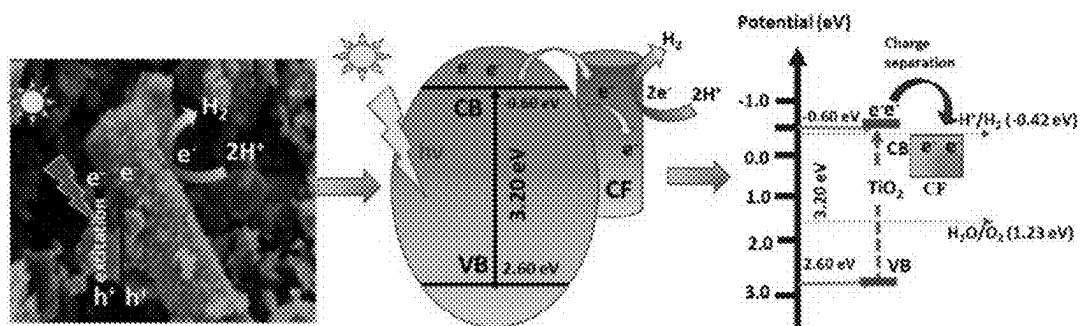
Fig. 19 - Proposed mechanism for photocatalytic H 2 evolution over a 3CFs/TiO 2 -S composite photocatalyst
