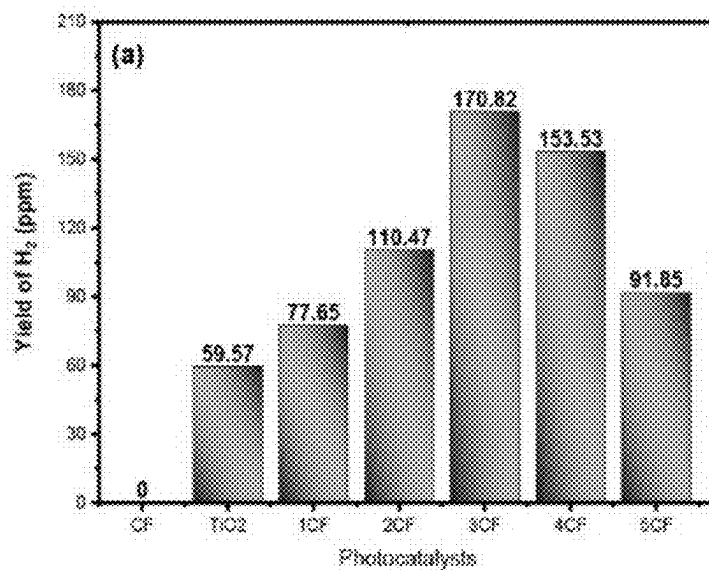
Fig. 12A - Effect of CF-loading on the performance of TiO 2 -A for photocatalytic H 2 evolution in a 5 vol % methanol solution and 100 mg catalyst loading
