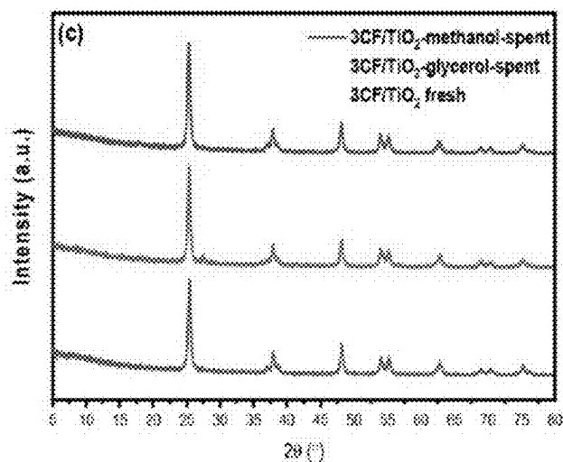
Fig. 16 - XRD analysis of the fresh and the spent catalyst
