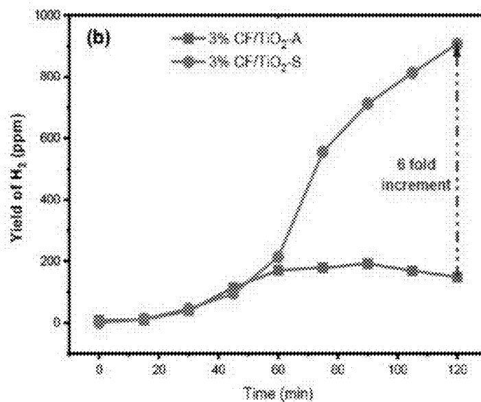
Fig. 12B - Performance comparison of 3CF/TiO 2 -A and 3CF/TiO 2 -S synthesized through sol-gel method for photocatalytic H 2 evolution with 5 vol % methanol and 100 mg catalyst loading
