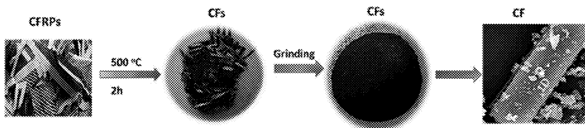
Schematic illustration for the preparation of CFs from CFRPs through thermal decomposition
