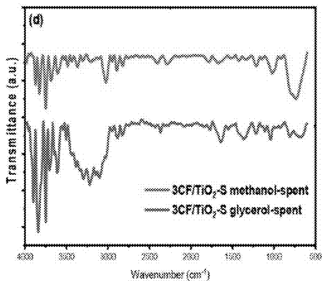
Fig. 17 - FTIR analysis of 3% CFs/TiO 2 -S composite after the reaction of methanol and glycerol
