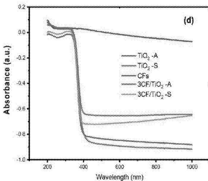
Fig. 9 - UV-vis diffuse reflectance spectra of TiO 2 , CFs, and their composites
