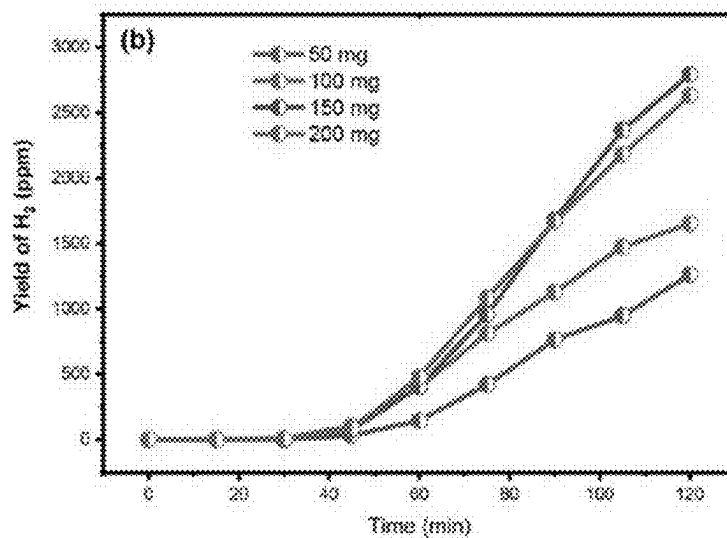
Fig. 14 - Effect of CFs loading on the performance of 3CFs/TiO 2 -S for photocatalytic H 2 evolution using a glycerol sacrificial reagent
