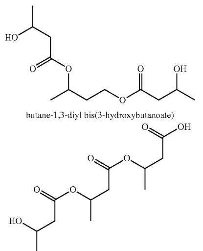
3-((3-((3-hydroxybutanoyl)oxy)butanoyl)oxy)butanoic acid
