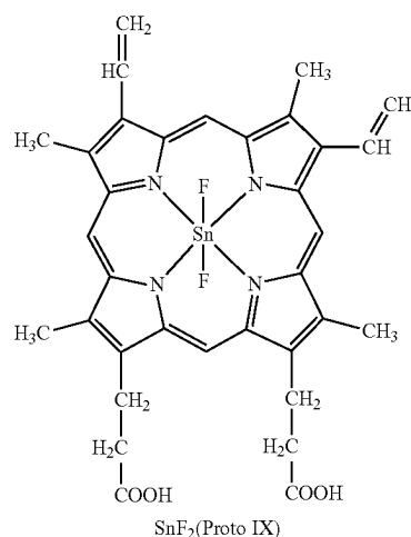
[Chemical Formulae 4]
