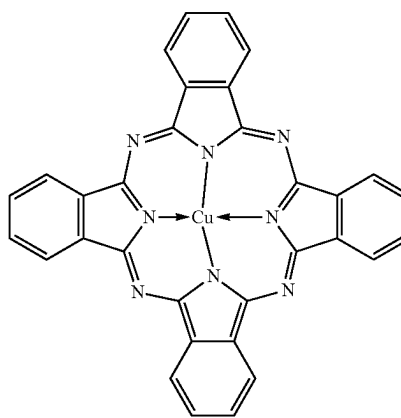
CuPc
