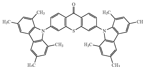
[Chemical Formula 6]
