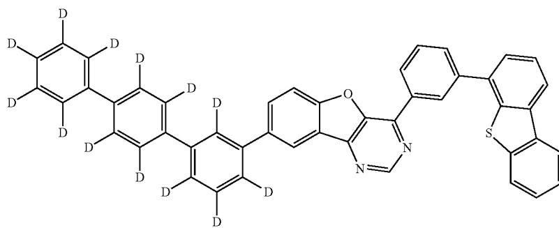
8mpTP-4mDBtPBfpm-d 13
