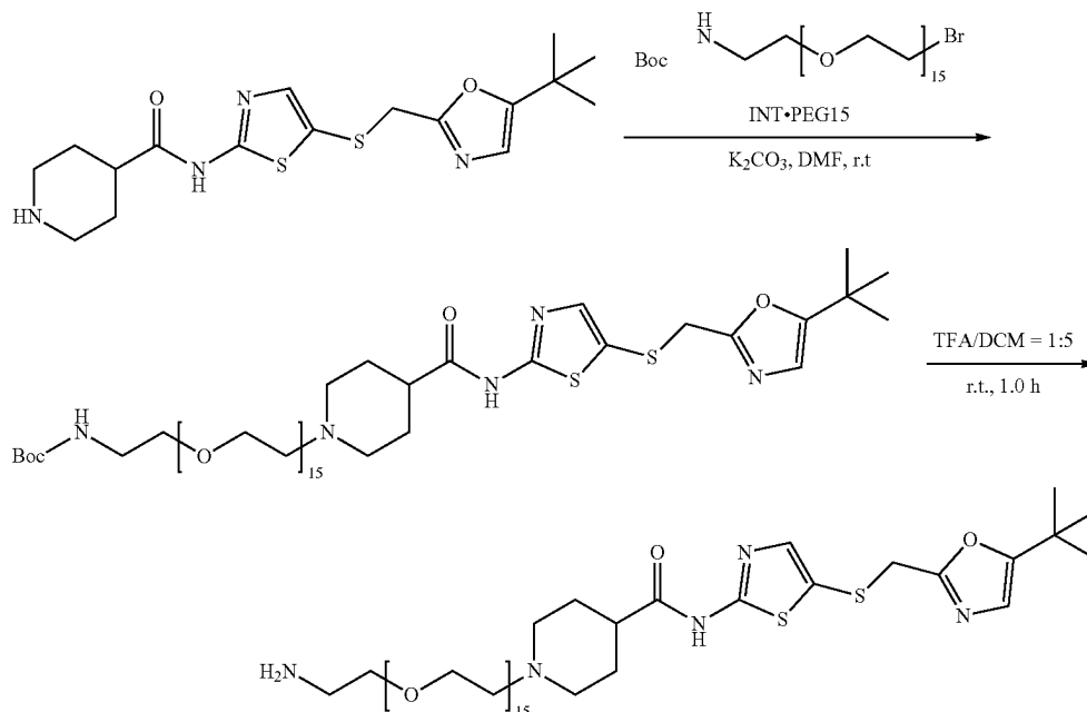
Scheme D. Example for Amine Formation Reaction (N-alkylation reaction)
