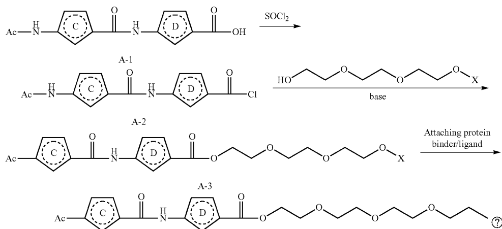
Scheme A: Synthesis of first terminus/second terminus/linker conjugate.
