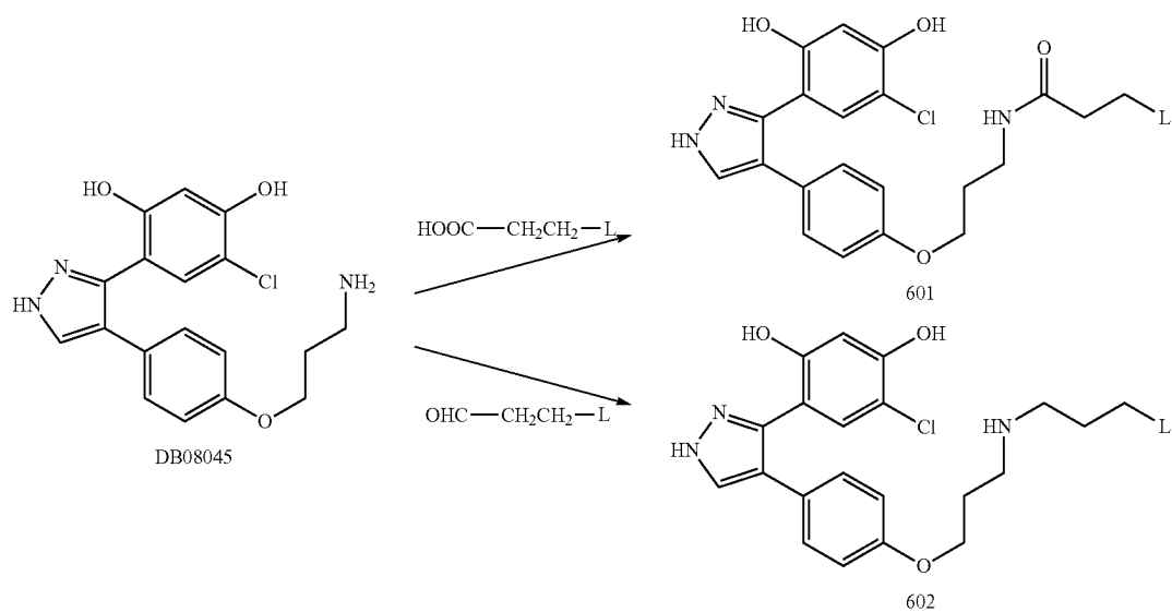
Scheme VI: Proposed synthesis of DB08045-based cyclin T1 inhibitor
