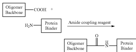
Scheme VIII. Amide Couplings
