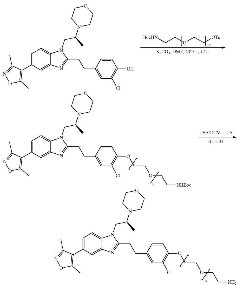
Scheme C. Example for Ether Formation Reaction (O-alkylation reaction)
