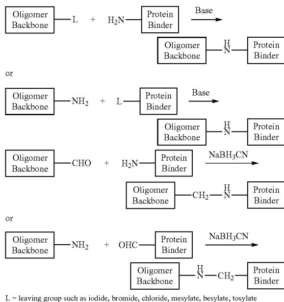
Scheme X. Amine Formation Reactions (N-alkylation reactions)
