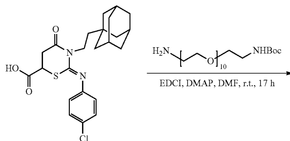
Scheme B. Example for Amide Coupling
