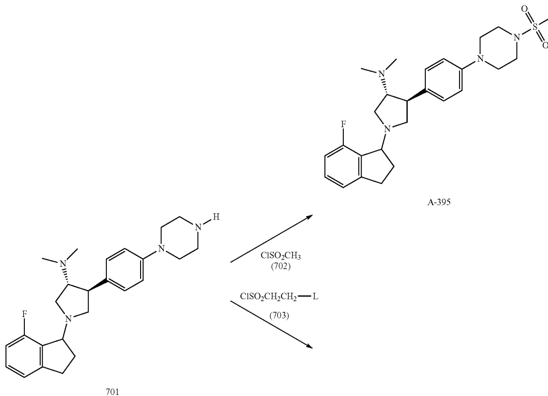
Scheme VII: Proposed synthesis of A-395 based PRC2 inhibitor
