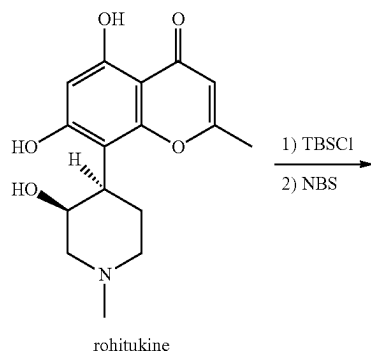
Scheme V: Proposed synthesis of rohitukine-based CDK9 inhibitor
