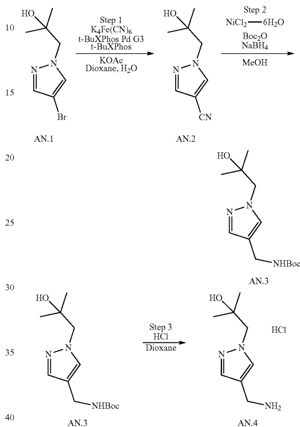
Scheme AN
