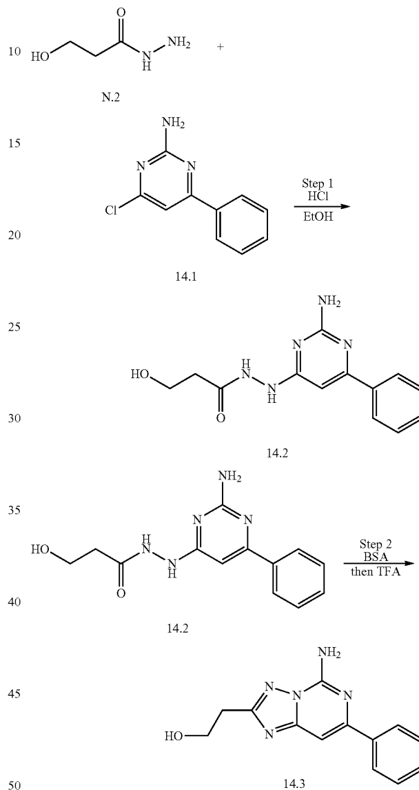
Scheme 14
