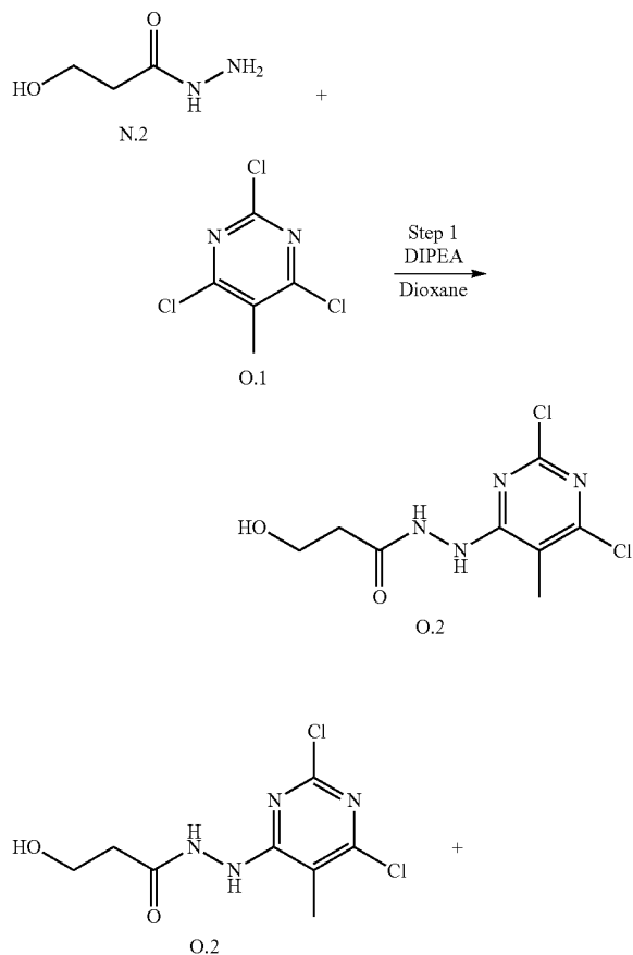
Scheme O
