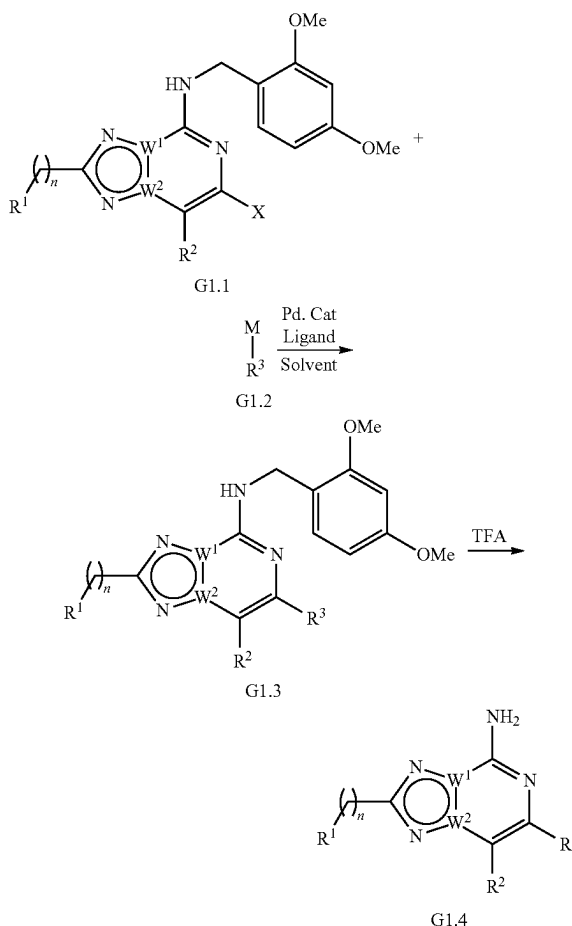
General Scheme 1
