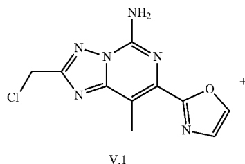
Scheme 11
