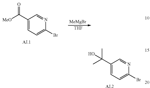
Scheme AJ
