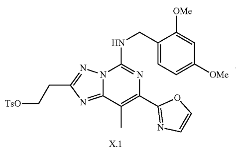
Scheme 17
