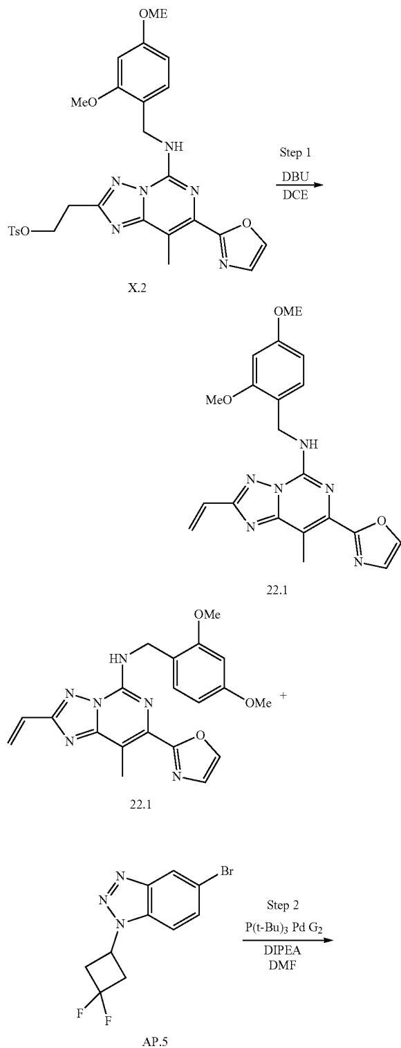
Scheme 22
