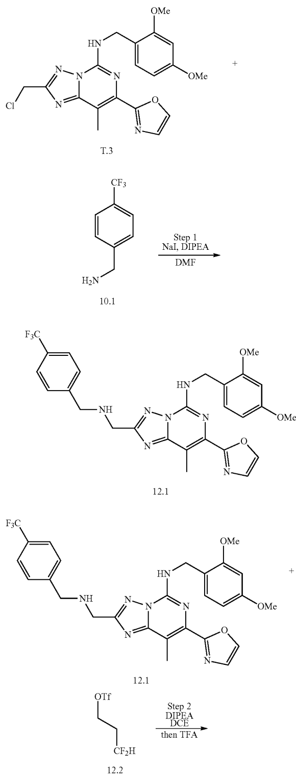
Scheme 12
