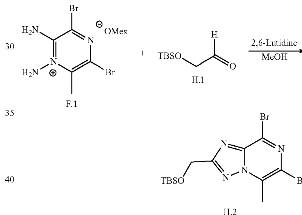
Scheme H
