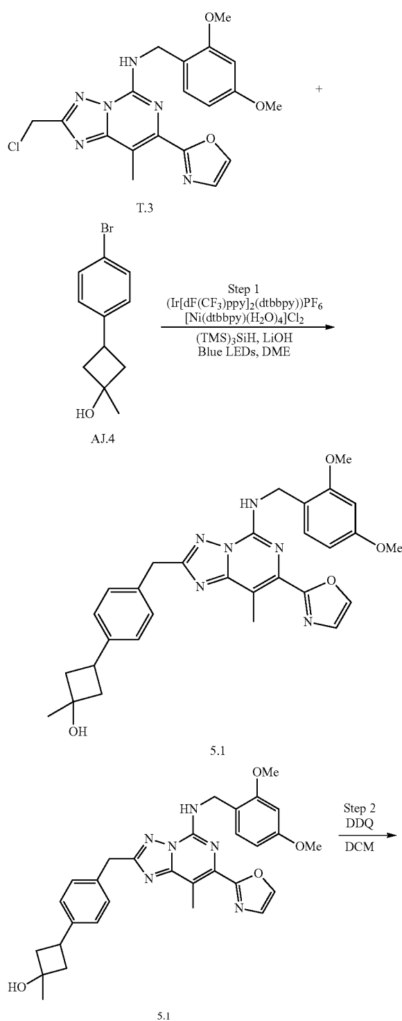
Scheme 5
