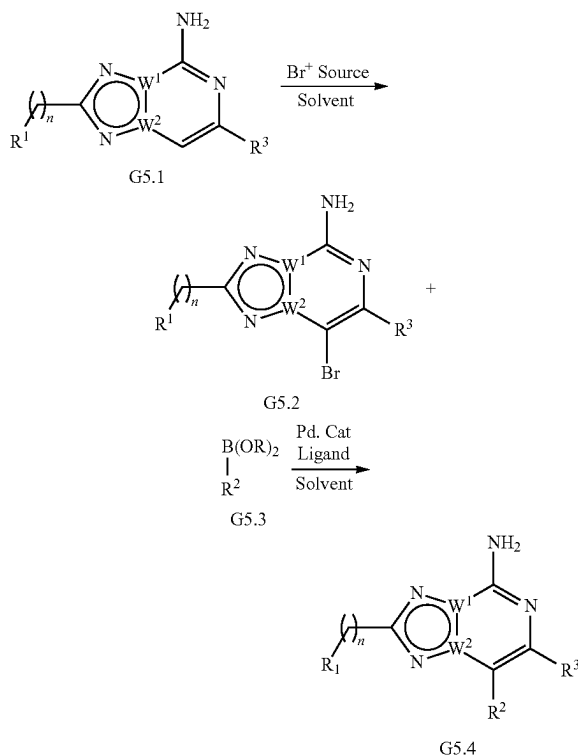
General Scheme 5
