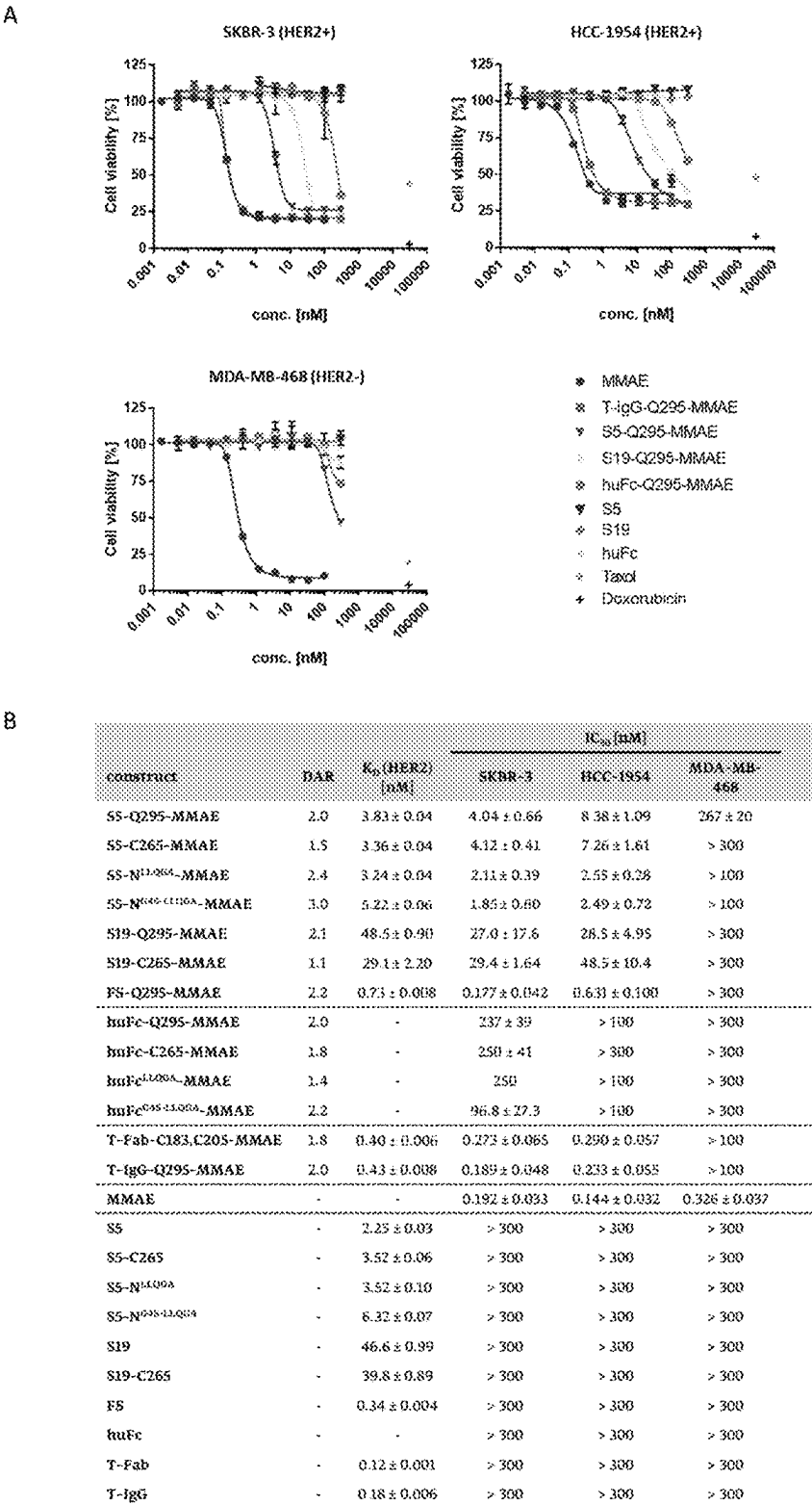
Fig. 25 - In vitro cytotoxicity data
