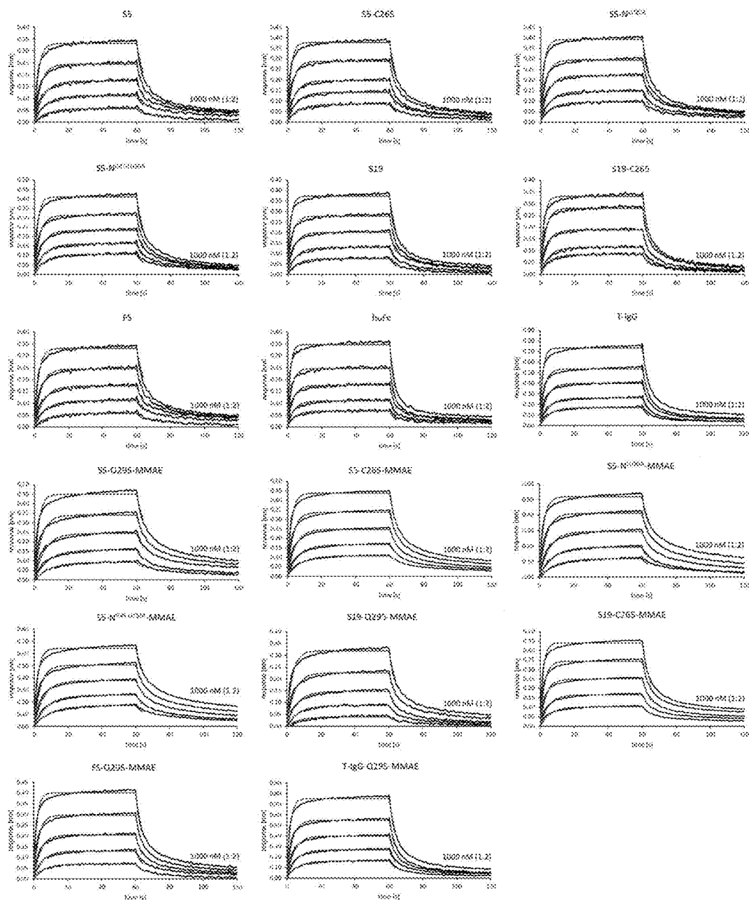
Fig. 23 - FcRn binding analysis of unconjugated Fcabs, Trastuzumab variants and respective MMAE conjugates via BLI
