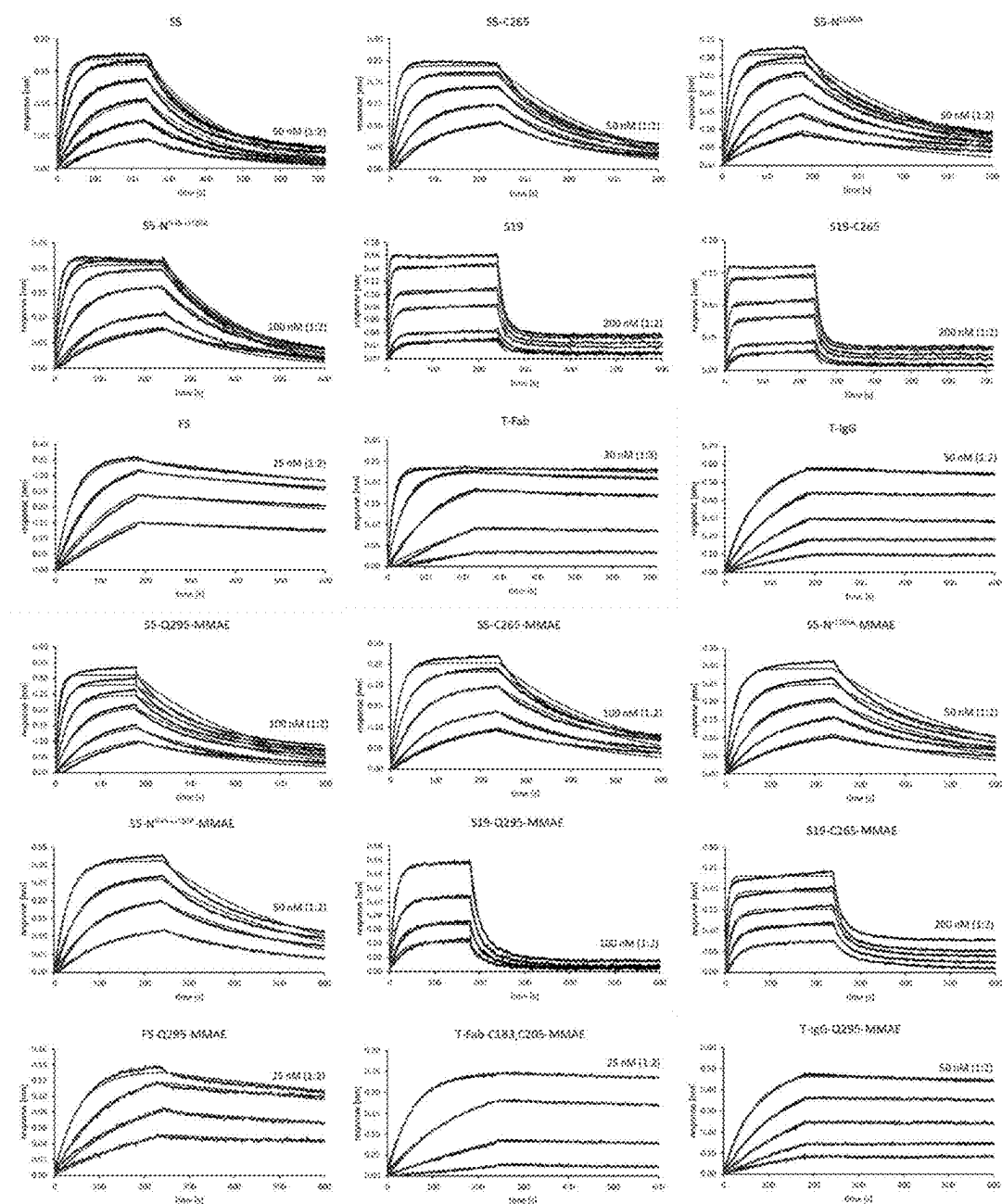
Fig. 22 - HER2 binding analysis of unconjugated Fcabs, Trastuzumab variants and respective MMAE conjugates via BLI
