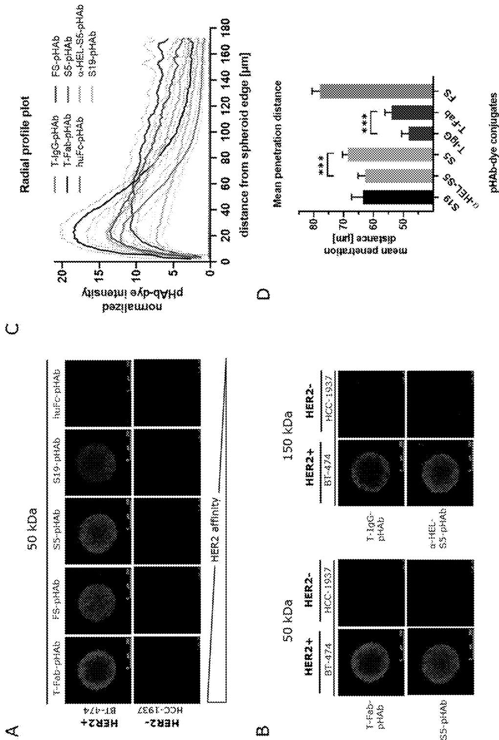
Fig. 5 - 3D tumor spheroid penetration model
