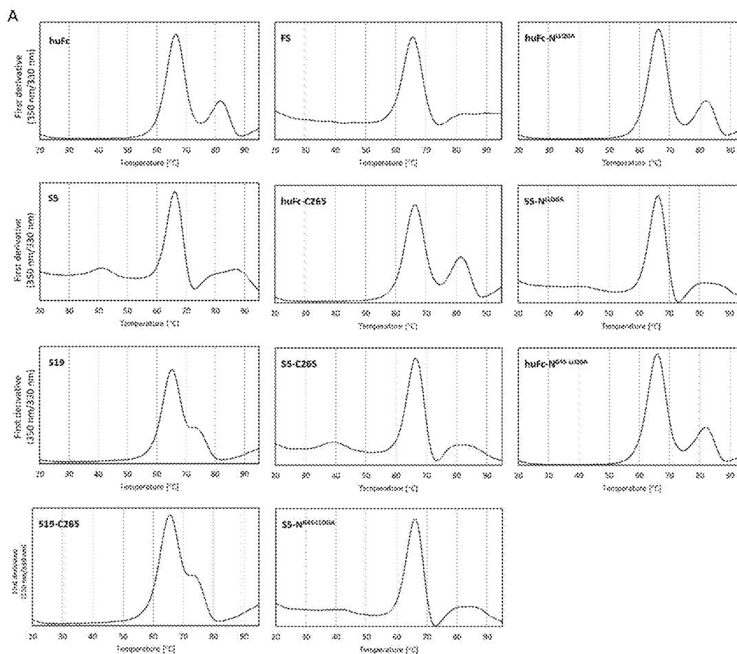
Fig. 11 - Thermal stability of Fcabs and huFc control molecules
