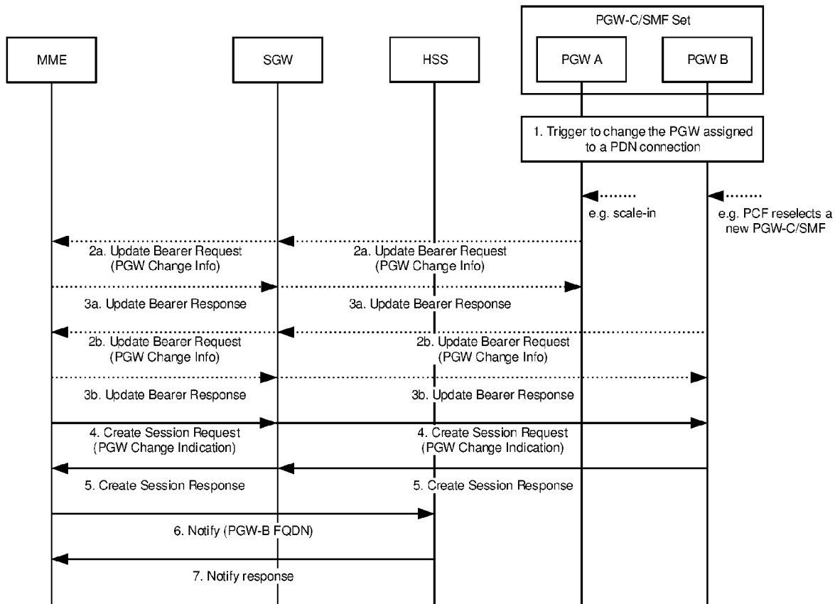
Figure 31.4-1: PGW triggered PDN connection restoration
