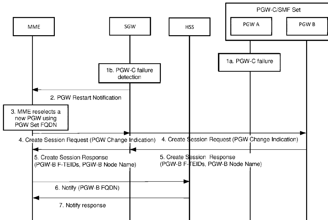
Figure 31.3-1: MME triggered PDN connection restoration
