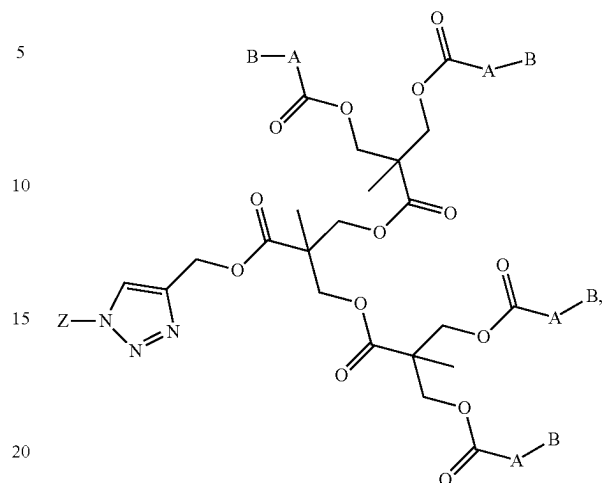
Formula Ie
