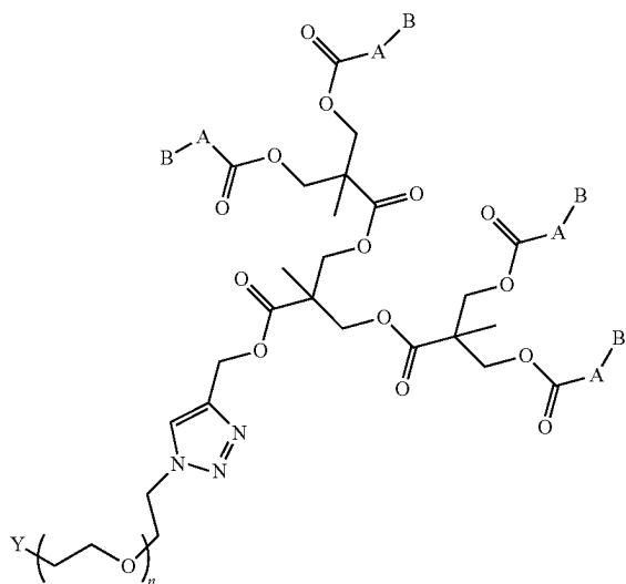
Formula If
