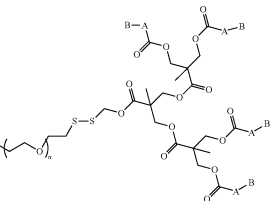
Formula Iia
