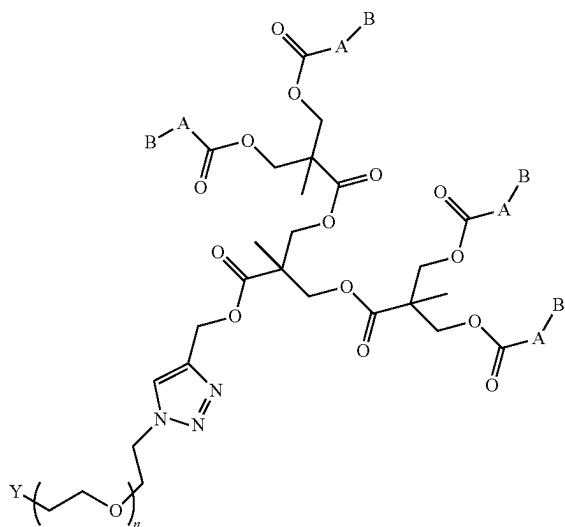
Formula Id
