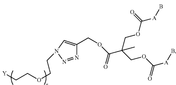
Formula Id
