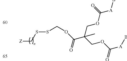
Formula Ig
