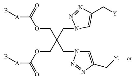
Formula Ig
