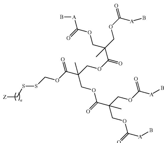
Formula Ii
