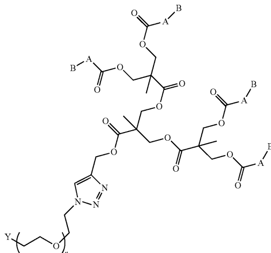
Formula If
