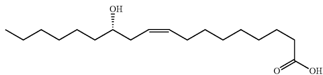
Ricinoleic Acid
