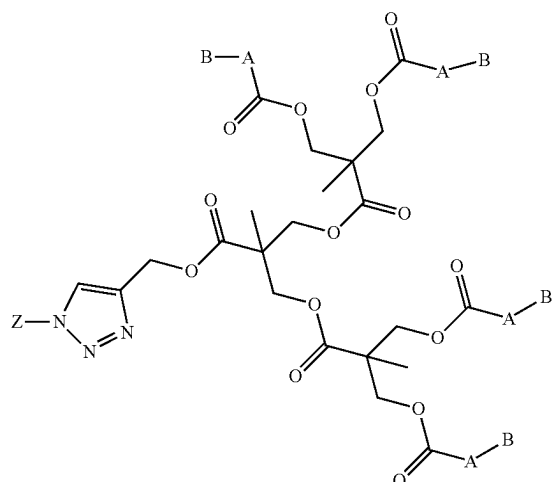
Formula Id
