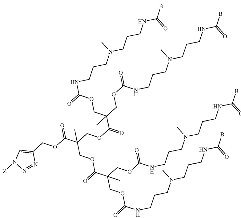
Compound 7
