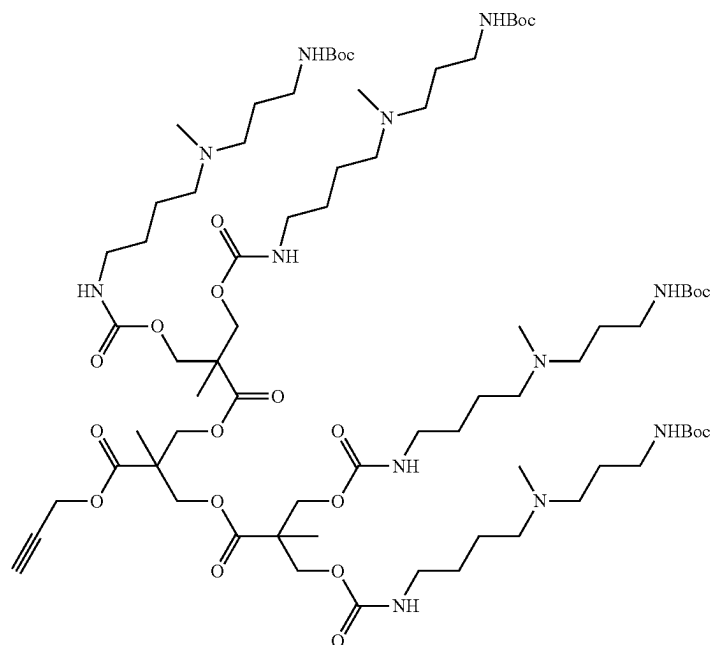
Compound 11 Chemical Formula: C 74 H 136 N 12 O 22 Molecular Weight: 1545.96
