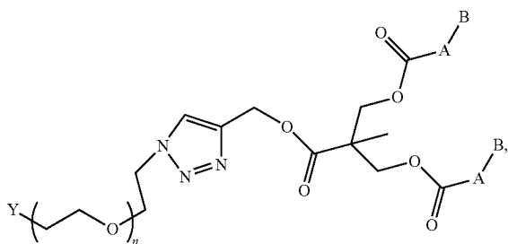
Formula If
