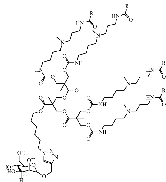
Compound 10
