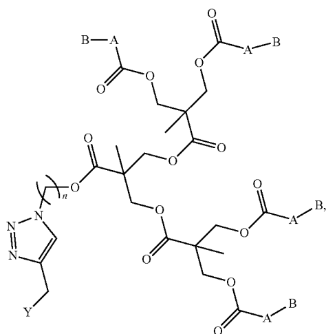
Formula Ib
