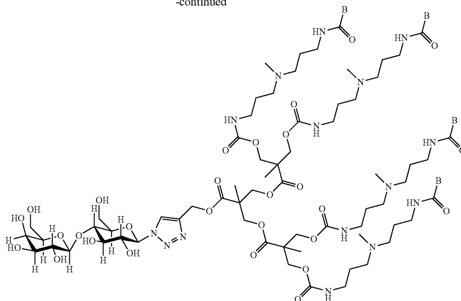
Compound 5
