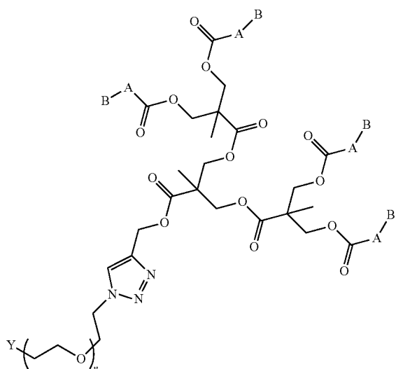
Formula Ig
