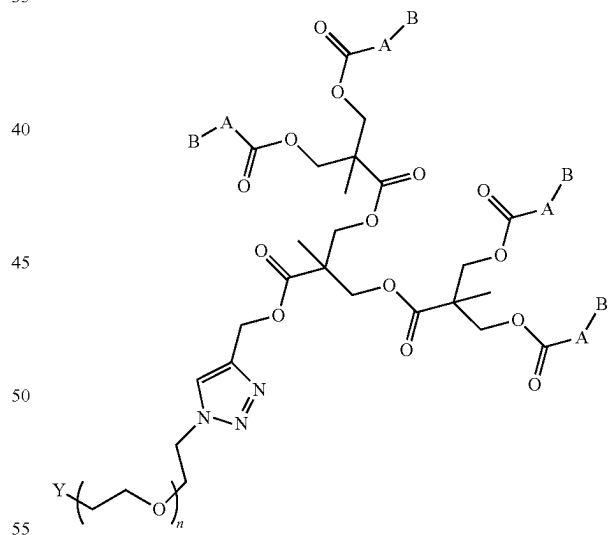
Formula Ig
