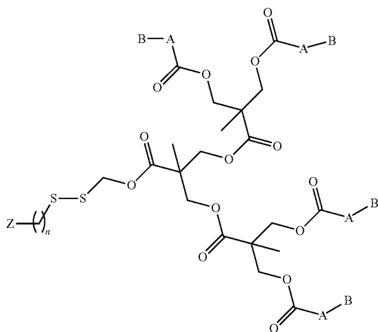
Formula Ih
