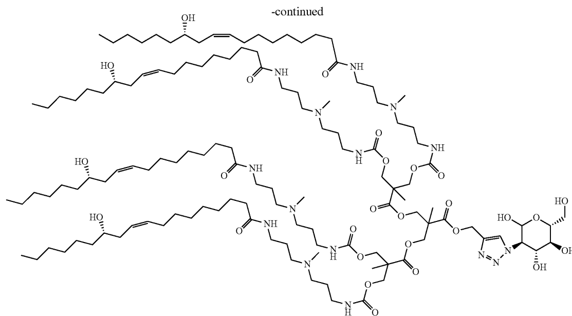
Compound 3
