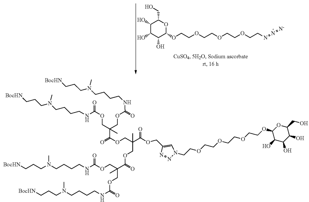
Compound 12 Chemical Formula: C 88 H 163 N 15 O 31 Molecular Weight: 1926.16
