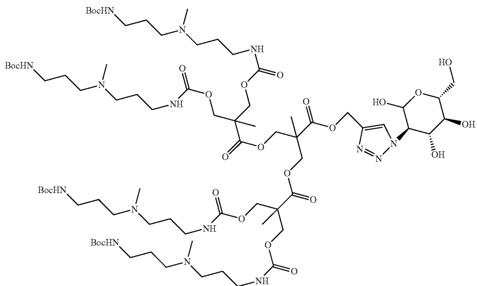
Compound 2
