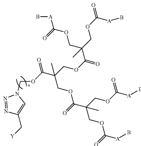
Formula Ib
