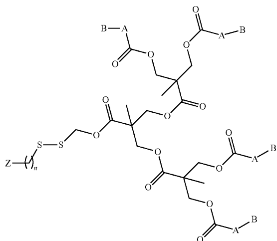
Formula Ii
