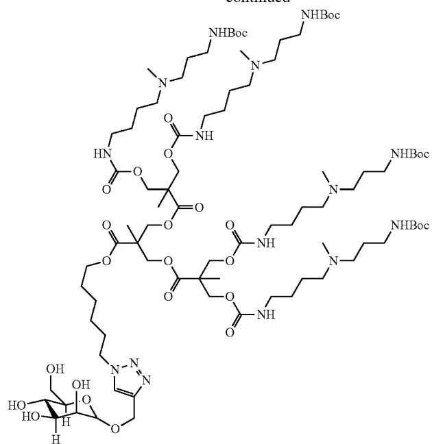
Compound 9
