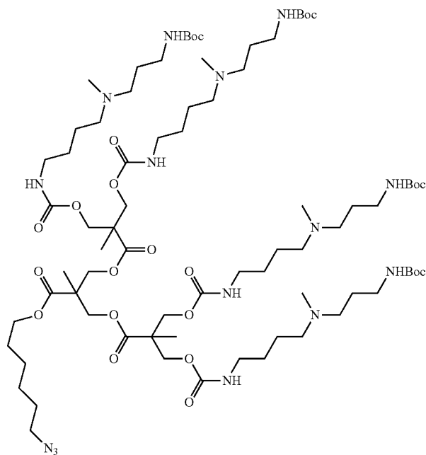
Compound 8
