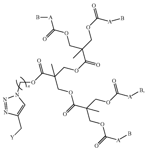
Formula Ib
