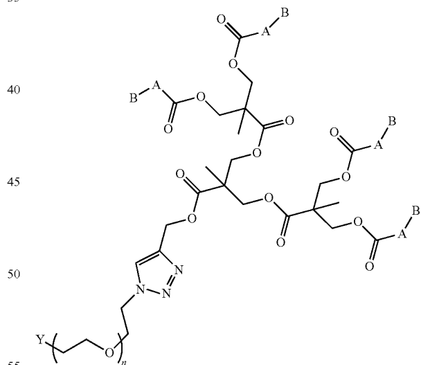
Formula Ig
