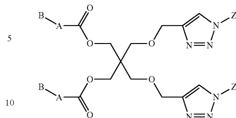
Formula Ih
