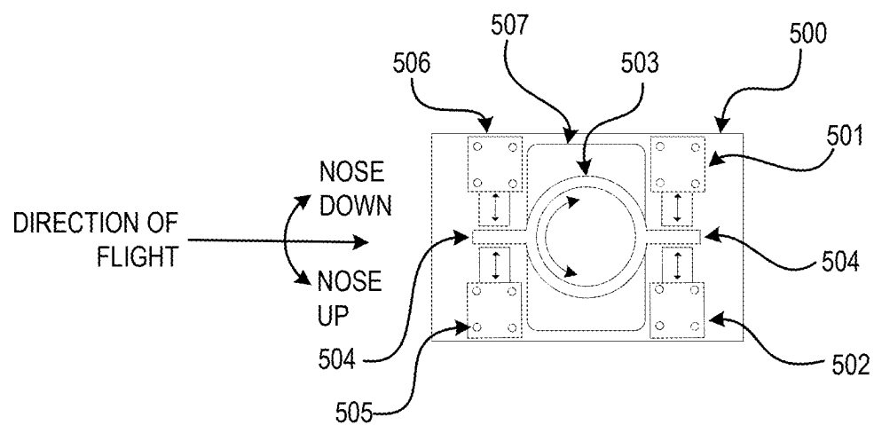
FIGURE 5A - SIDE VIEW
