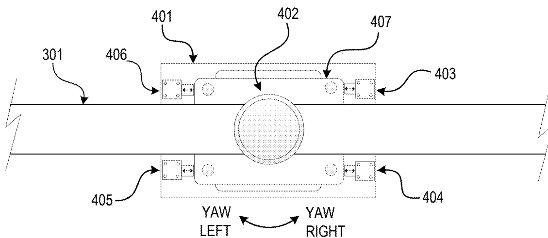
FIGURE 4A – TOP VIEW
