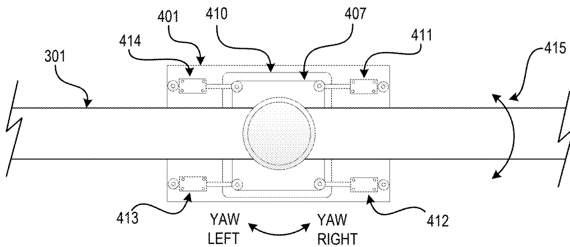
FIGURE 4D – TOP VIEW
