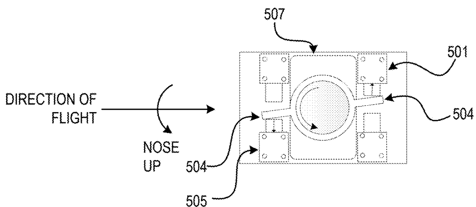
FIGURE 5B - SIDE VIEW
