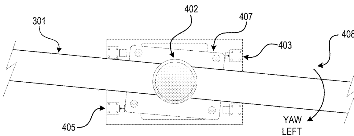
FIGURE 4B – TOP VIEW
