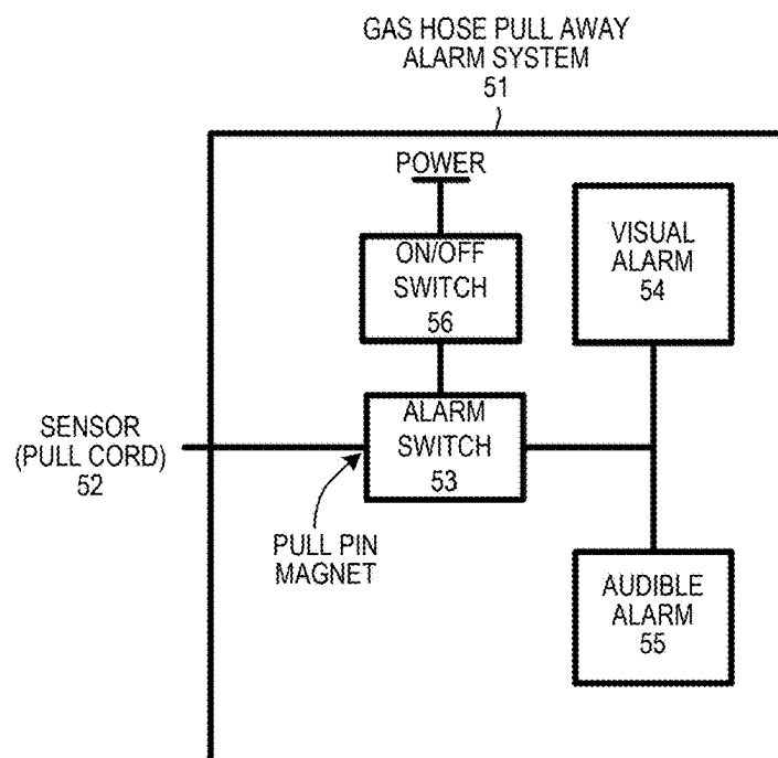
ANALOG CIRCUIT CONTROLLED GAS HOSE PULL AWAY ALARM SYSTEM
