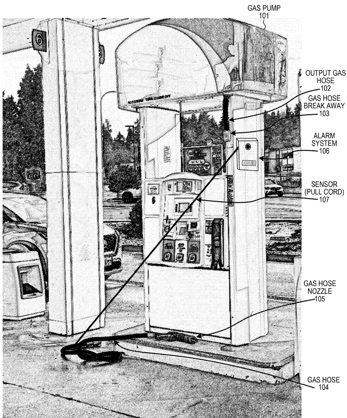
GAS STATION PUMP WITH GAS HOSE PULL AWAY ALARM SYSTEM (ALARM ENGAGED AFTER GAS HOSE PULL AWAY)
