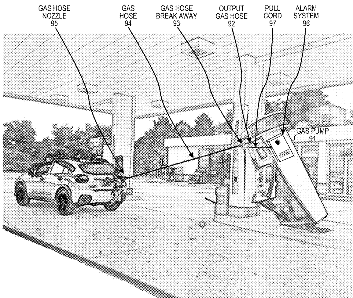
GAS STATION PUMP WITH GAS HOSE PULL AWAY ALARM SYSTEM (ALARM ENGAGED AFTER GAS HOSE PULL AWAY)
