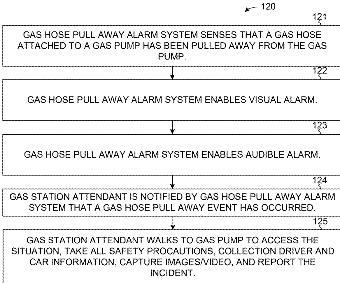
GAS HOSE PULL AWAY ALARM SYSTEM OPERATIONAL FLOWCHART
