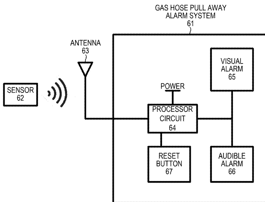
DIGITAL AND WIRELESS CIRCUIT CONTROLLED GAS HOSE PULL AWAY ALARM SYSTEM
