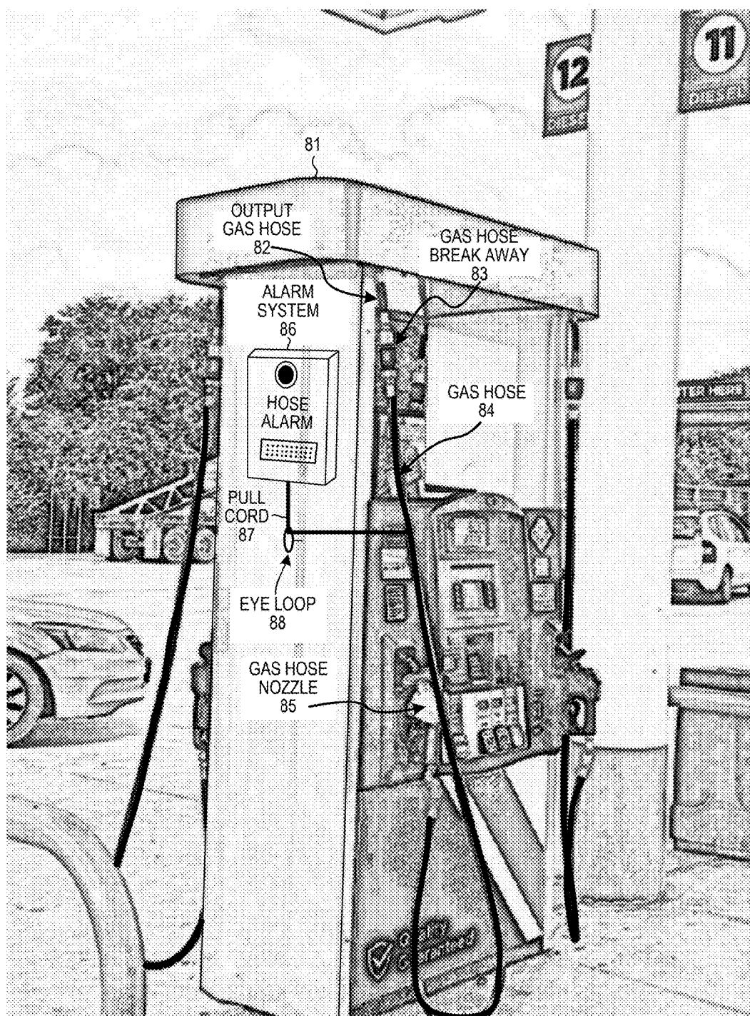
GAS STATION PUMP WITH GAS HOSE PULL AWAY ALARM SYSTEM (ALARM NOT ENGAGED)
