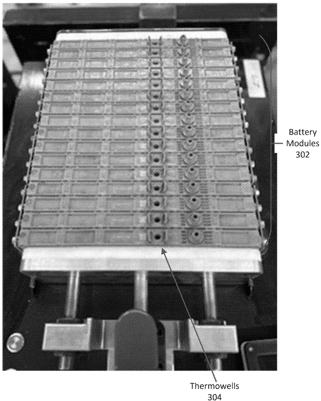
Battery Pack 300
