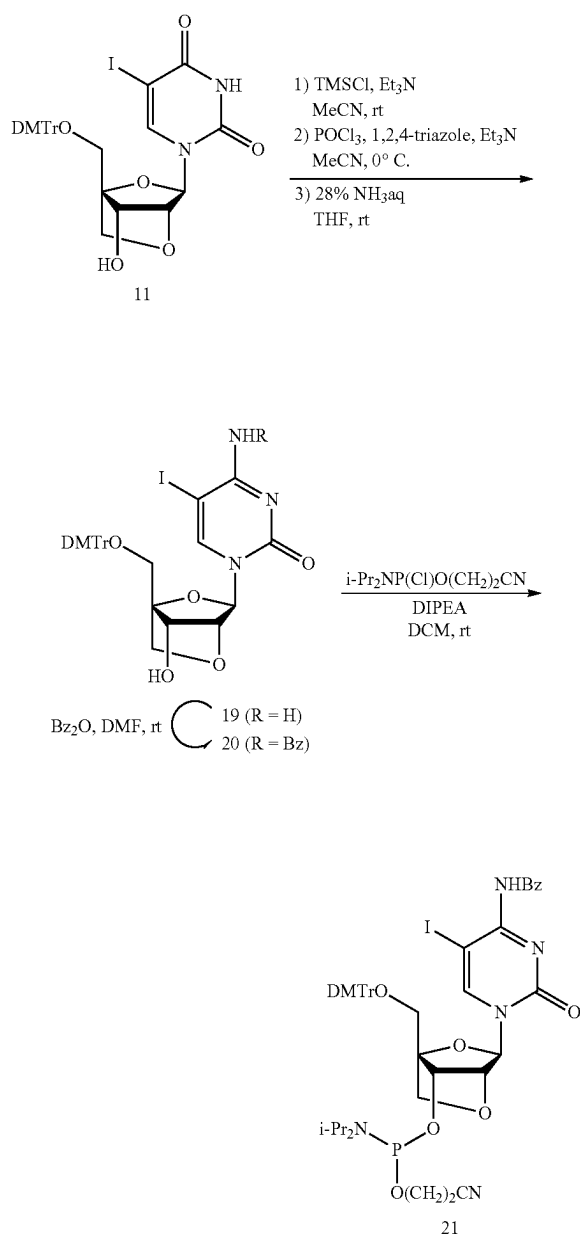
Scheme 21. Synthesis of LNA-5-iodocytidine phosphoramidite (21)
