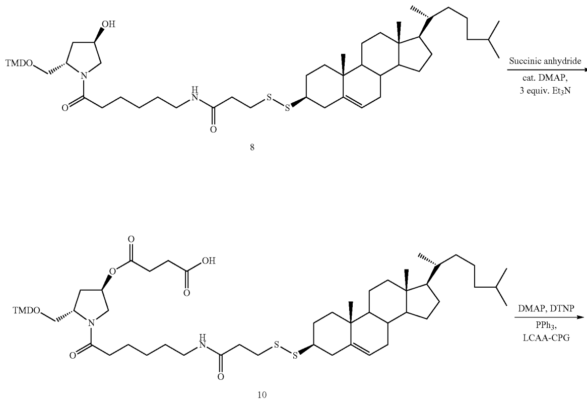
Scheme 14. Synthesis of polymer support immobilized with thiocholesterol
