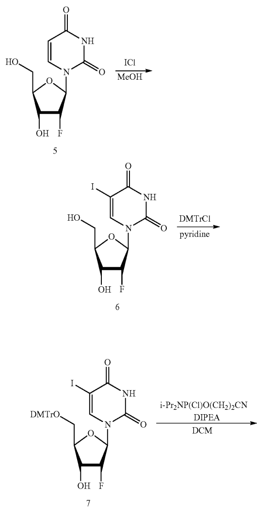
Scheme 17. Synthesis of 2'-deoxy-2'-(R)-fluoro-5-iodouridine phosphoramidite (8)
