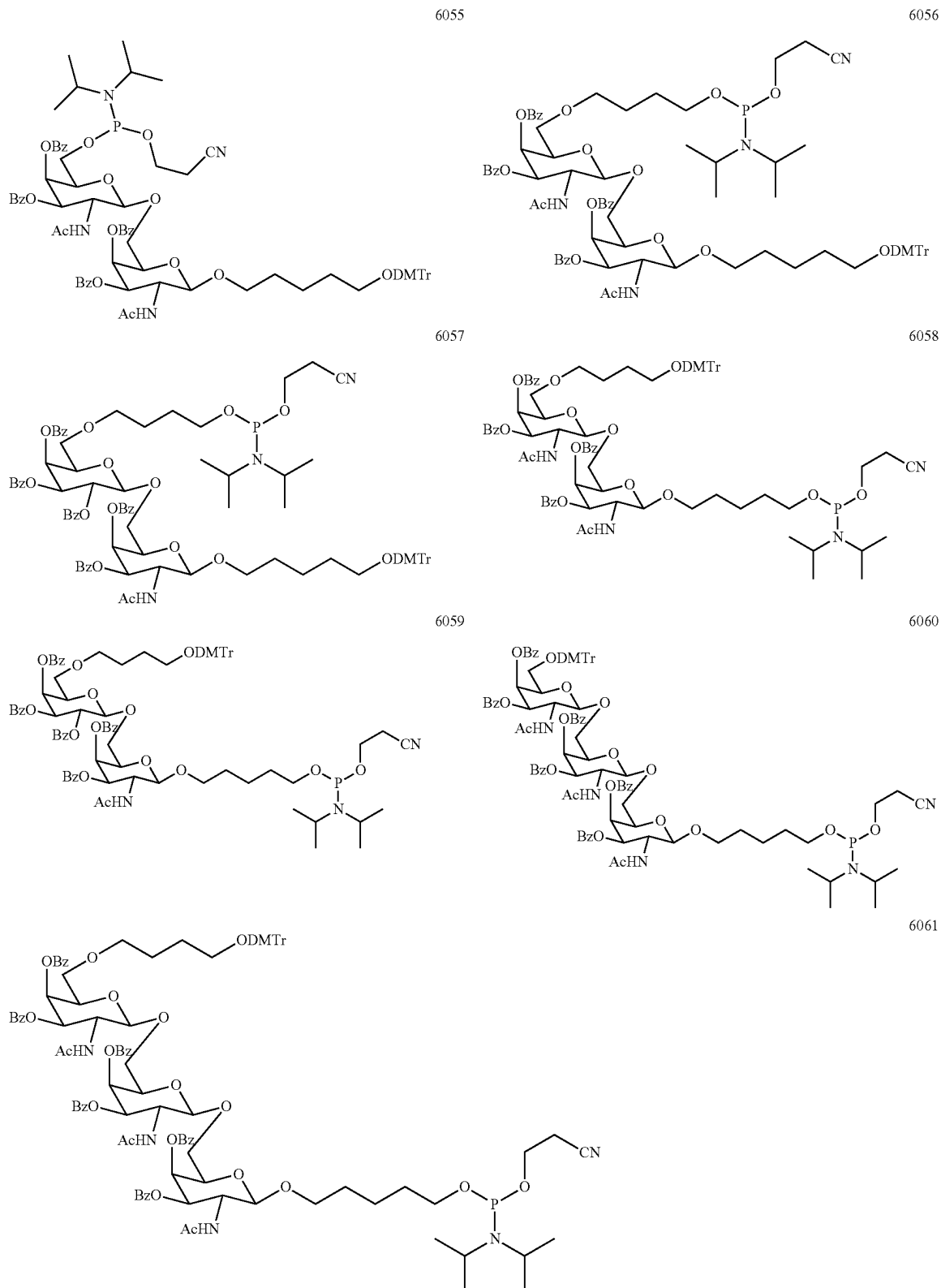
Scheme 29. Various modified carbohydrates (di or tri sacchaides of galactose, galactosamine, glucose, glucosamine, mannose, mannoseamine derivatives)
