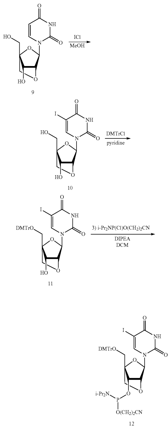
Scheme 18. Synthesis of LNA-5-iodouridine phosphoramidite 12
