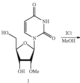
Scheme 16. Synthesis of 2'-O-methyl-5-iodouridine phosphoramidite (4)
