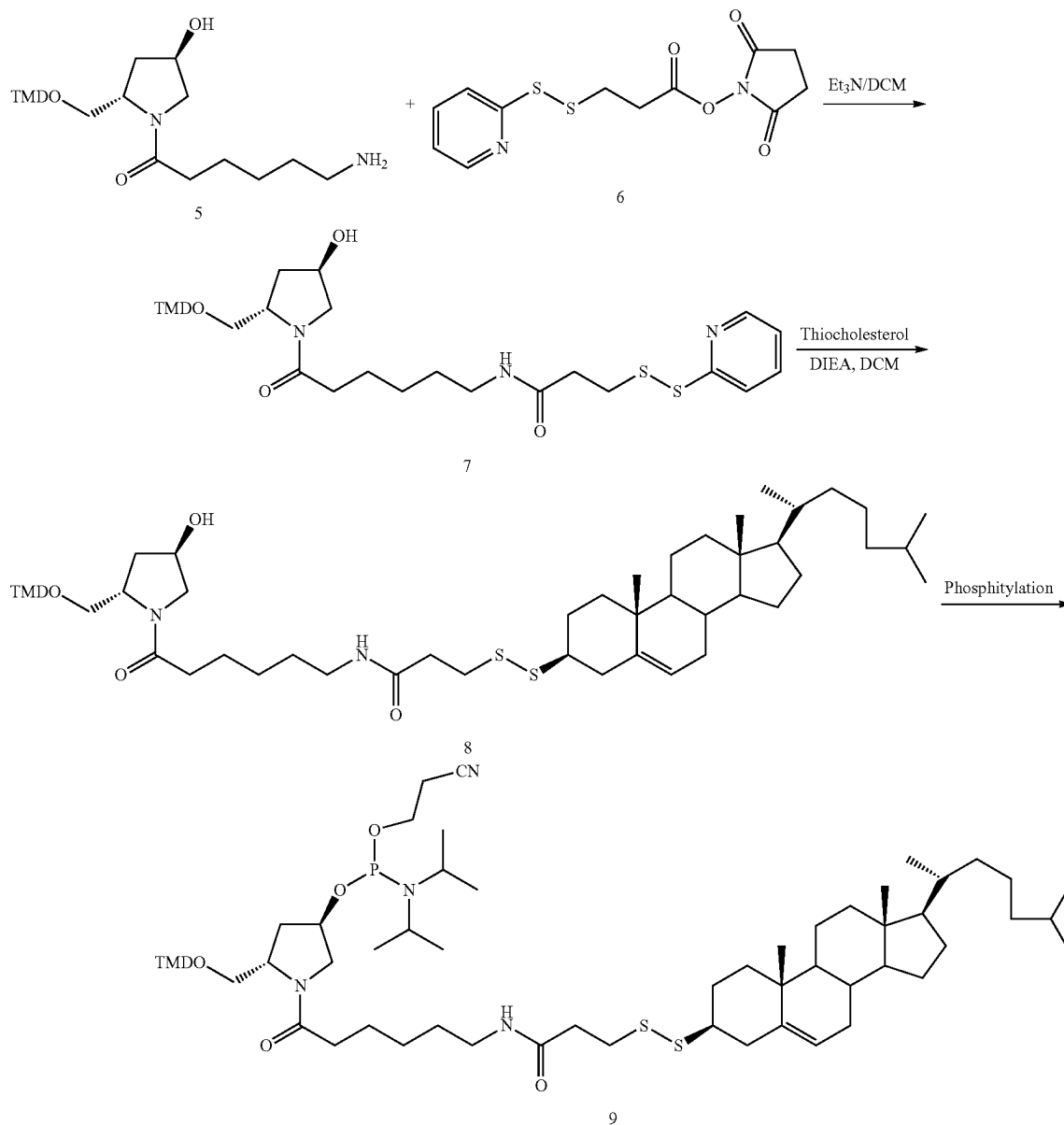
Scheme 13. Synthesis of 4-hydroxy-L-prolinol-thiocholesterol phosphoramidite
