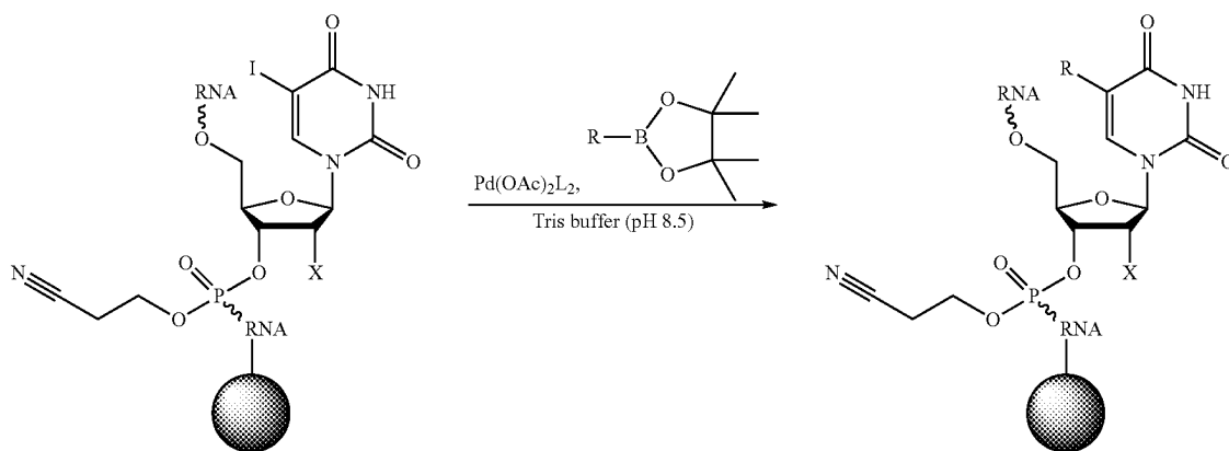
Scheme 27. Conjugation on CPG
