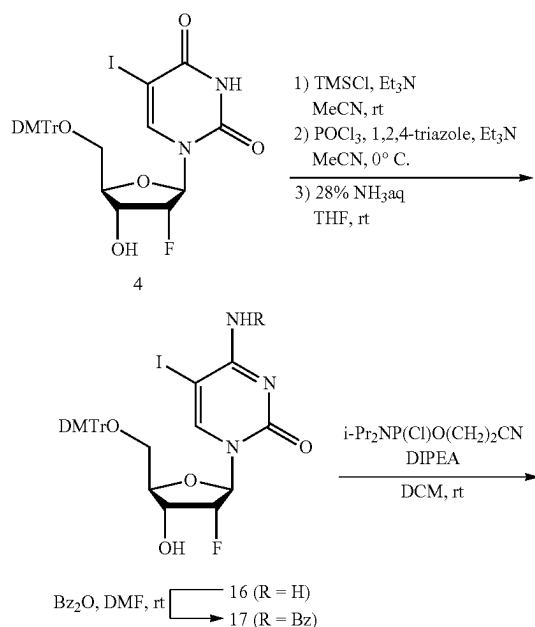
Scheme 20. Synthesis of 2'-deoxy-2'-(R)-fluoro-5-iodocytidine phosphoramidite (18)
