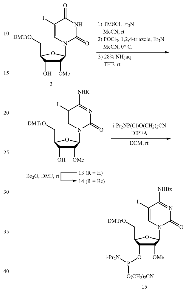
Scheme 19. Synthesis of 2'-O-methyl-5-iodocytidine phosphoramidite (15)
