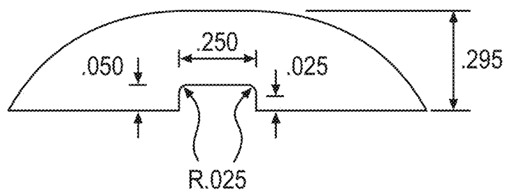
5-WIRE OPENING
