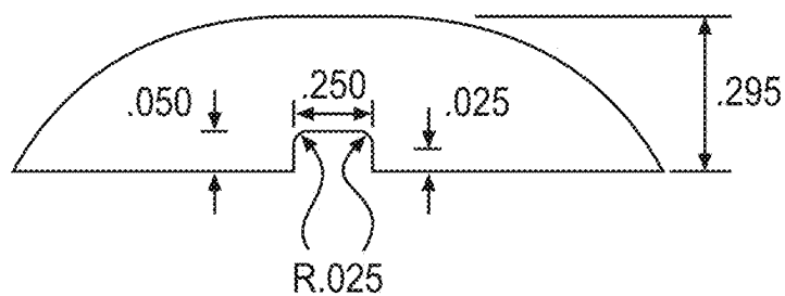
3-WIRE OPENING
