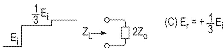
(C) Line Terminated in Z_L = 2Z_0
