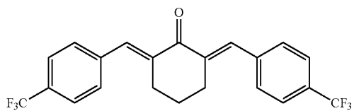
Compound S18
