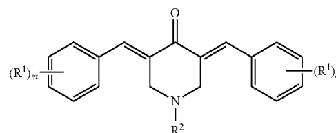
Structure I-A1
