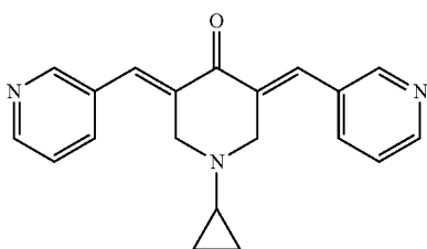
(3E,5E)-1-cyclopropyl-3,5-bis(pyridin-3-ylmethylene)piperidin-4-one (9-8)
