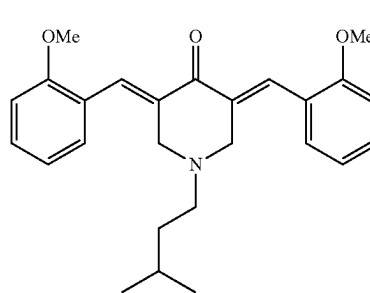
(3E,5E)-1-isopentyl-3,5-bis(2-methoxybenzylidene)piperidin-4-one (10-1)
