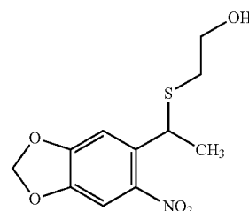
Chemical Formula: C 11 H 13 NO 5 S Exact Mass: 271.05144 Molecular Weight: 271.28700
