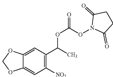
Chemical Formula: C 14 H 12 N 2 O 9 Exact Mass: 352.05428 Molecular Weight: 352.25500
