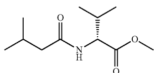
(R)-methyl 3-methyl-2-(3-methylbutanamido)butanoate (8a)
