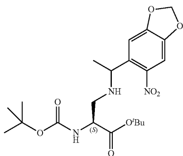
Chemical Formula: C 21 H 31 N 3 O 8 Exact Mass: 453.2111 Molecular Weight: 453.49200
