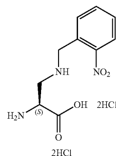
Chemical Formula: C 10 H 13 N 3 O 4 •2HCl Exact Mass: 239.09061 Molecular Weight: 312.14700 (as 2HCl salt)
