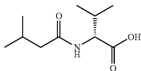
(R)-3-methyl-2-(3-methylbutanamido)butanoic acid (8b)
