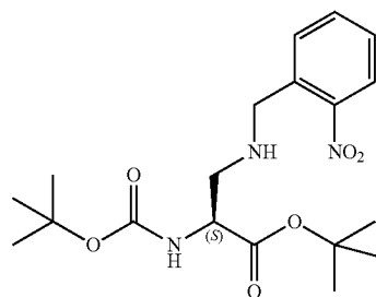
Chemical Formula: C 19 H 29 N 3 O 6 Exact Mass: 395.20564 Molecular Weight: 395.45600
