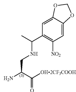
2TFA (mixture of ~1:1 epimers) Chemical Formula: C 21 H 15 N 3 O 6 •2CF 3 COOH Exact Mass: 297.09609 Molecular Weight: 525.31342 (as disalt of CF 3 COOH)
