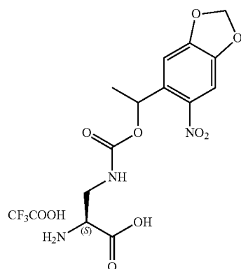
TFA (mixture of ~1:1 epimers) Chemical Formula: C 13 H 15 N 3 O 8 •CF 3 COOH Exact Mass: 341.08591 Molecular Weight: 455.29921 (with TFA)
