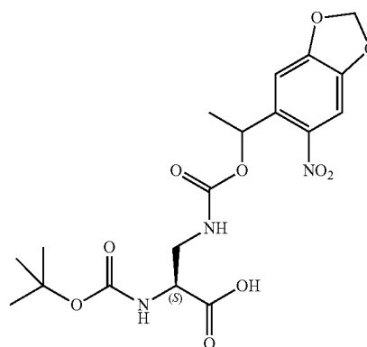
Chemical Formula: C 18 H 23 N 3 O 10 Exact Mass: 441.13834 Molecular Weight: 441.39300
