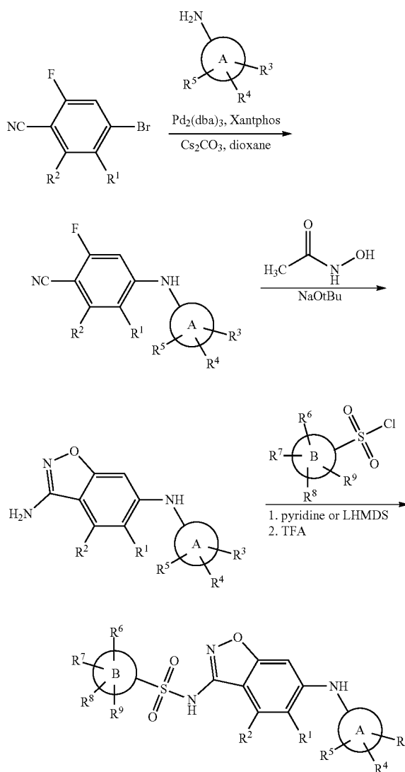
Scheme IV
